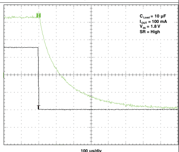
Figure 17. t_{OFF} Response
