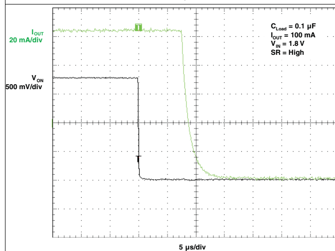
Figure 16. t_{OFF} Response
