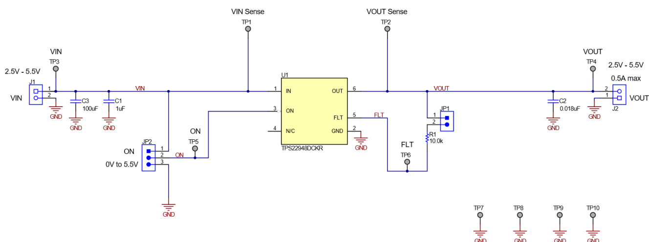
Figure 1. TPS22948EVM Schematic
