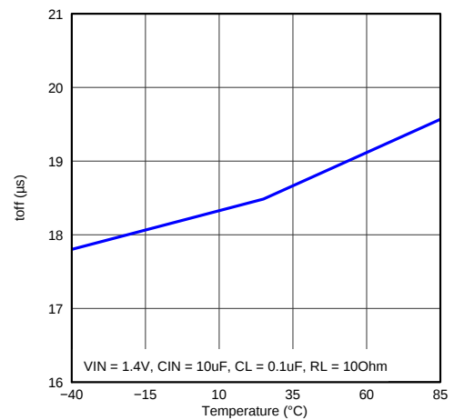
Figure 16. t_{OFF} vs Temperature (VIN = 1.4 V)
