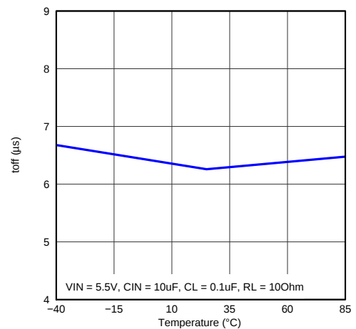
Figure 14. t_{OFF} vs Temperature (VIN = 5.5 V)
