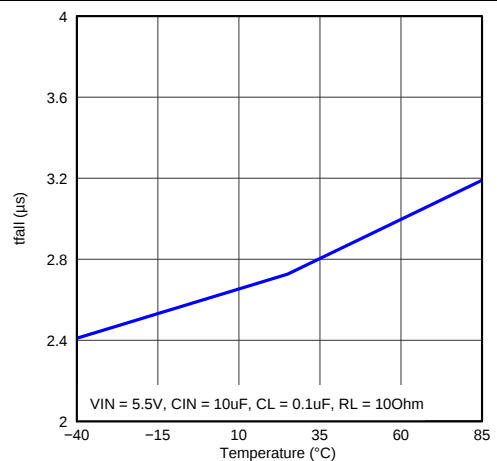
Figure 10. t_F vs Temperature ( V_{IN} = 5.5\text{V} )
