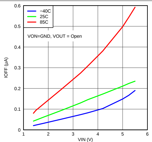
Figure 6. I_{IN(off)} vs V_{IN}
