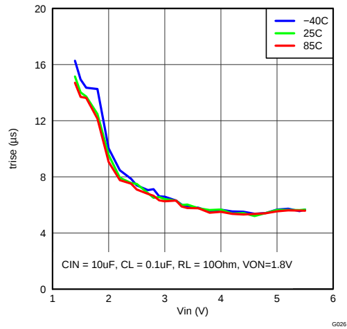
Figure 17. t_R vs V_{IN}
