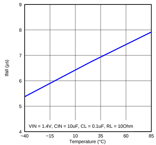
Figure 12. t_F vs Temperature (VIN = 1.4 V)
