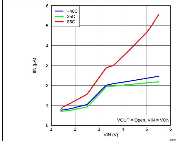
Figure 3. I IN vs V IN
