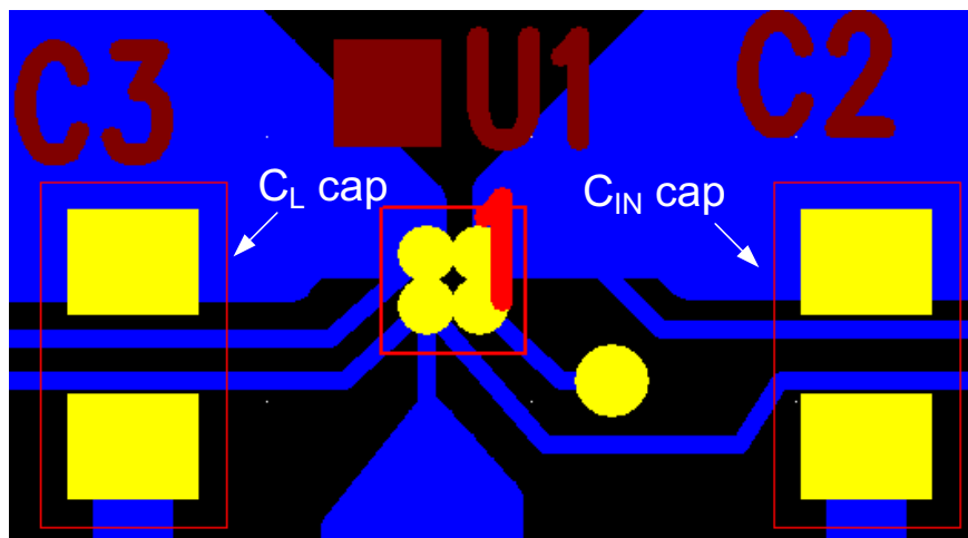
Figure 29. Layout Recommendation
