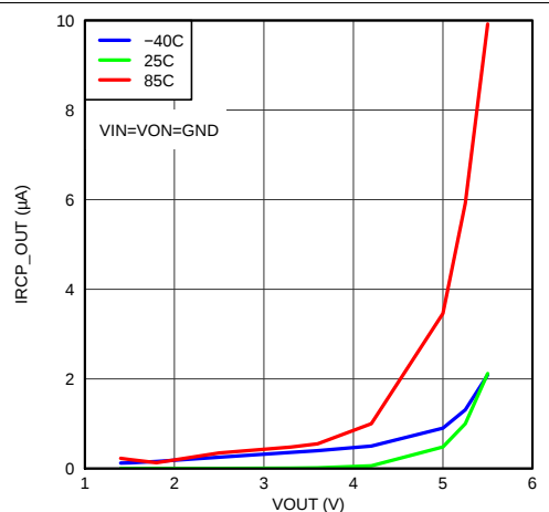
Figure 8. I_{RCP(Leak)} vs V_{OUT} (Measured on V_{OUT} )
