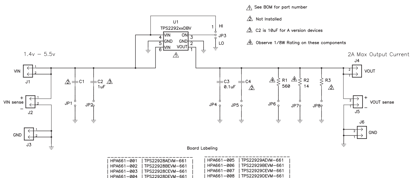
Figure 4. TPS2292xxEVM-661 Schematic
