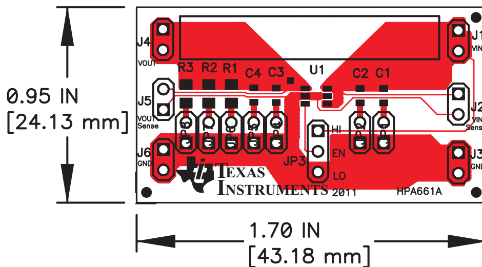
Figure 2. Top Layer
