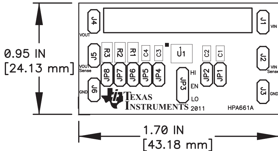
Figure 1. Top Assembly Layer
