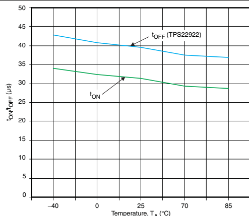
Figure 13. t_{ON}/t_{OFF} vs Temperature ( V_{IN} = 3.3 V)
