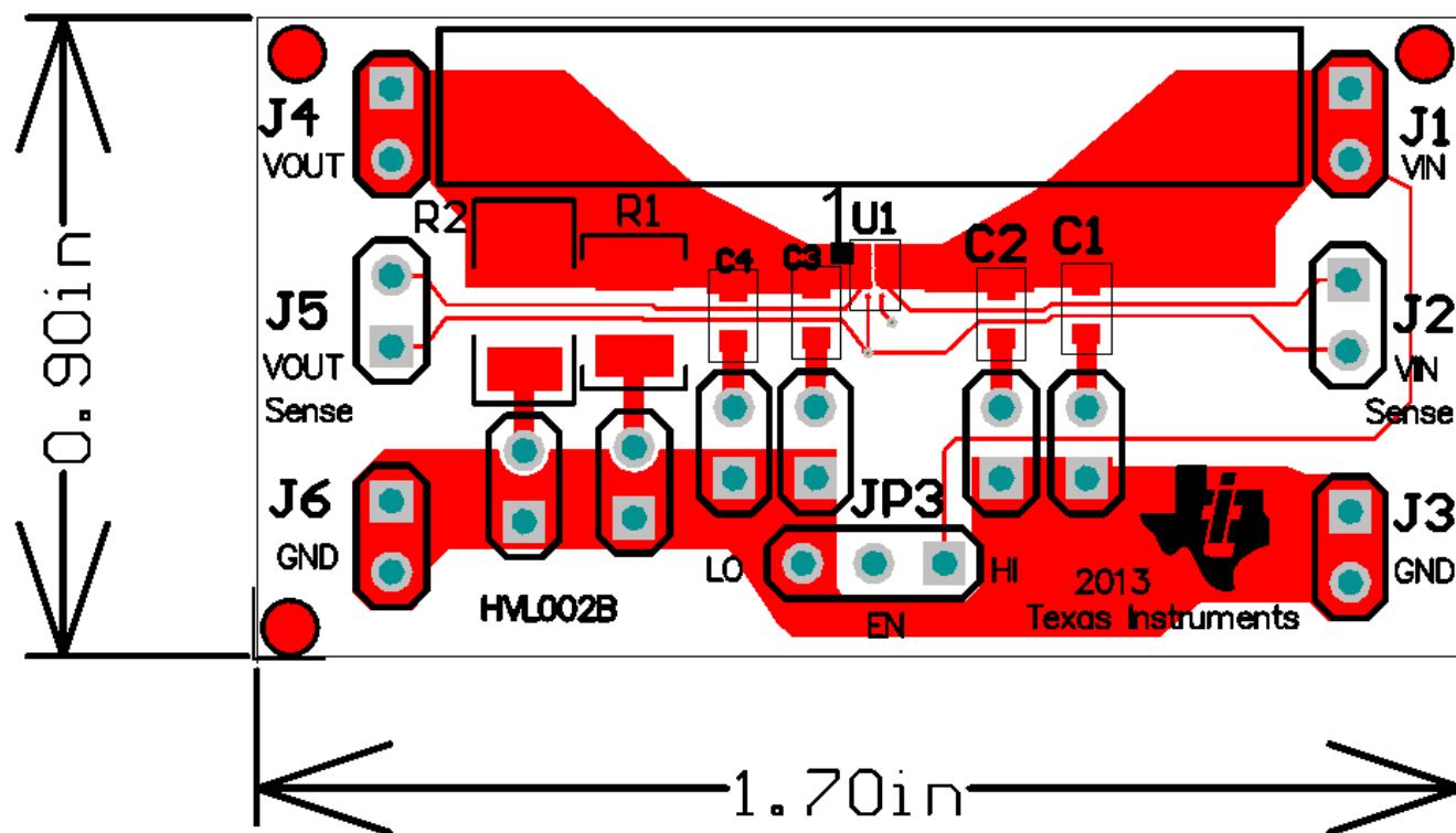
Figure 2. Top Layer
