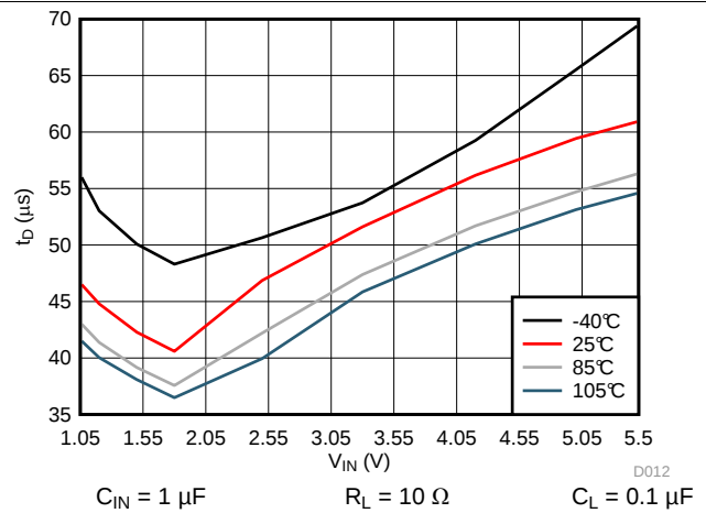
Figure 12. t_D vs V_{IN}
