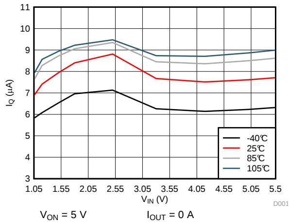
Figure 1. I_Q vs V_{IN} (TPS22914B/15B)
