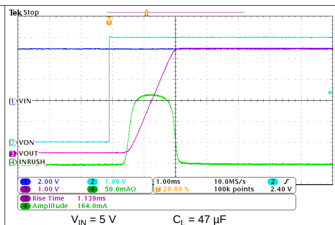
Figure 37. TPS22914C/15C Inrush Current
