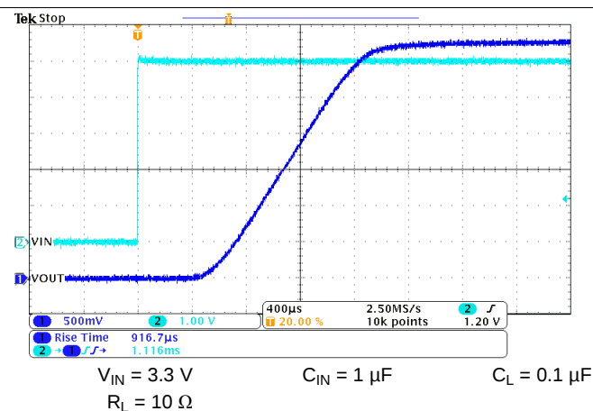
Figure 29. t_R at V_{IN} = 3.3\text{ V}
