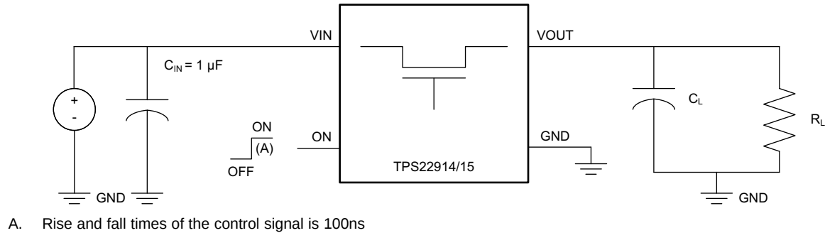
Figure 33. Test Circuit
