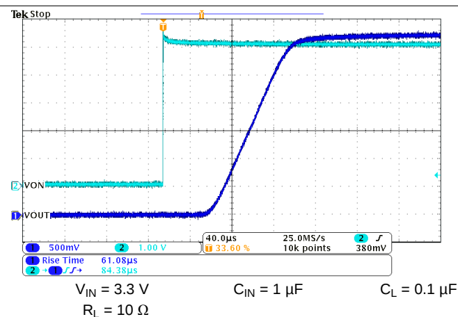
Figure 18. t_R at V_{IN} = 3.3\text{ V}
