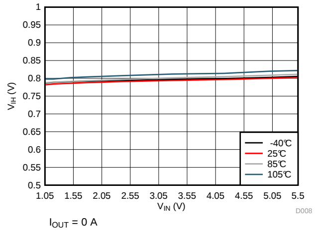
Figure 8. V_{IH} vs V_{IN}
