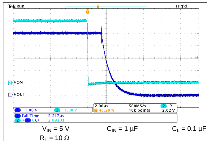
Figure 17. t_F at V_{IN} = 5\text{ V}
