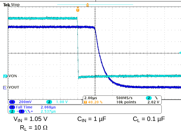
Figure 21. t_F at V_{IN} = 1.05\text{ V}
