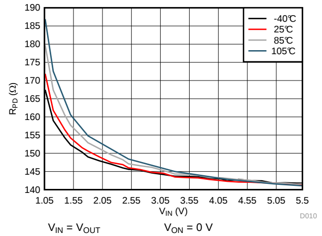
Figure 10. R_{PD} vs V_{IN}
