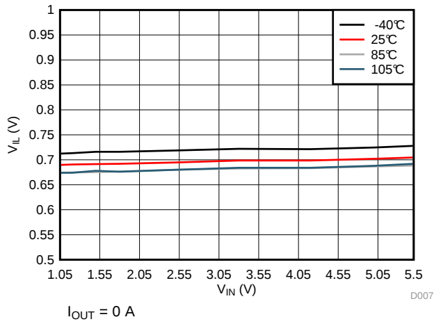
Figure 7. V_{IL} vs V_{IN}
