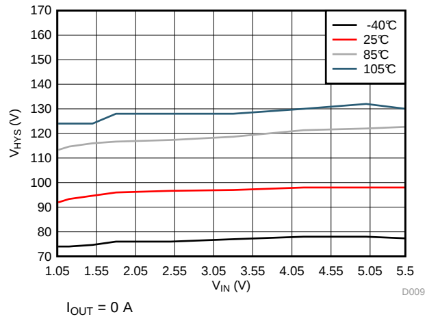
Figure 9. V_{HYS} vs V_{IN}
