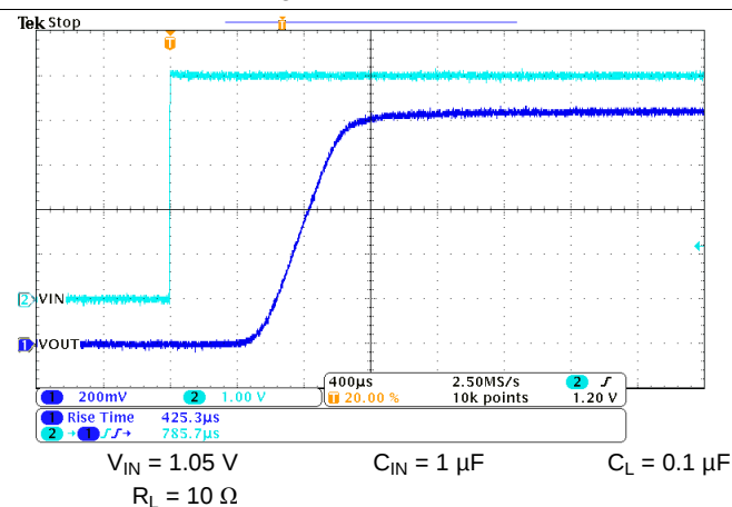
Figure 31. t_R at V_{IN} = 1.05\text{ V}
