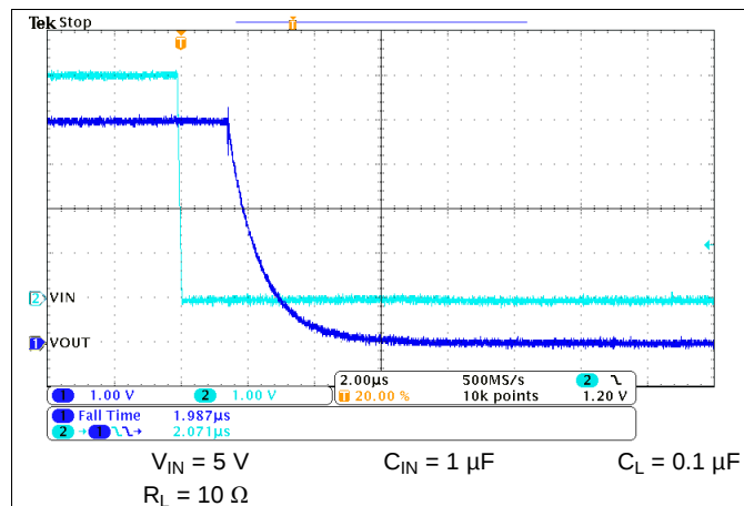
Figure 28. t_F at V_{IN} = 5\text{ V}
