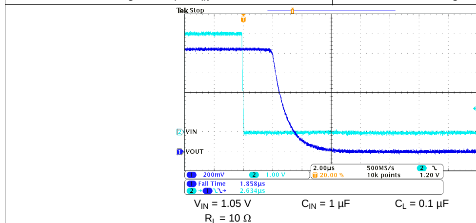
Figure 32. t_F at V_{IN} = 1.05\text{ V}
