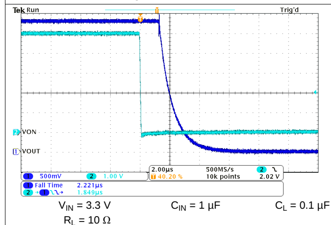
Figure 19. t_F at V_{IN} = 3.3\text{ V}
