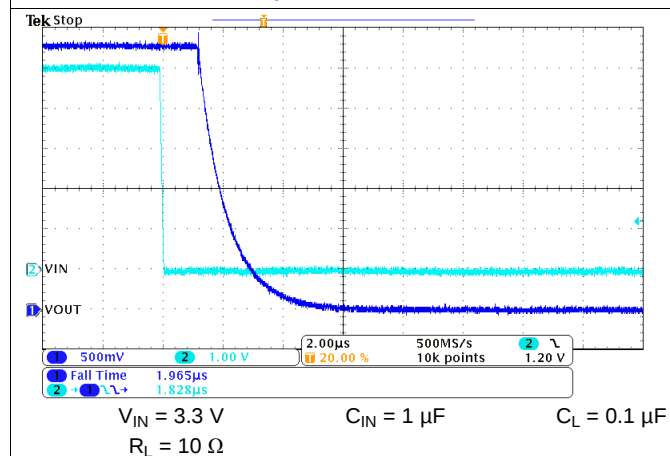
Figure 30. t_F at V_{IN} = 3.3\text{ V}
