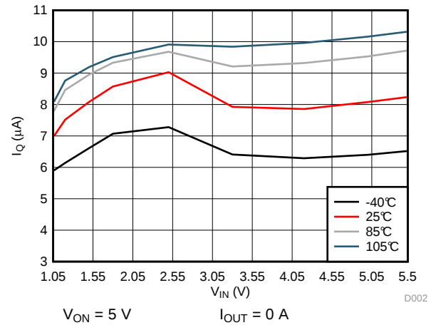
Figure 2. I_Q vs V_{IN} (TPS22914C/15C)
