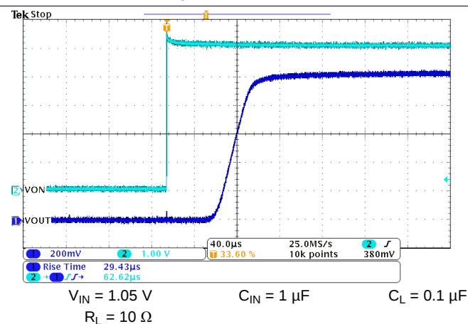
Figure 20. t_R at V_{IN} = 1.05\text{ V}
