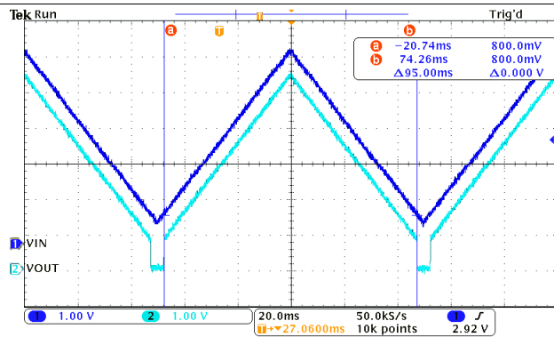
Figure 9. Under Voltage Lockout Response ( I_{OUT} = -100\text{mA} )
