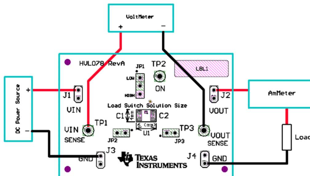
Figure 5. R_{ON} Setup
