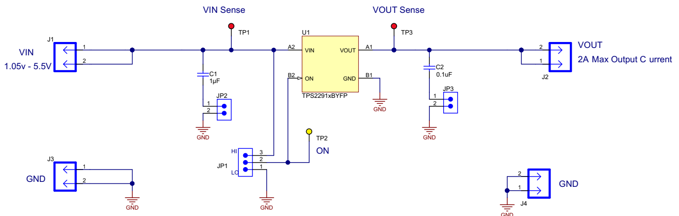
Figure 1. TPS22914/15EVM-078 Schematic
