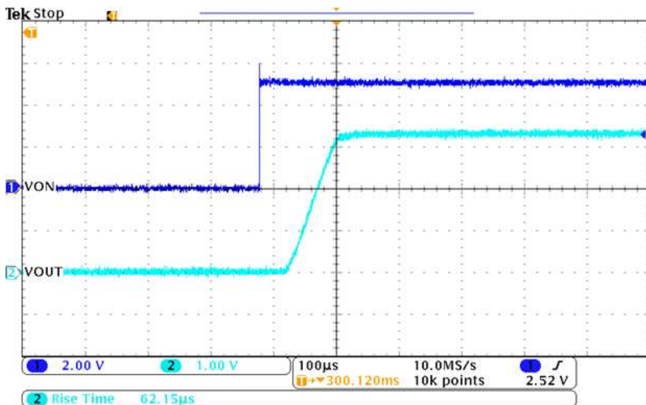
Figure 7. TPS22914/15 Vout t_r Example ( V_{IN} = 3.3V , R_L = 10\Omega )
