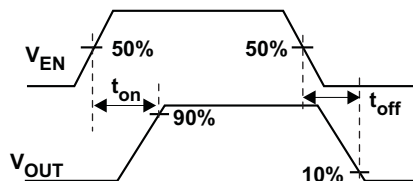
Figure 25. Enable Timing, Active High Enable
