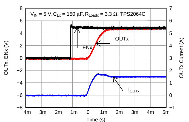
Figure 14. TPS2064C Enable into 3.3Ω and 150-µF Load
