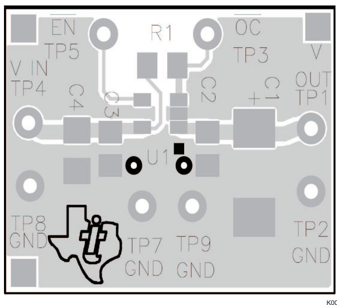
Figure 4. Top-Side Layout of TPS2041B EVM
