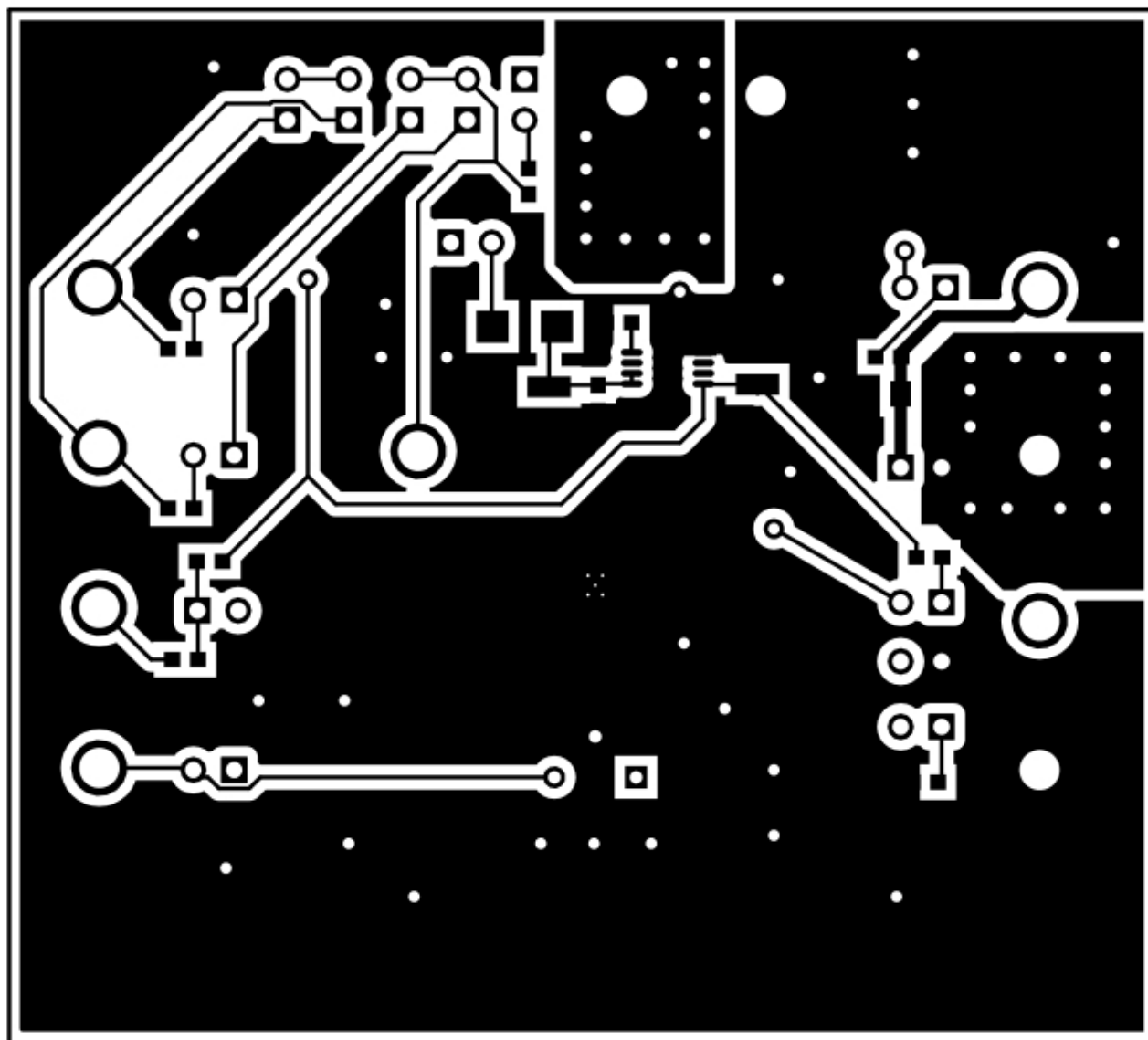
Figure 4. TPS1H000-Q1EVM Bottom Layer (Bottom View)
