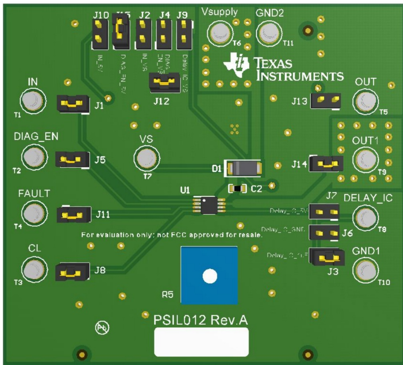
Figure 2. TPS1H000-Q1 EVM Component Placement (Top View)
