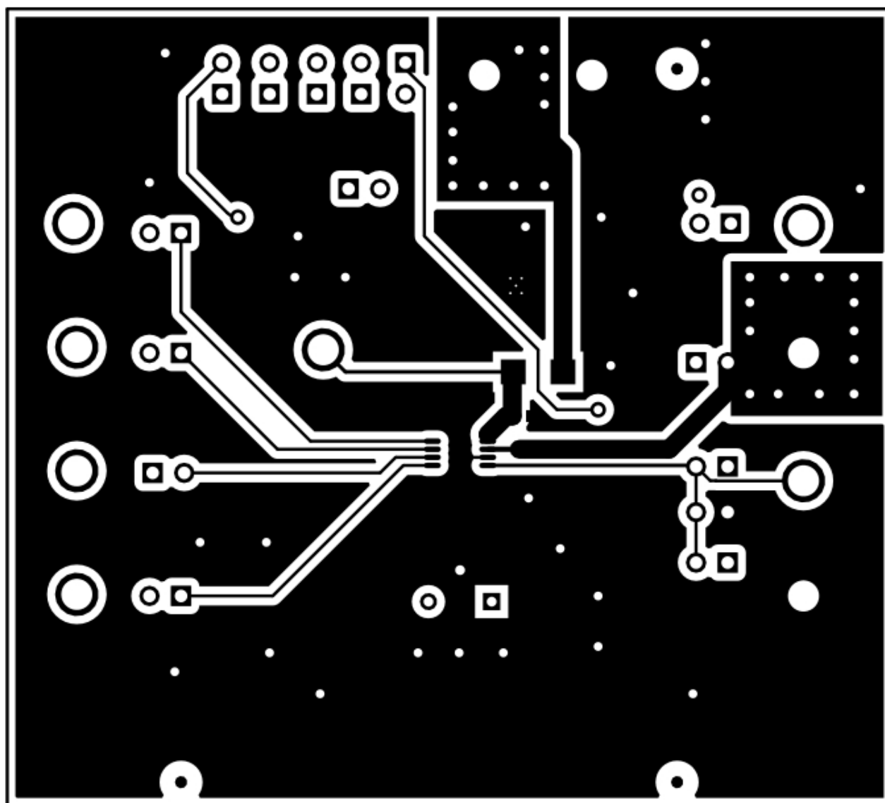
Figure 3. TPS1H000-Q1EVM Top Layer (Top View)
