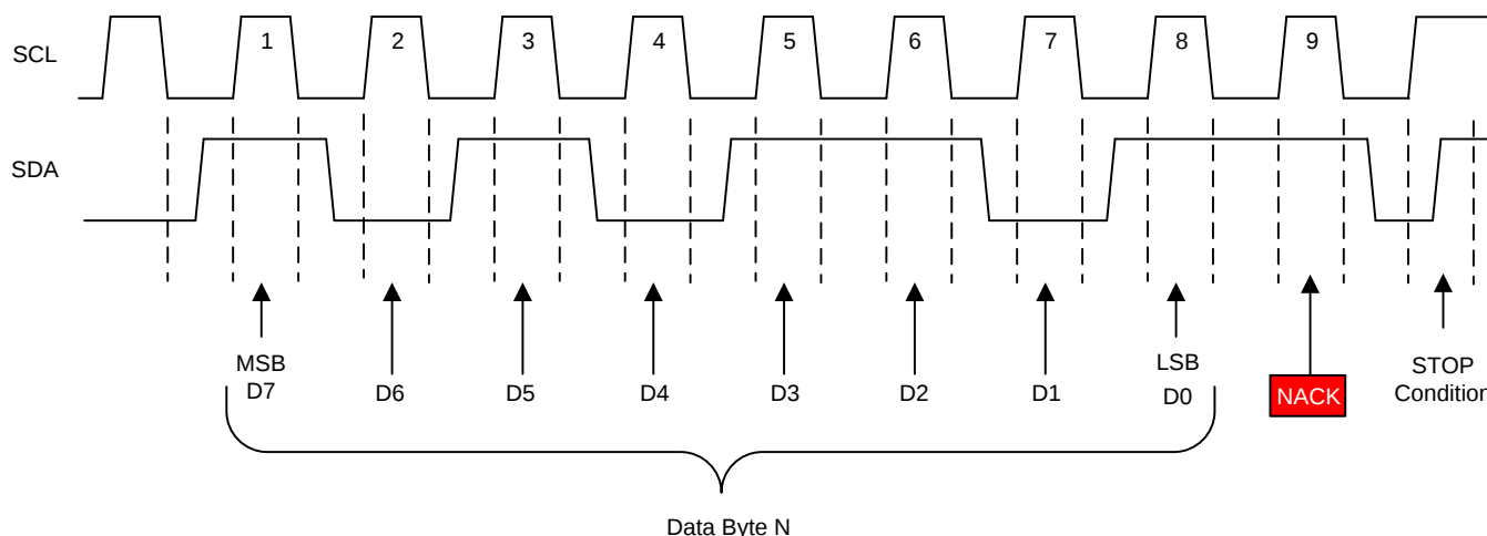
Figure 25. Example use of NACK
