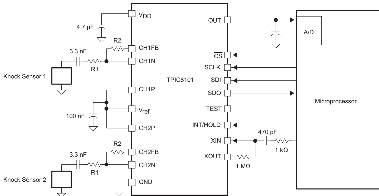
Figure 5. Application Schematic
