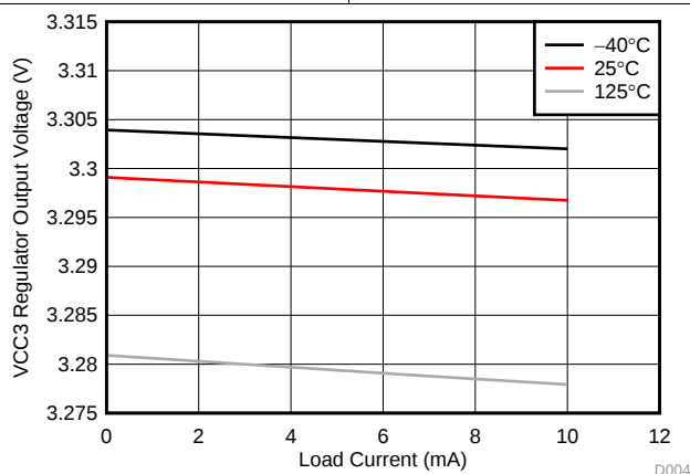
Figure 4-4. VCC3 Regulator Load Regulation Across Temperature (VDD = 4.5 V)
