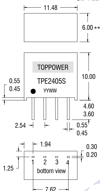
SIP Package
