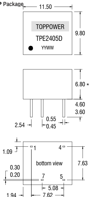
DIP Package
