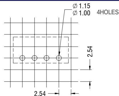
4 Pin SIP Package
