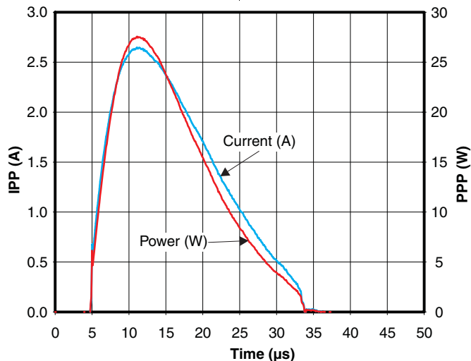
Figure 5. Pulse Waveform
