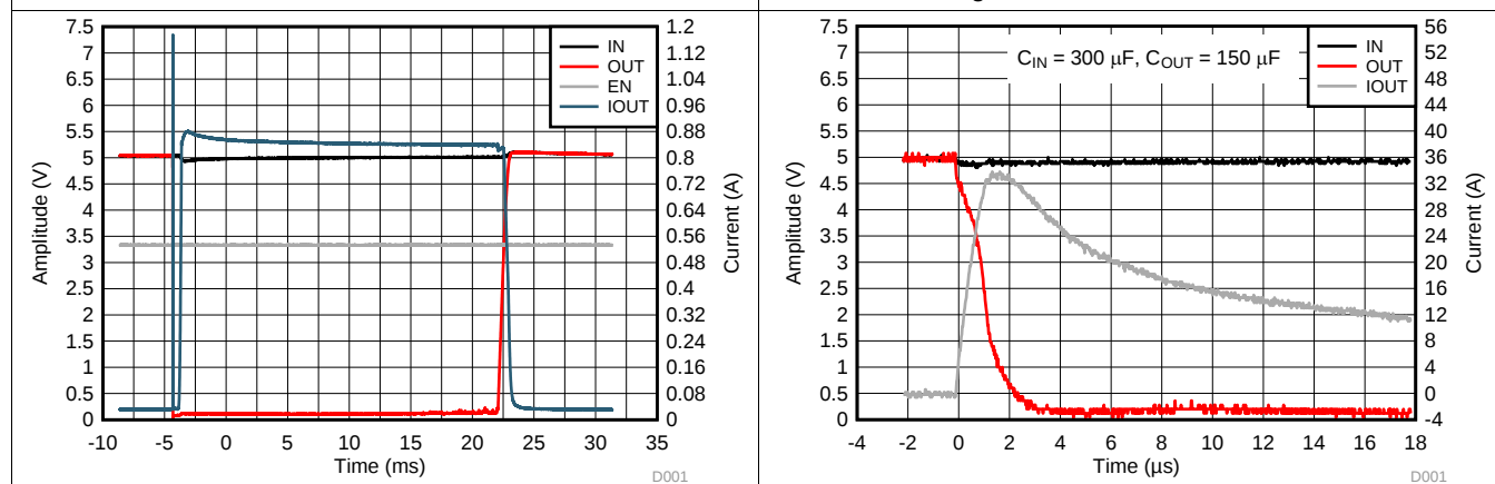
Figure 3. TPD3S014 Enable into Short
