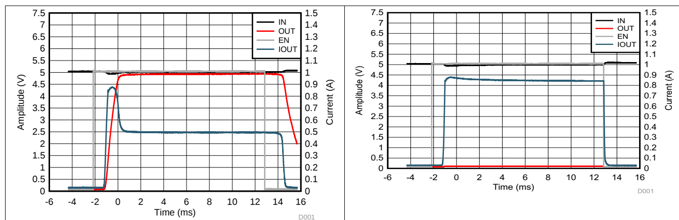
Figure 2. TPD3S014 Turn ON into 10 Ω
