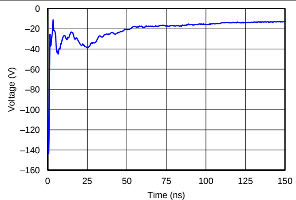
Figure 12. -8-kV Contact ESD Clamping
