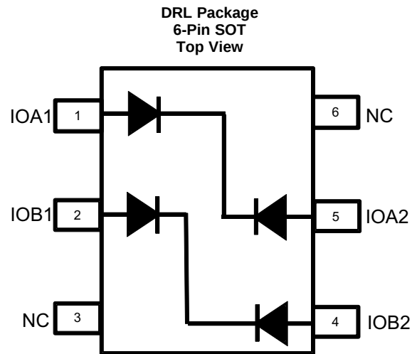
Pin Functions
