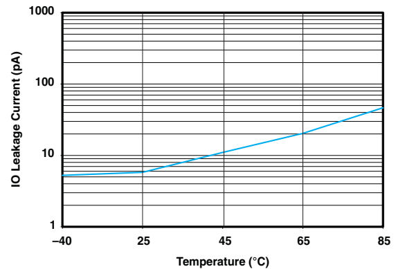
Figure 2. IO Leakage Current vs Temperature ( V_{CC} = 5\text{ V} )
