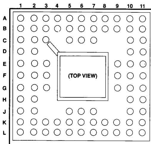
I/O Pin Assignments for the 84-Pin Ceramic Pin Grid Array Package
