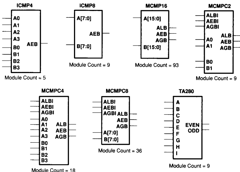
Figure 29. Comparators/Parity Checker
