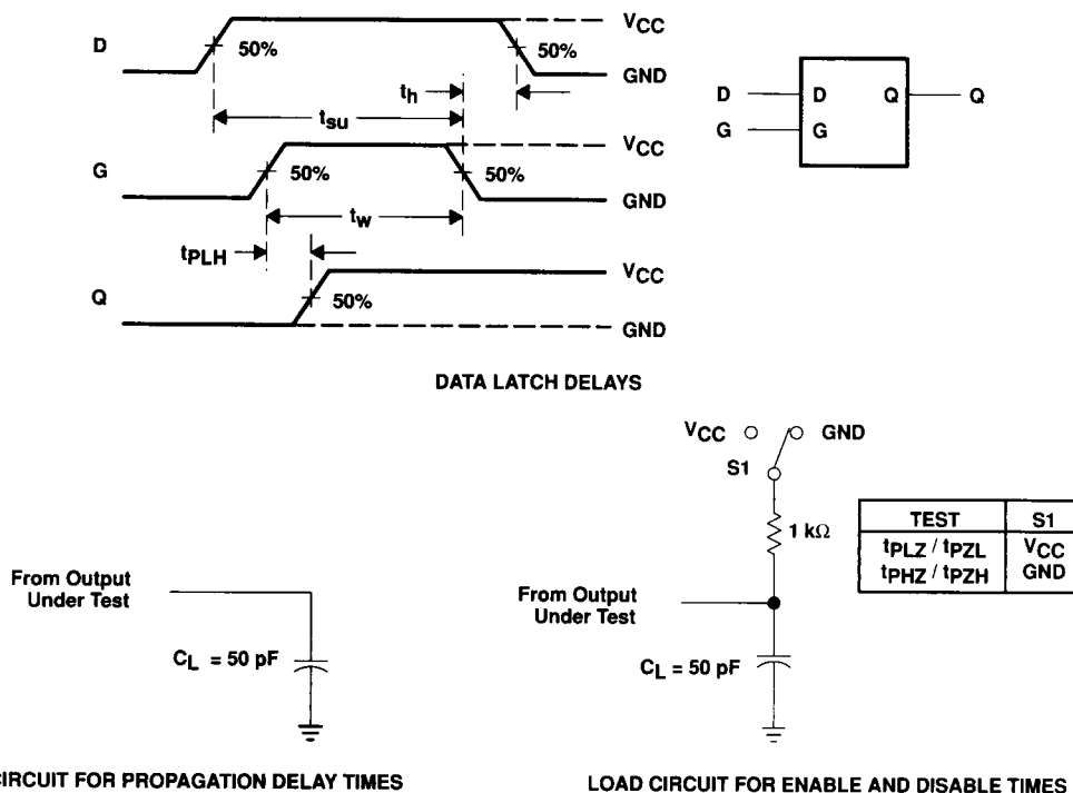
Figure 8. Symbols, Test Loads, and Voltage Waveforms (Continued)
