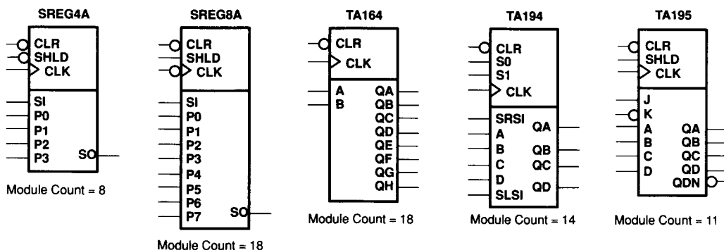
Figure 32. Shift Registers
