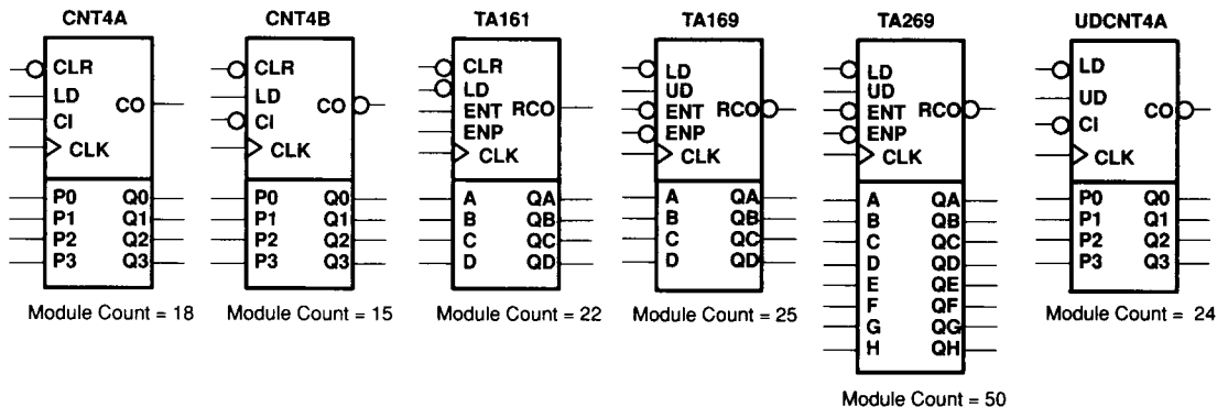
Figure 30. Counters
