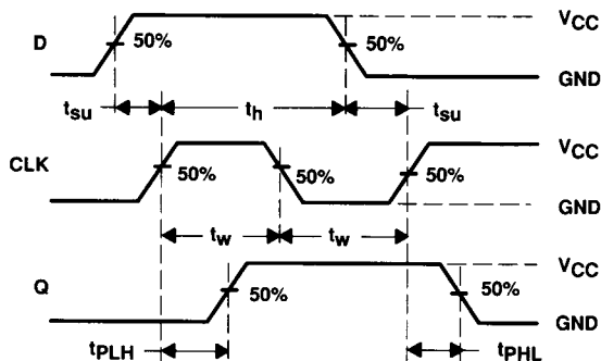
Figure 8. Symbols, Test Loads, and Voltage Waveforms
