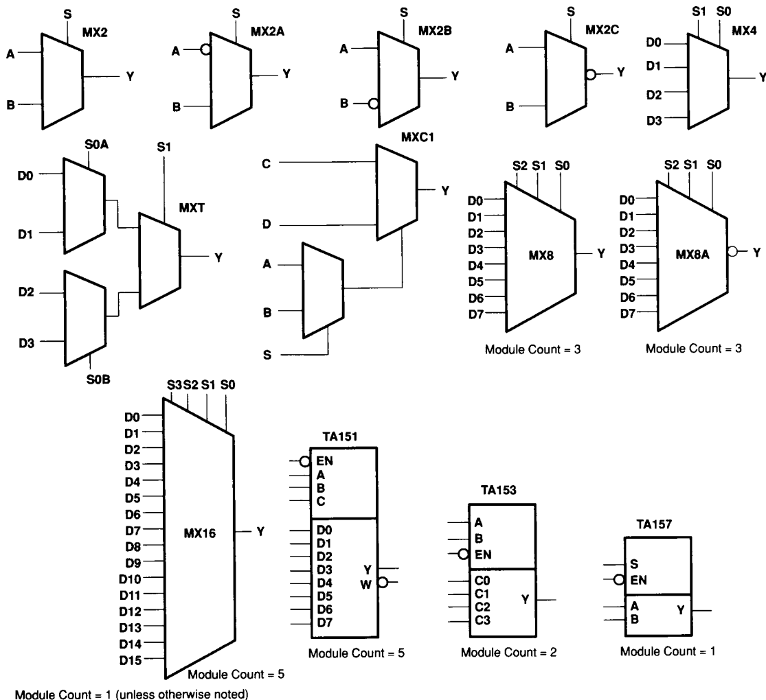
Figure 20. Multiplexers
