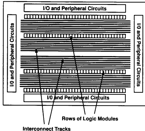
TPC10 Series FPGA Die Architecture
