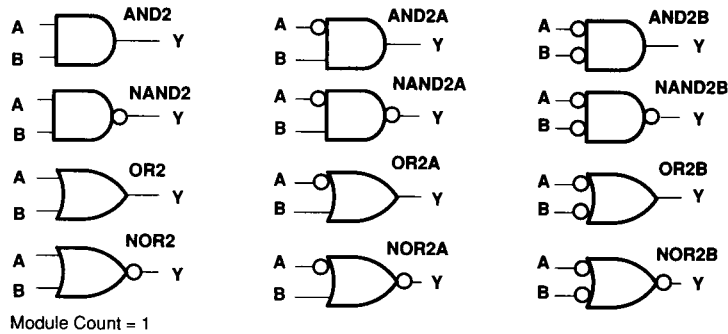
Figure 9. 2-Input Gates
