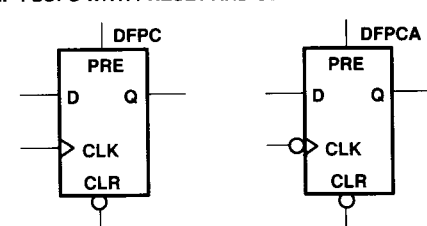
Figure 23. D-Type Flip-Flops
