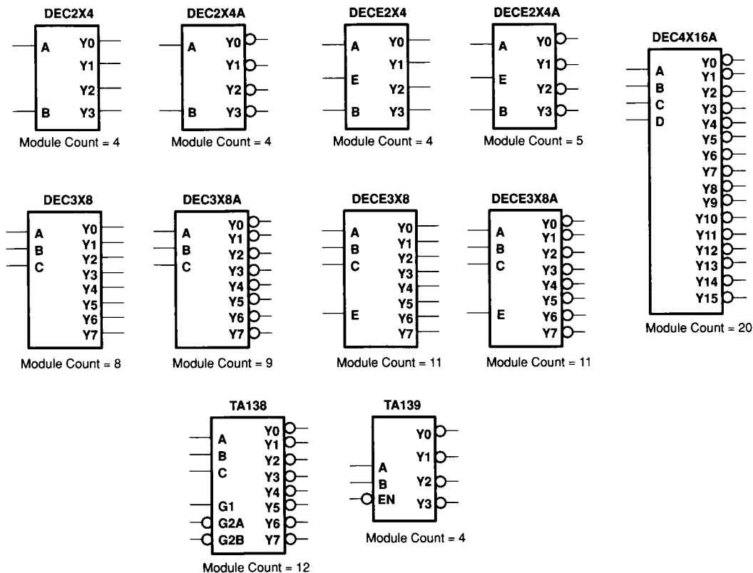
Figure 31. Decoders
