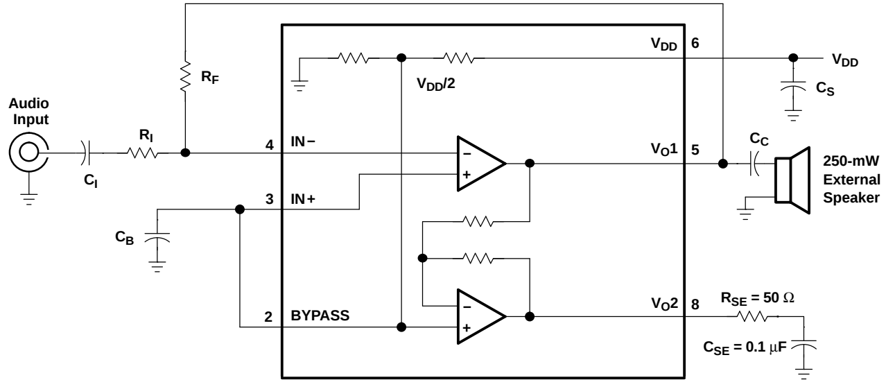
Figure 38. Singled-Ended Mode
