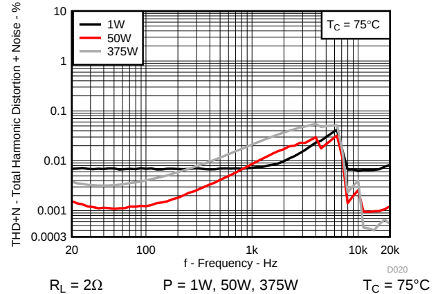
Figure 20. Total Harmonic Distortion+Noise vs Frequency
