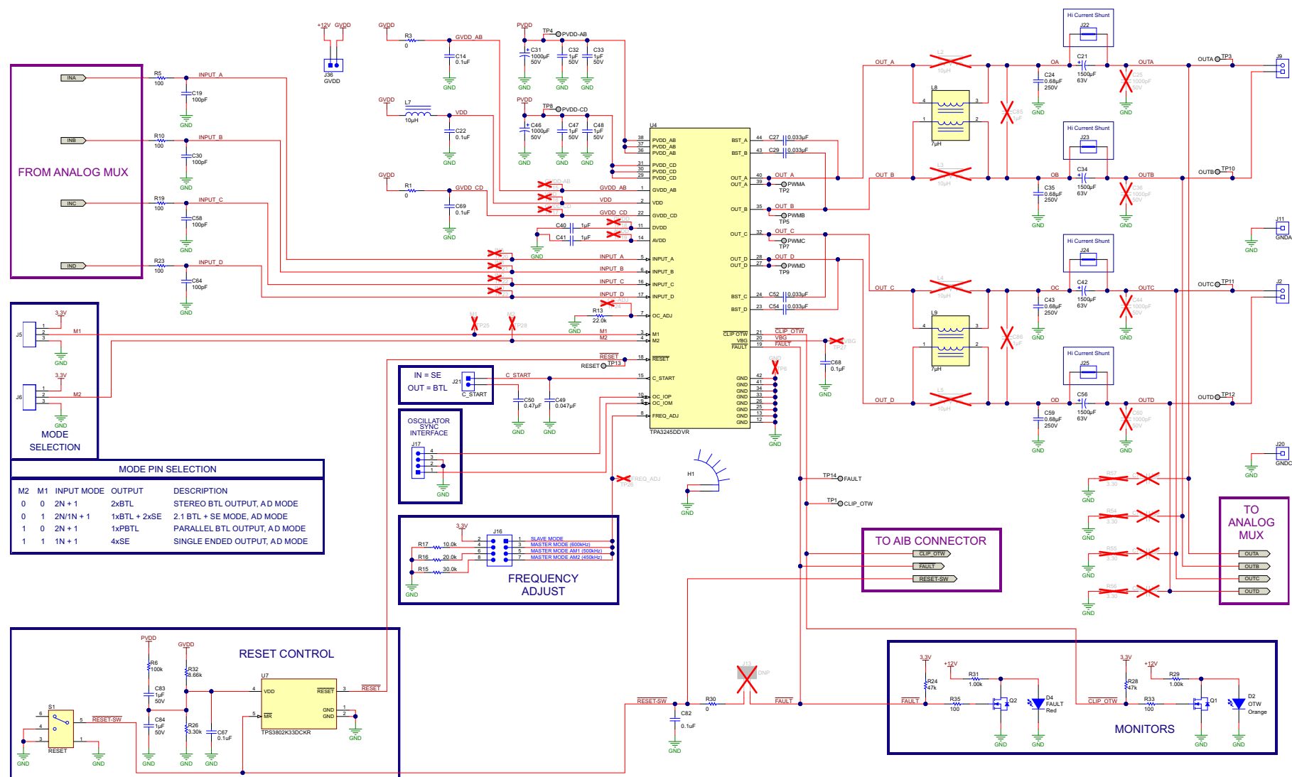
Figure 31. TPA3245EVM Schematic 2
