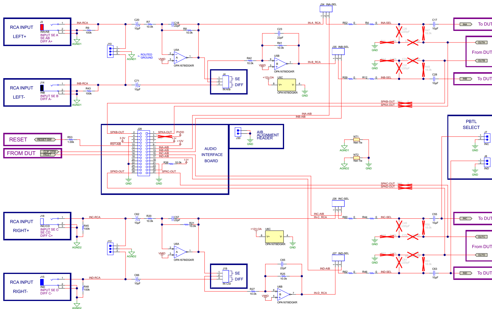
Figure 30. TPA3245EVM Schematic 1
