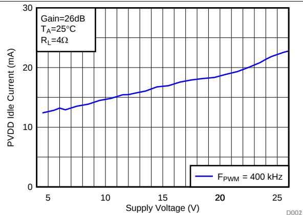
Figure 1. Idle Current vs PVCC
