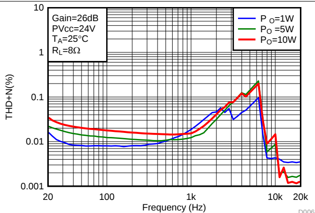
Figure 3. Total Harmonic Distortion + Noise (BTL) vs Frequency
