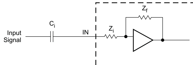
Figure 26. Input Impedance
