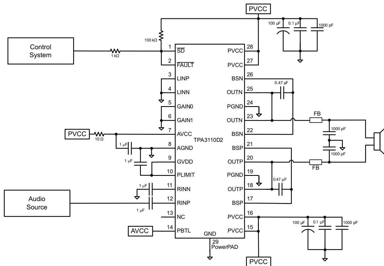
Figure 38. Stereo Class-D Amplifier with PBTB Output and Single-Ended Input
