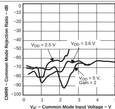
Figure 26. Common-Mode Rejection Ratio versus Common-Mode Input Voltage
