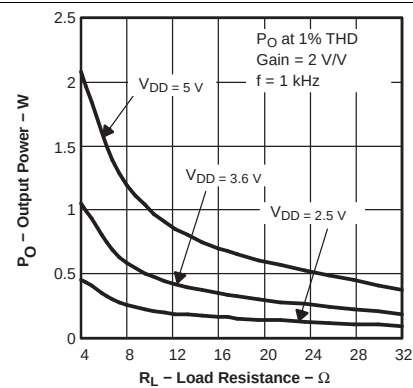
Figure 36. Output Power versus Load Resistance
