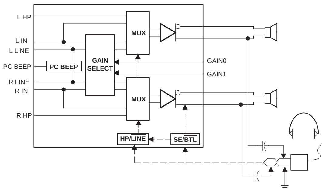
Figure 3–4. TPA0222 Amplifier IC
