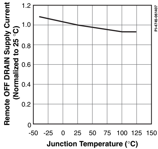
Figure 50. Remote OFF DRAIN Supply Current vs. Temperature.
