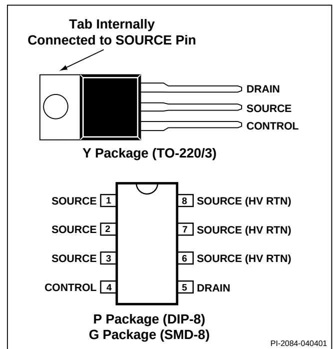
Figure 3. Pin Configuration.
