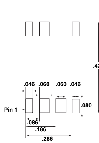
Solder Pad Dimensions
