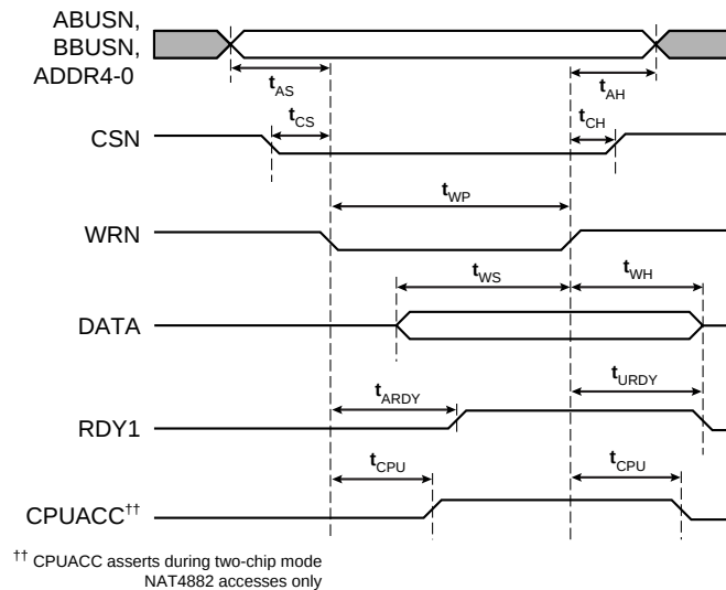
Figure 9. CPU Write
