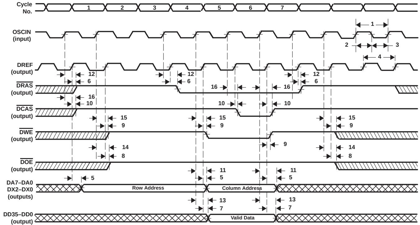
Figure 35. DRAM Write Cycle
