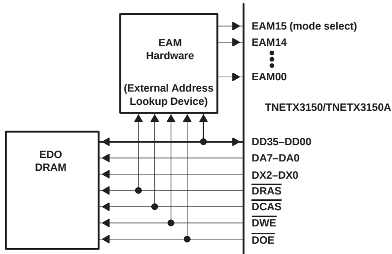
Figure 14. EAM Interface
