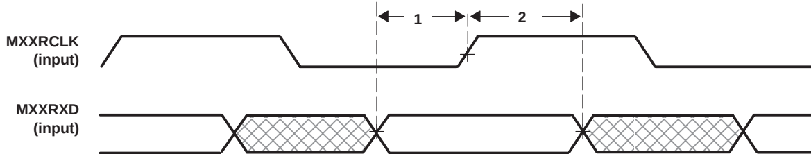
Figure 46. Ports (03–14) Receive Interface Timing
