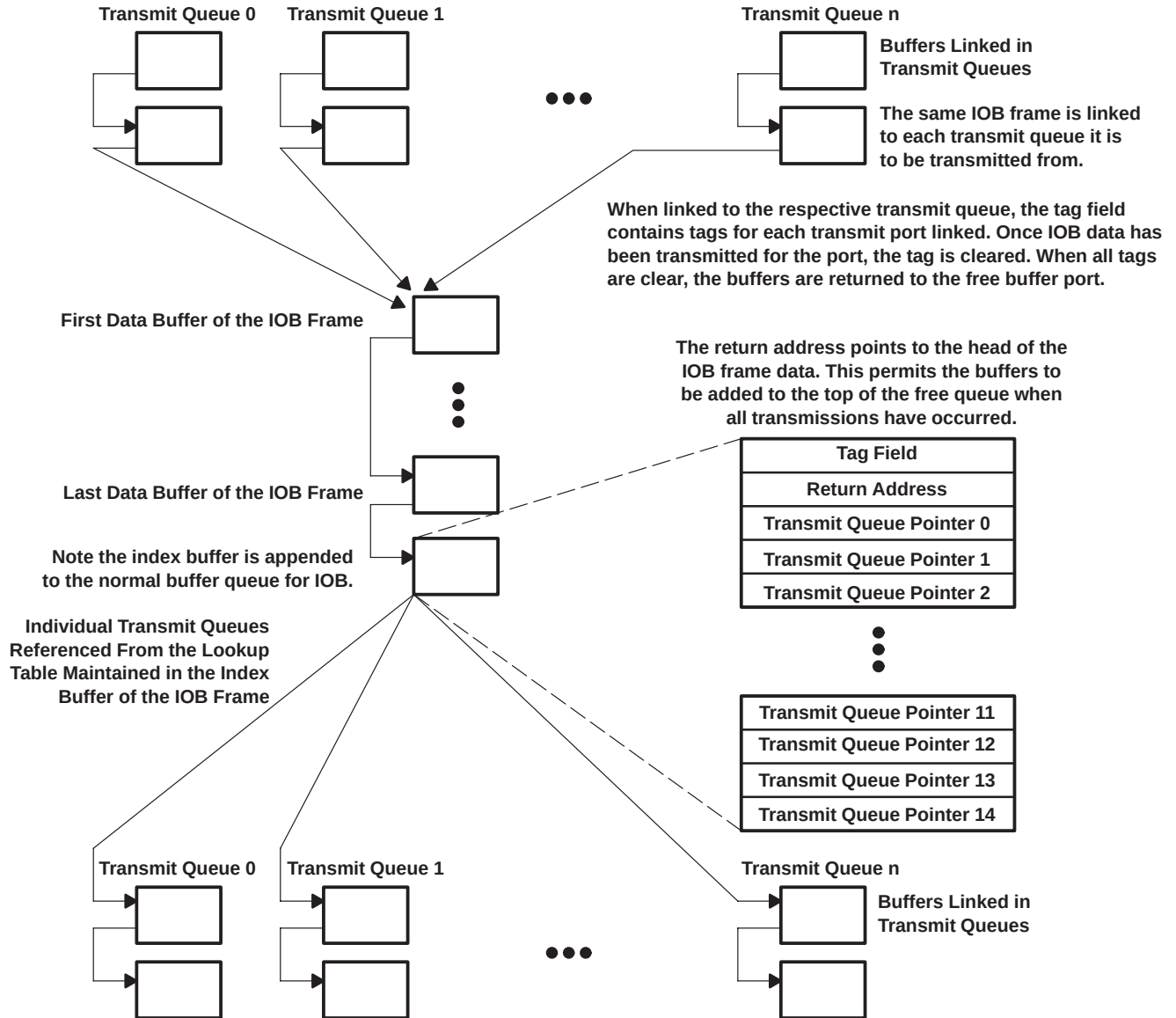
Figure 30. IOB Operation
