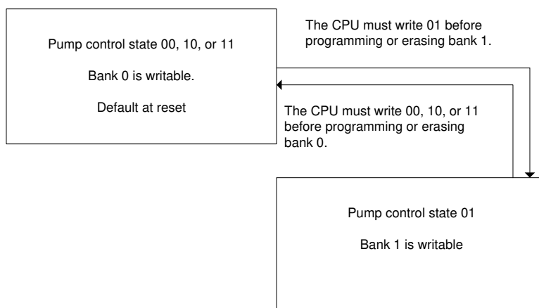
Figure 3-19. PUMP_OWNERSHIP Configuration
