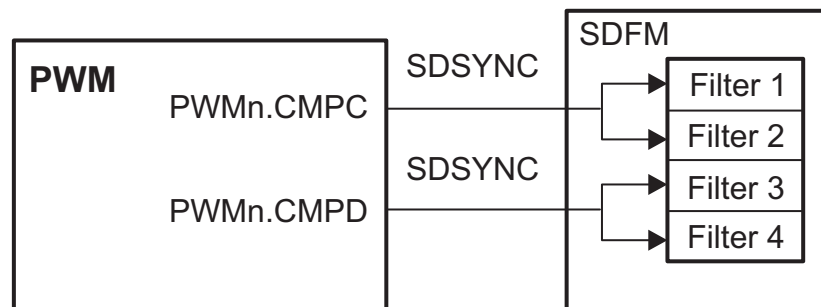
Figure 13-8. SDSYNC Event
