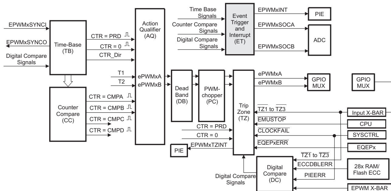
Figure 14-43. Event-Trigger Submodule
