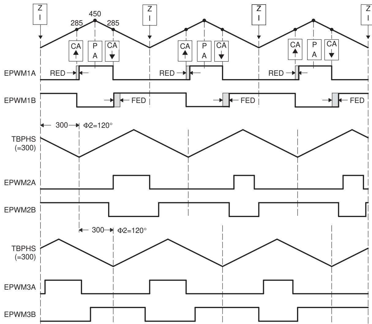
Figure 14-71. 3-Phase Interleaved DC/DC Converter Waveforms for Figure 14-70
