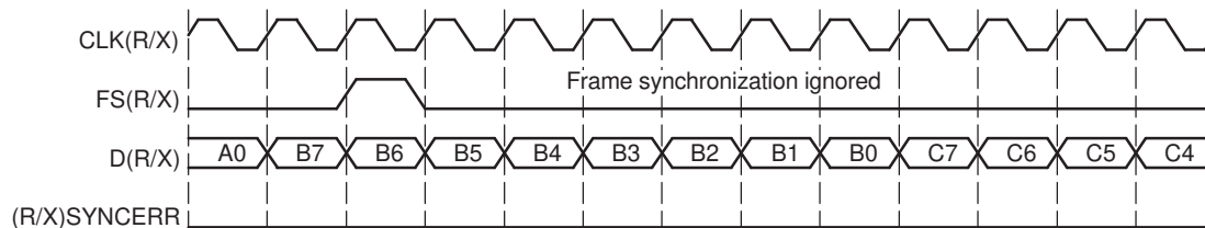
Figure 20-44. Unexpected Frame-Synchronization Pulse With (R/X)FIG = 1
