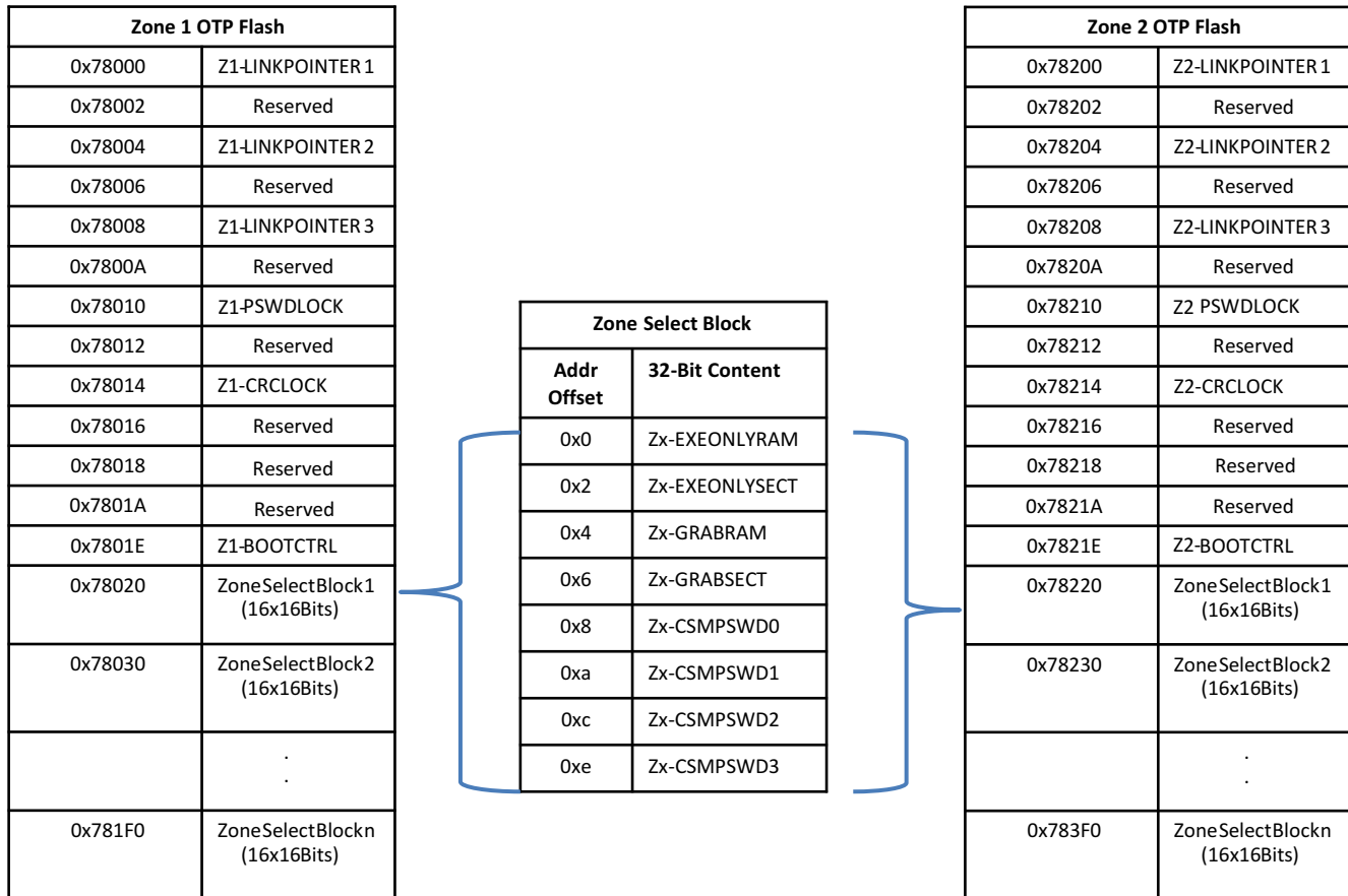
Figure 3-21. Location of Zone-Select Block Based on Link-Pointer
