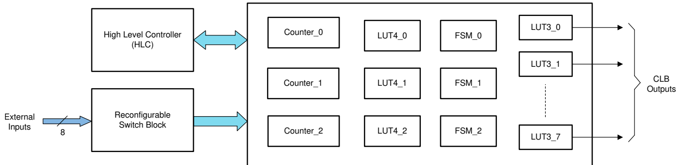
Figure 25-7. The CLB Tile Submodules
