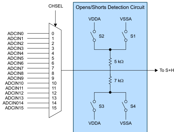
Figure 10-11. Opens/Shorts Detection Circuit
