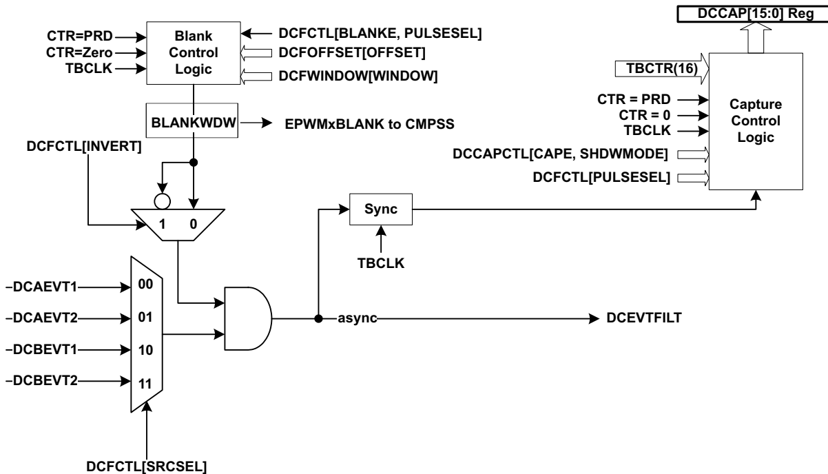
Figure 14-54. Event Filtering
