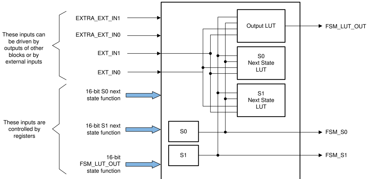
Figure 25-9. FSM Block
