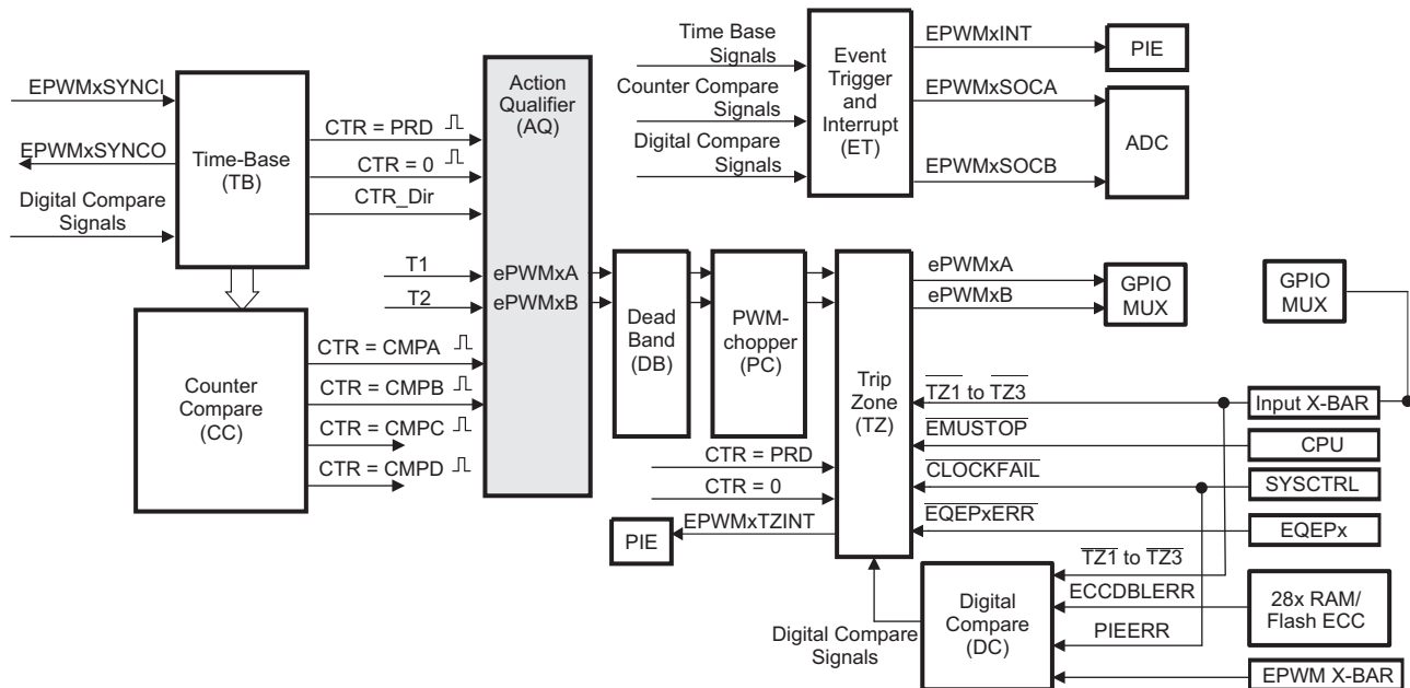
Figure 14-19. Action-Qualifier Submodule
