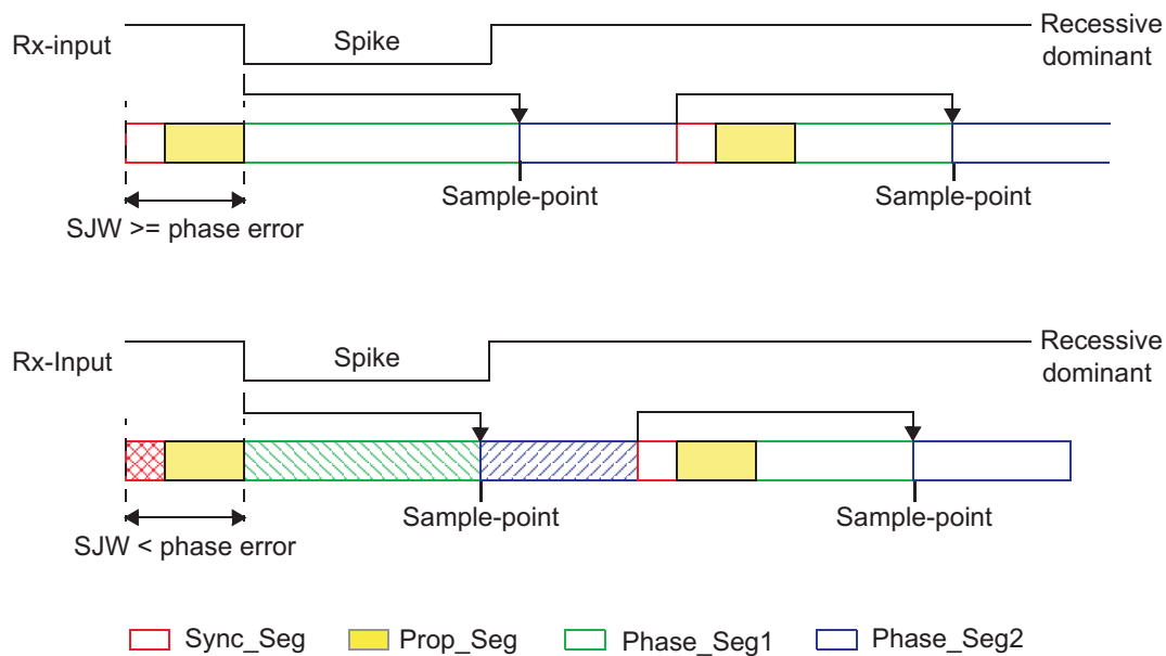
Figure 21-15. Filtering of Short Dominant Spikes
