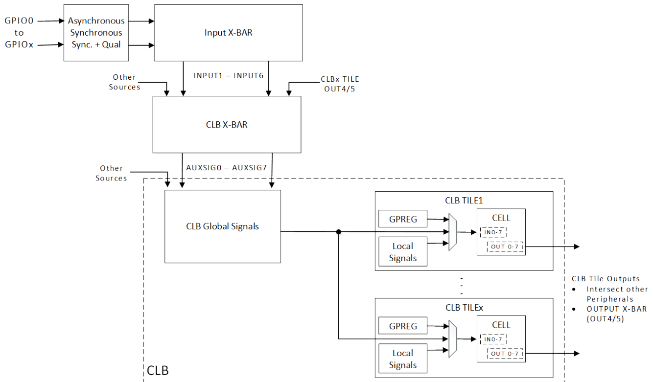
Figure 25-4. GPIO to CLB Tile Connections
