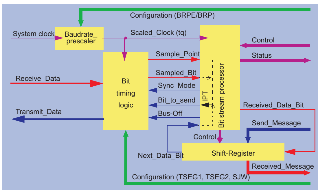
Figure 21-16. Structure of the CAN Core's CAN Protocol Controller
