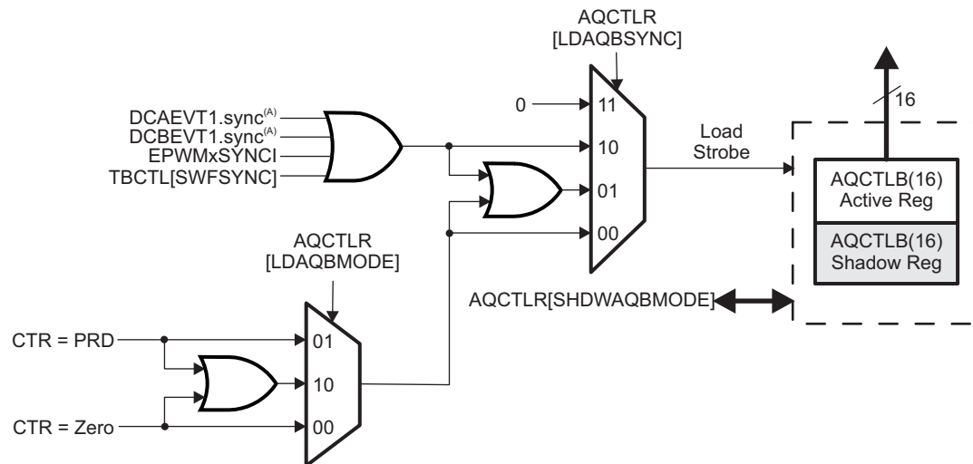
Figure 14-23. AQCTL[SHDWAQBMODE]
