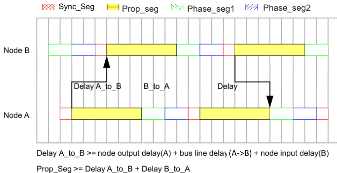
Figure 21-13. The Propagation Time Segment
