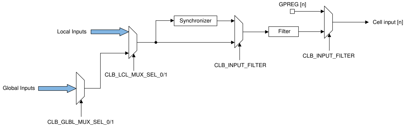
Figure 25-3. CLB Input Mux and Filter
