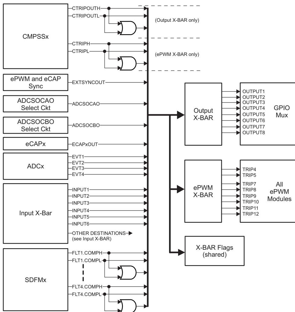
Figure 14-57. ePWM X-BAR
