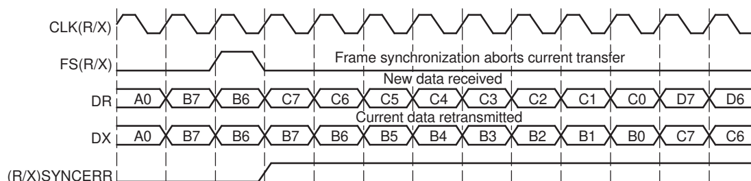
Figure 20-51. Unexpected Frame-Synchronization Pulse With (R/X) FIG = 0
