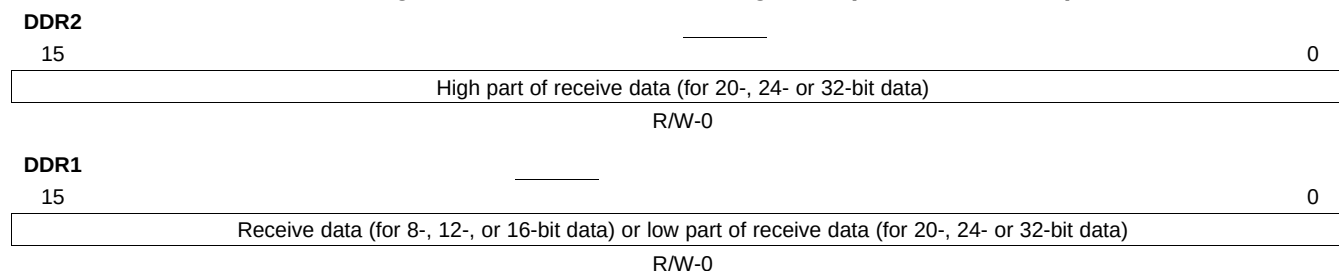
Figure 20-67. Data Receive Registers (DDR2 and DDR1)
