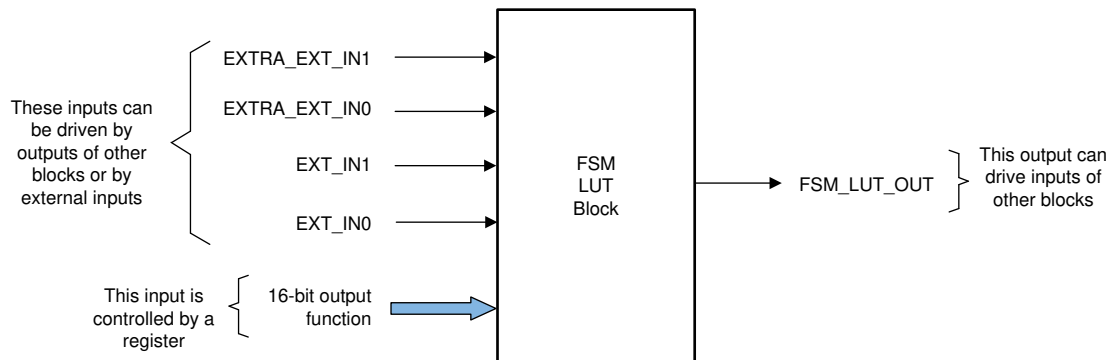
Figure 25-10. FSM LUT Block
