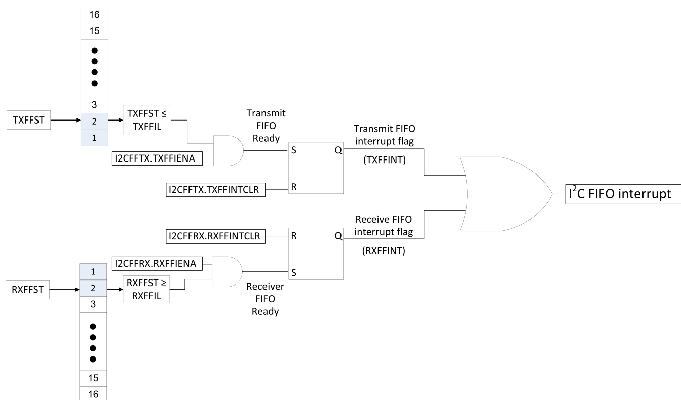
Figure 19-17. I2C_FIFO_interrupt
