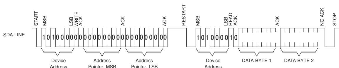
Figure 4-11. Random Read
