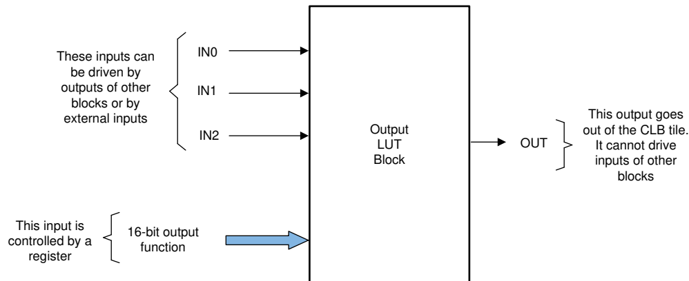
Figure 25-12. Output LUT Block
