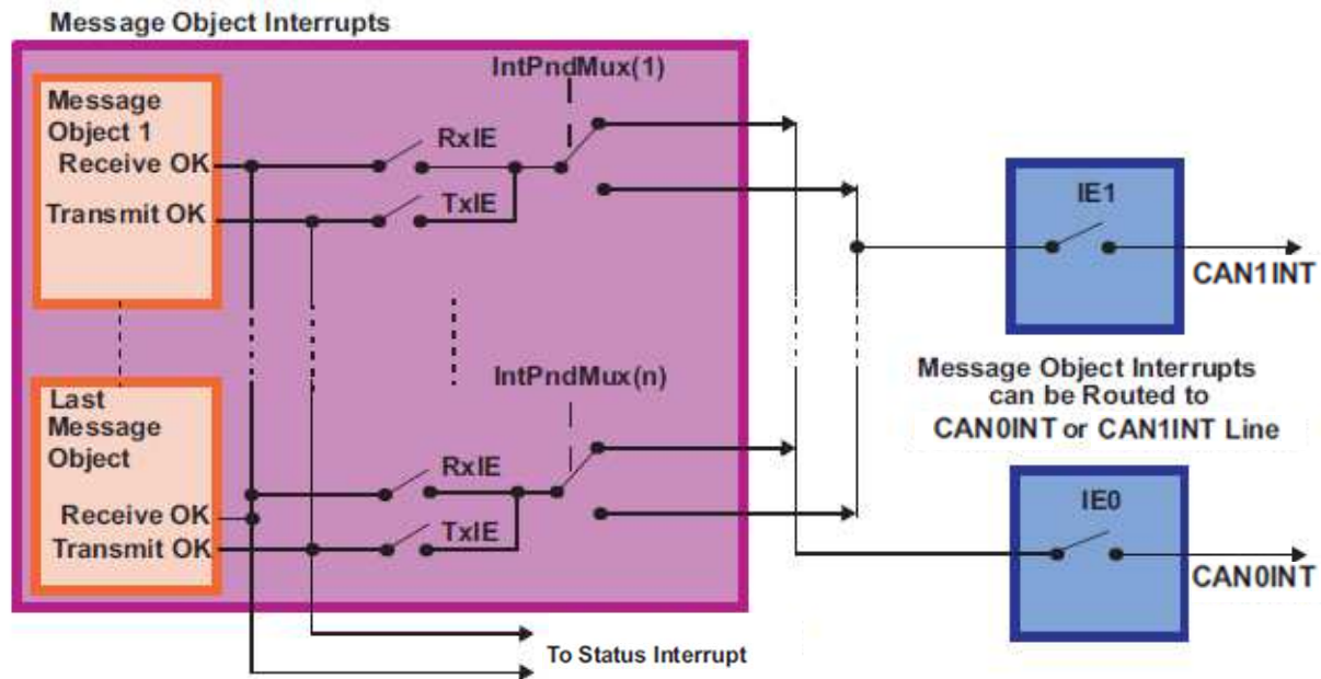
Figure 21-7. CAN Interrupt Topology 2
