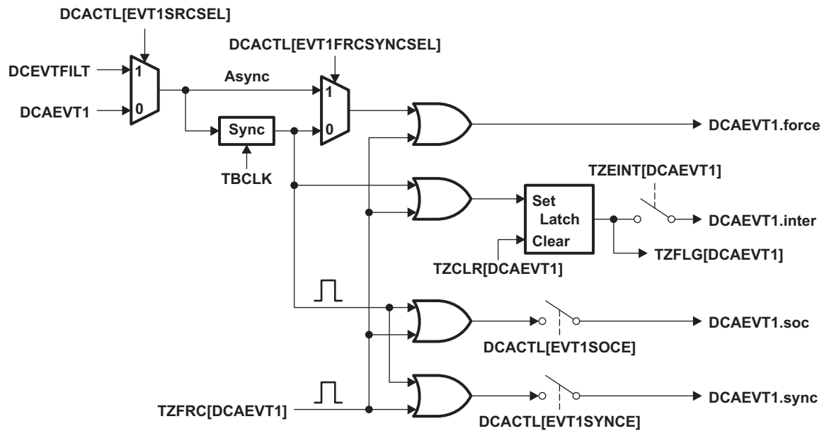
Figure 14-50. DCAEVT1 Event Triggering
