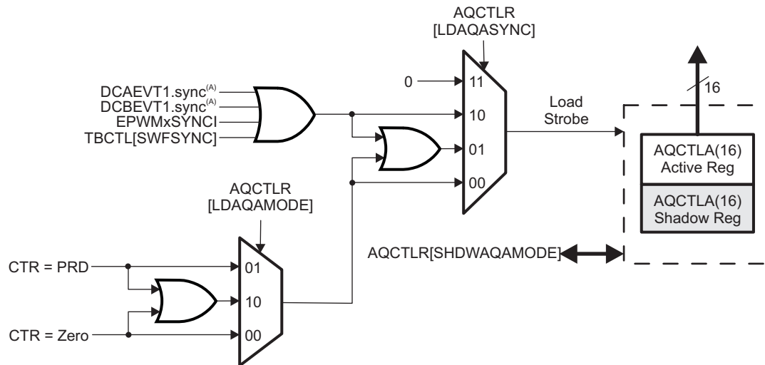
Figure 14-22. AQCTL[SHDWAQAMODE]
