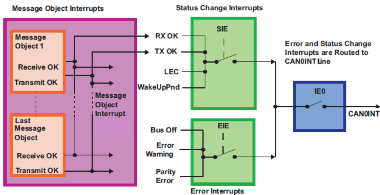
Figure 21-6. CAN Interrupt Topology 1
