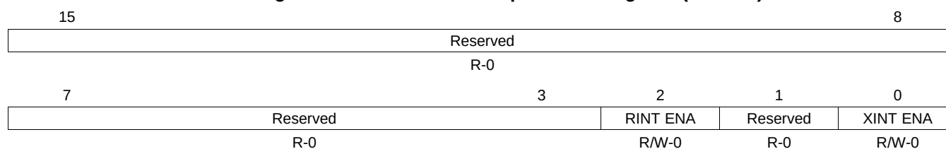
Figure 20-82. McBSP Interrupt Enable Register (MFFINT)
