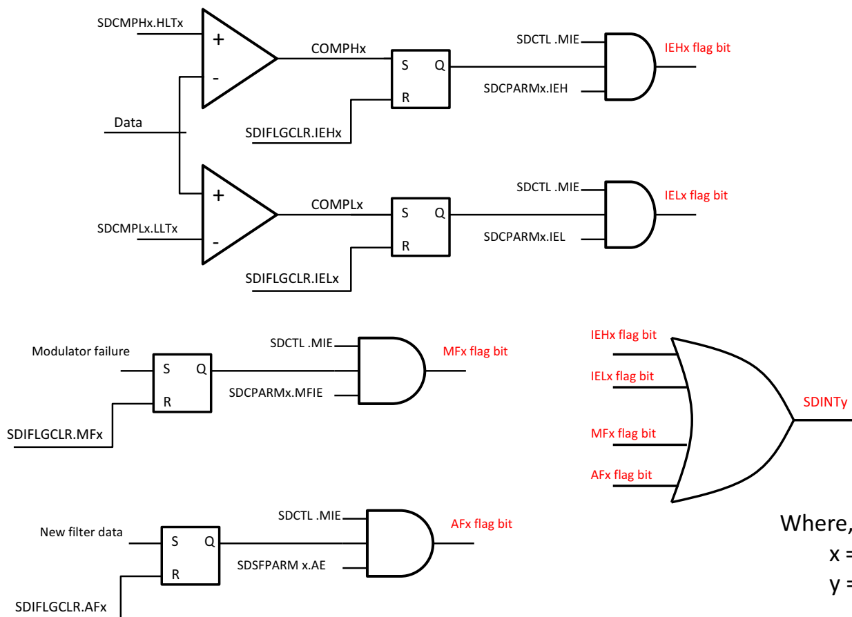
Figure 13-10. SDFM Interrupt Unit
