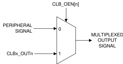
Figure 25-6. Peripheral Signal Multiplexer
