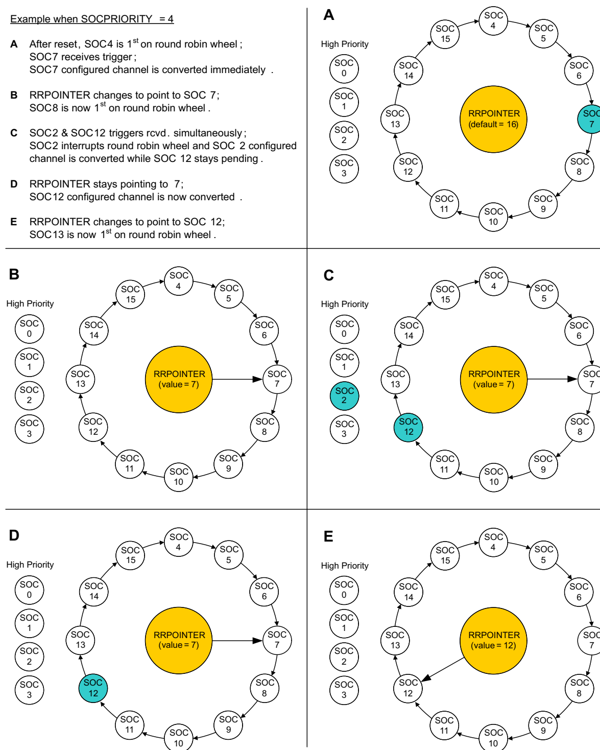
Figure 10-6. High Priority Example
