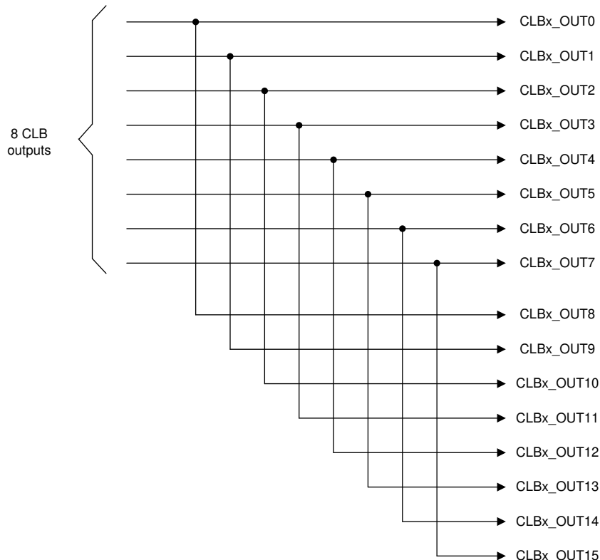
Figure 25-5. CLB Outputs
