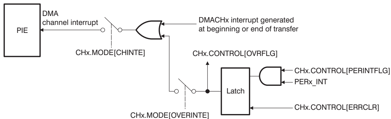
Figure 5-8. Overflow Detection Logic
