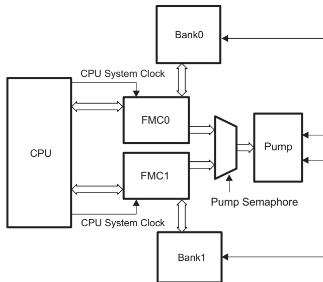
Figure 3-16. FMC Interface with Core, Bank and Pump
