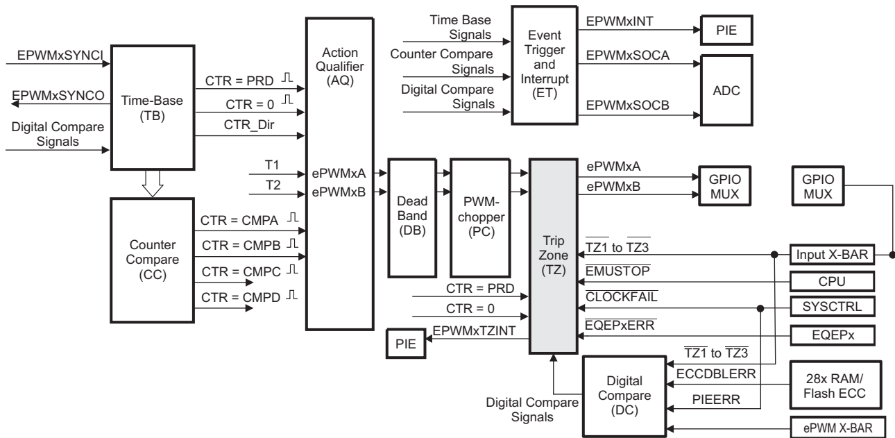
Figure 14-40. Trip-Zone Submodule
