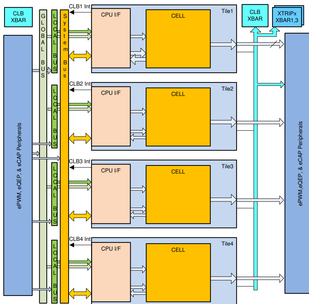
Figure 25-1. Block Diagram of the CLB Subsystem in the Device
