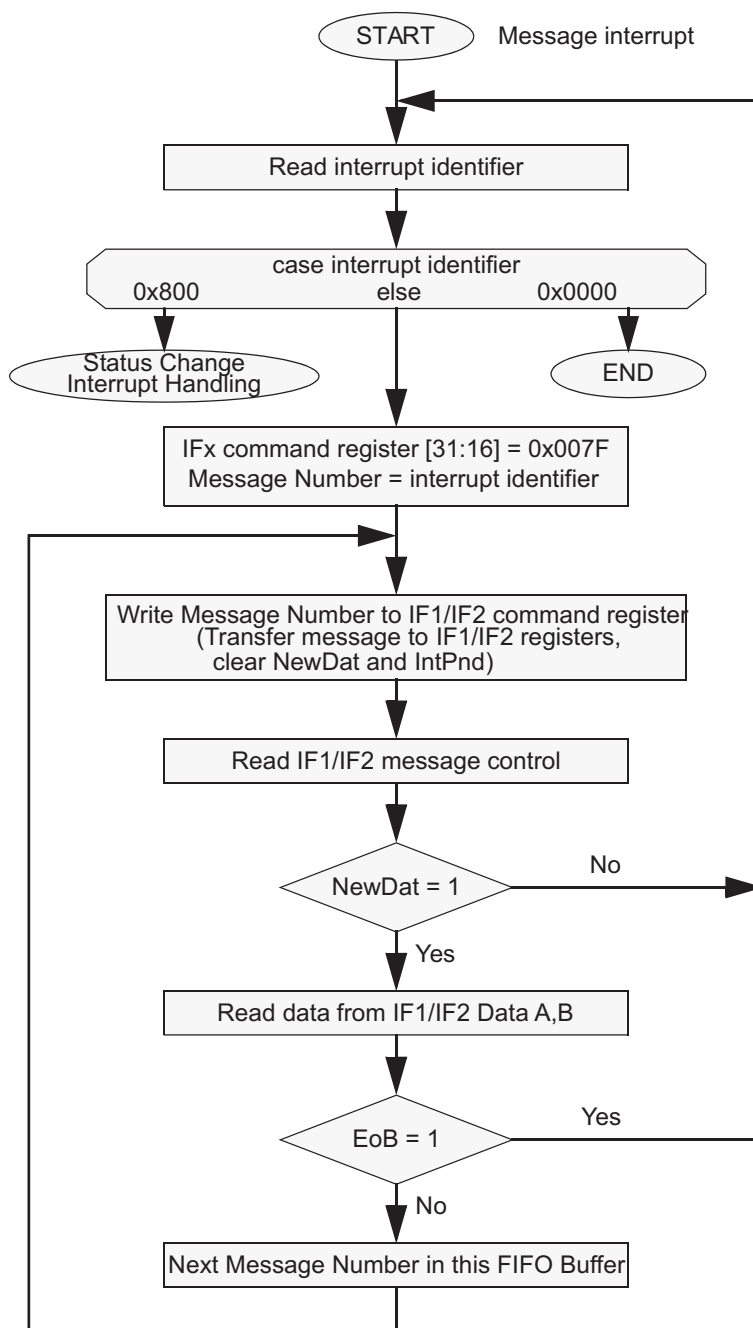
Figure 21-11. CPU Handling of a FIFO Buffer (Interrupt Driven)
