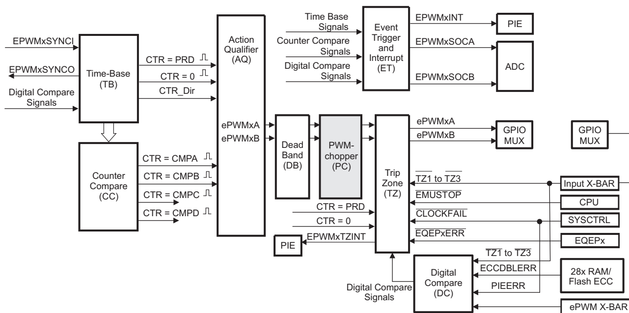
Figure 14-35. PWM Chopper Submodule
