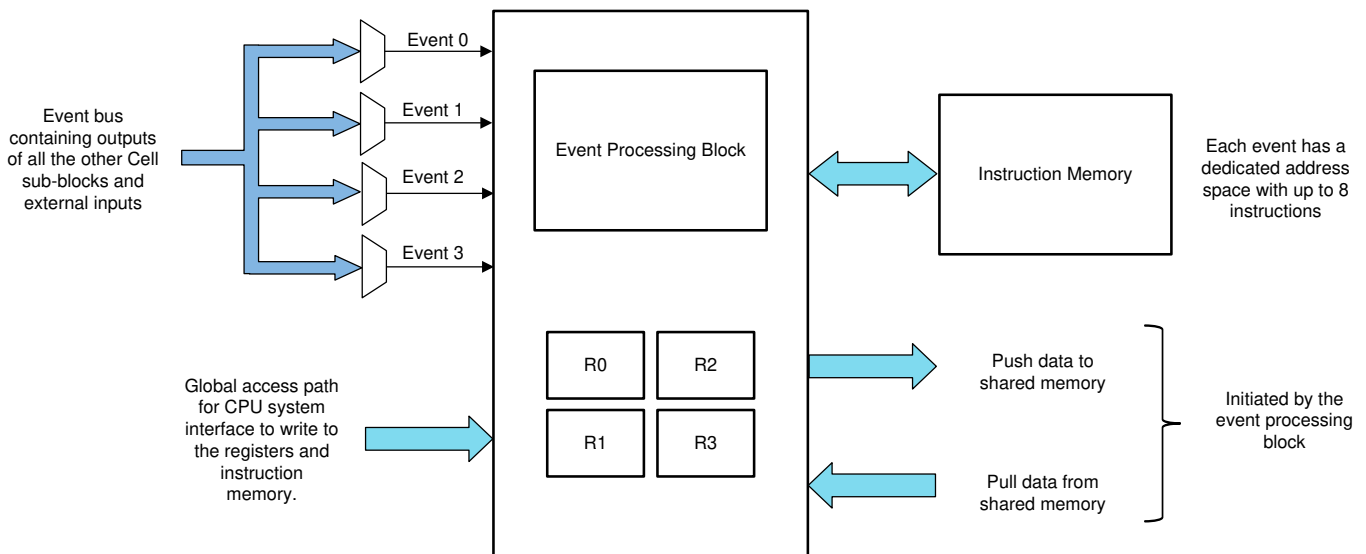
Figure 25-13. High Level Controller Block
