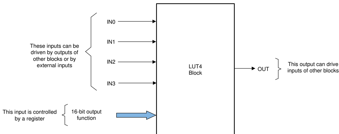
Figure 25-11. LUT4 Block
