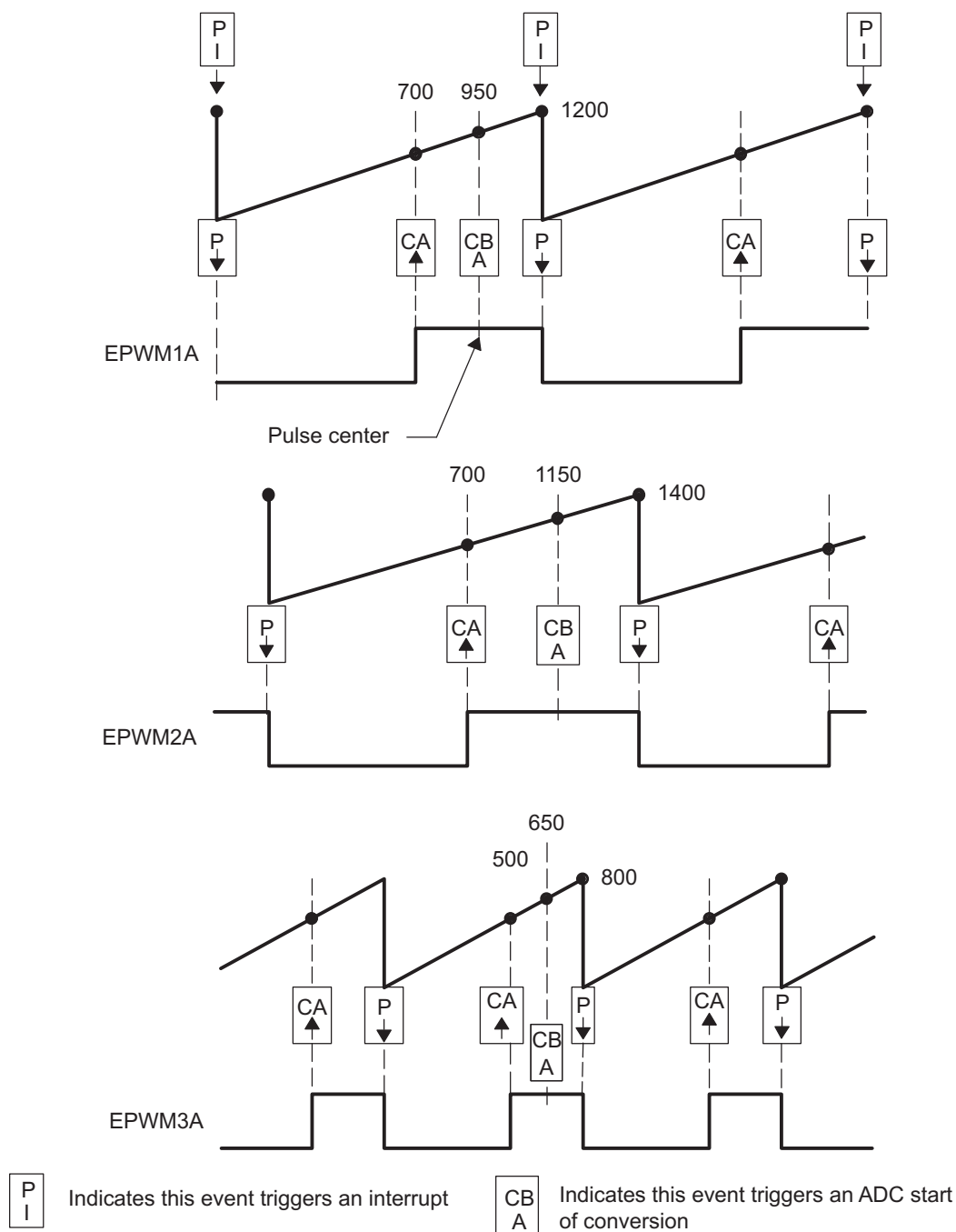
Figure 14-61. Buck Waveforms for Figure 14-60 (Note: Only three bucks shown here)
