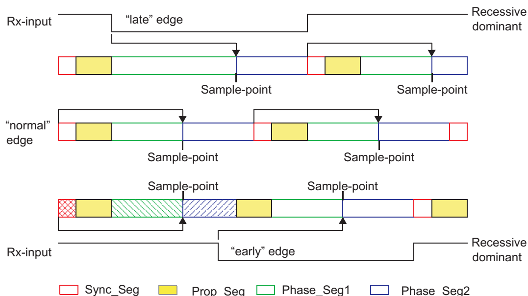
Figure 21-14. Synchronization on Late and Early Edges
