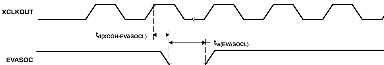
Figure 6–15. \overline{EVASOCL} Timing
