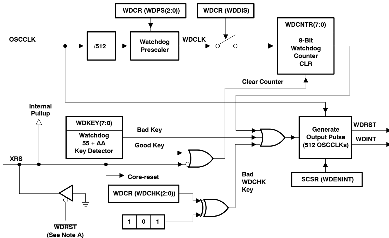
Figure 3–10. Watchdog Module
