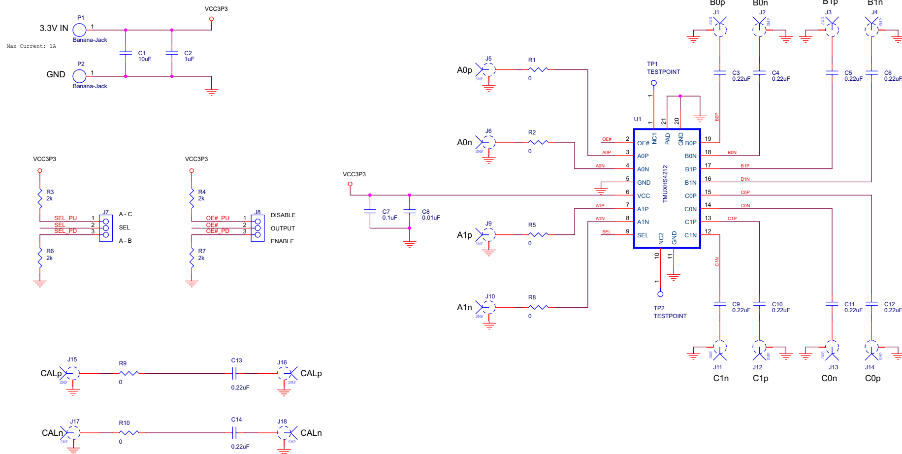
Figure 3. TMUXHS4212EVM Schematic
