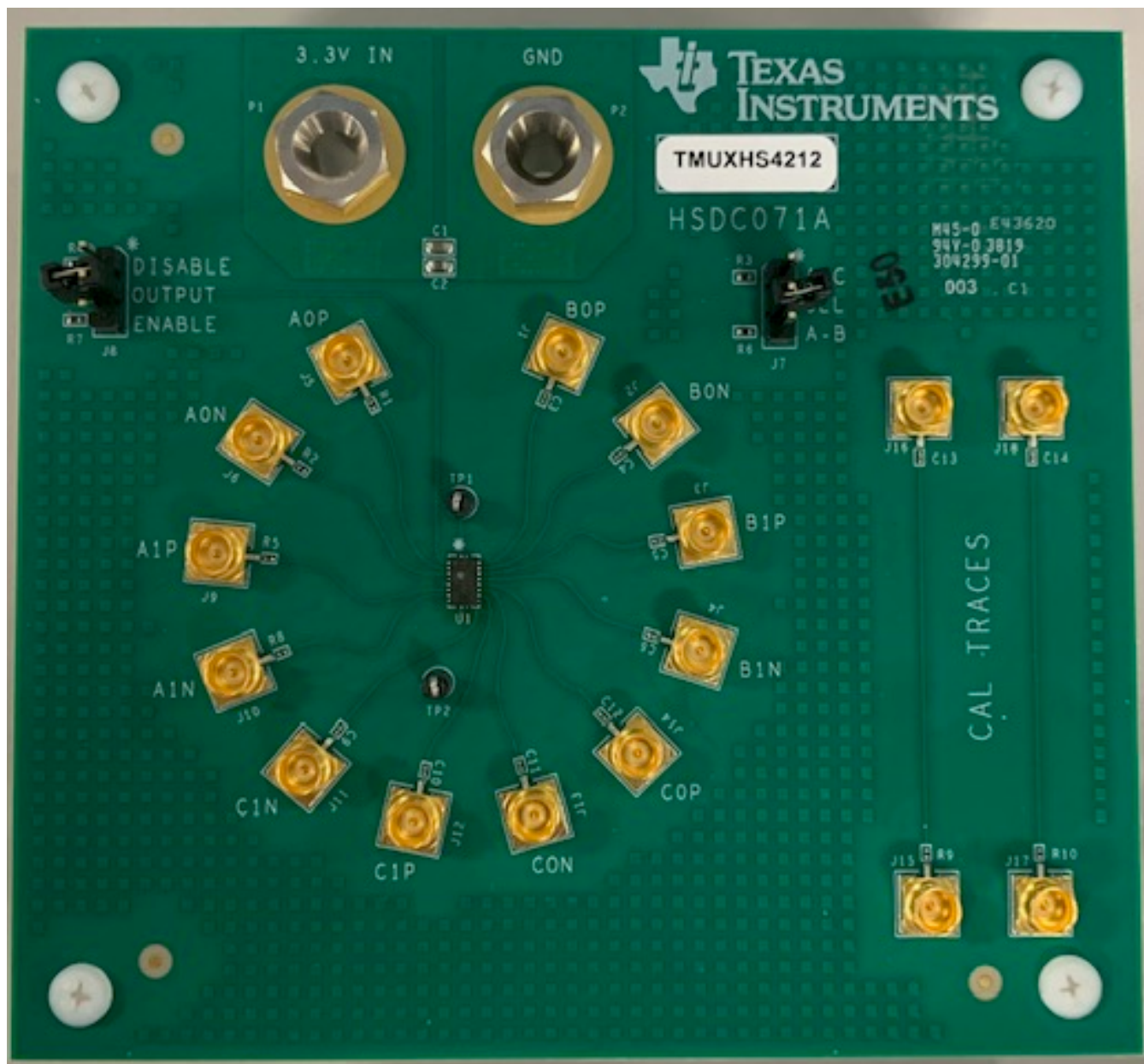
Figure 2. TMUXHS4212EVM
