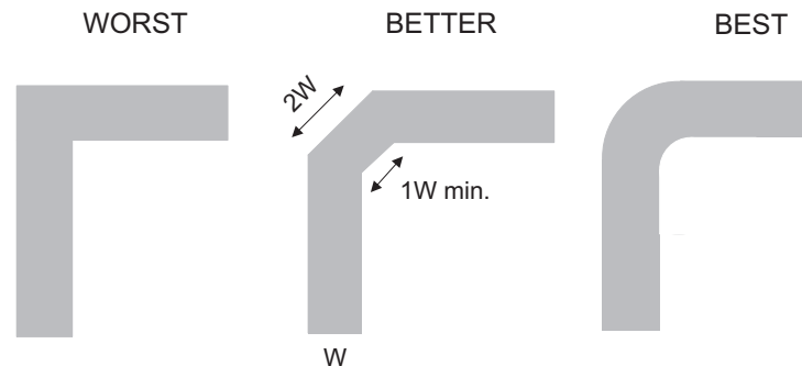
Figure 34. Trace Example
