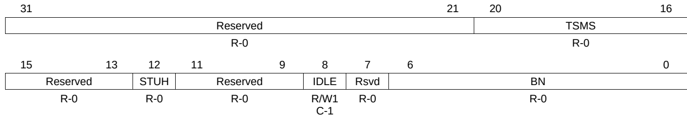
Figure 23-34. Transfer Status Current Buffer (TSCB) [offset_TU = 18h]
