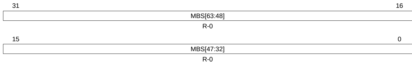
Figure 23-168. Message Buffer Status Changed Register 2 (MBSC2) [offset_CC = 344h]
