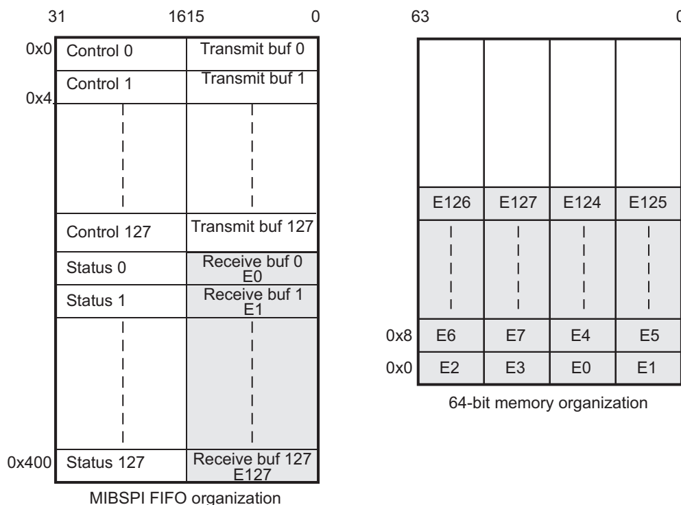
Figure 16-13. Example of DMA Data Packing
