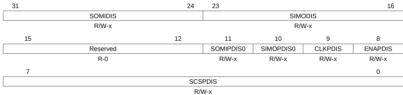
Figure 25-38. SPI Pin Control Register 7 (SPIPC7) [offset = 30h]
