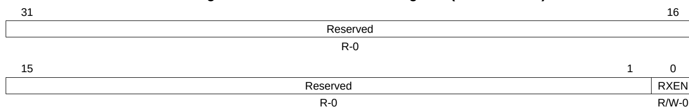
Figure 29-46. Receive Control Register (RXCONTROL)
