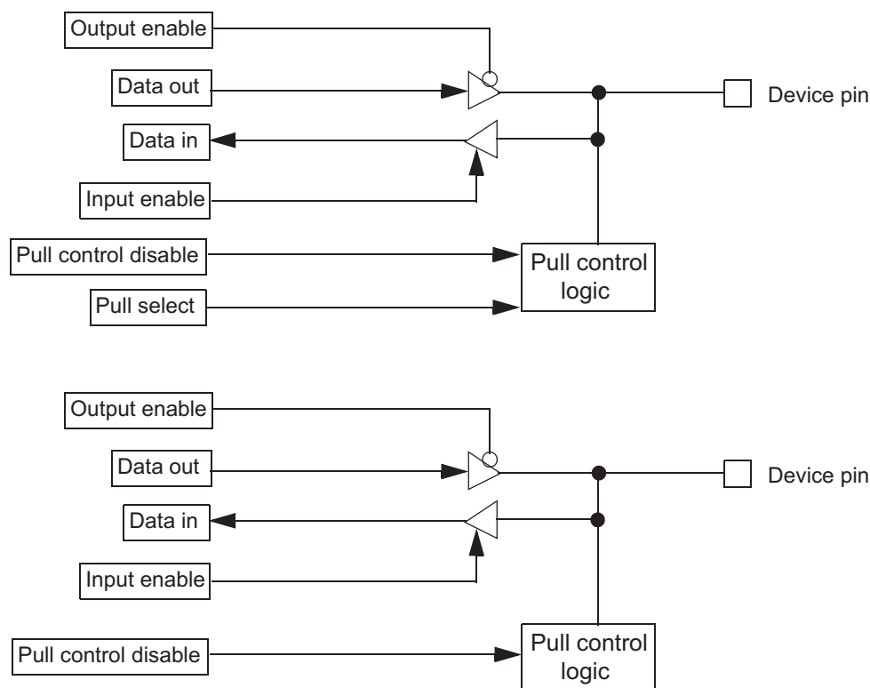
Figure 27-32. GPIO Functionality
