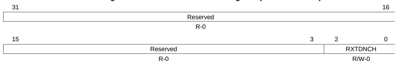
Figure 29-47. Receive Teardown Register (RXTEARDOWN)
