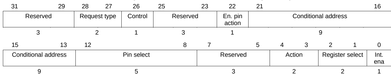
Figure 20-168. PWCNT Control Field (C31:C0)
