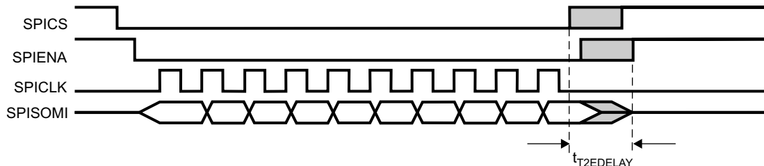
Figure 28-47. Transmit-Data-Finished-to-ENA-Inactive-Timeout
