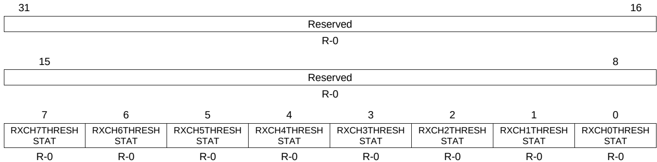
Figure 32-22. EMAC Control Module Receive Threshold Interrupt Status Register (C0RXTHRESHSTAT)
