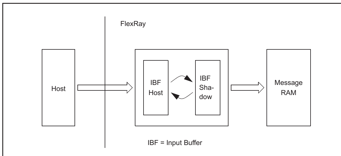
Figure 26-18. Double Buffer Structure Input Buffer
