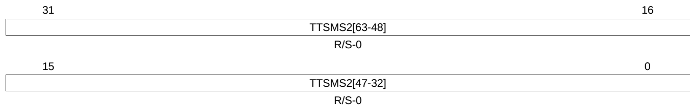
Figure 26-57. Trigger Transfer to System Memory Set 2 (TTSMS2) [offset_TU = 88h]
