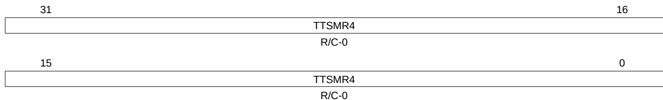
Figure 26-62. Trigger Transfer to System Memory Reset 4 (TTSMR4) [offset_TU = 9Ch]
