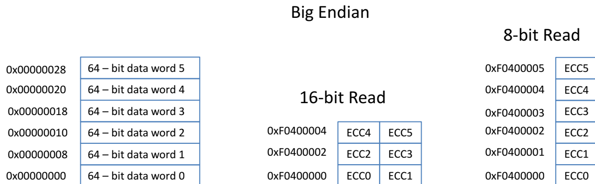
Figure 5-1. ECC Organization for Program Flash (144-Bits Wide)
