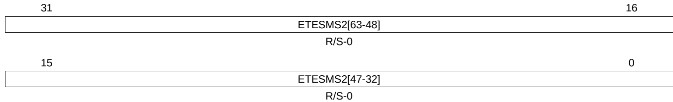
Figure 26-73. Enable Transfer on Event to System Memory Set 2 (ETESMS2) [offset_TU = C8h]
