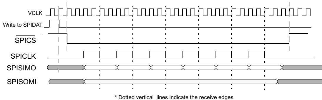
Figure 28-82. SPI/MibSPI Pins During Master Mode 4-pin with \overline{\text{SPIC}}\text{S} Configuration
