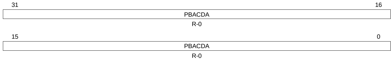
Figure 16-66. Port B Active Channel Destination Address Register (PBACDAADDR) [offset = 19Ch]
