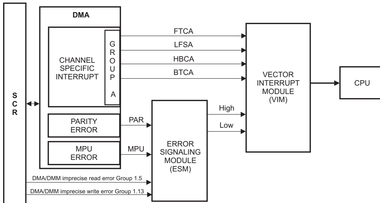
Figure 16-14. DMA Interrupts
