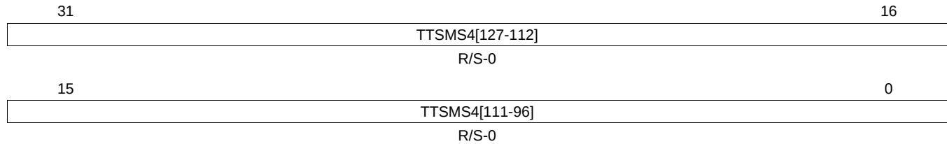
Figure 26-61. Trigger Transfer to System Memory Set 4 (TTSMS4) [offset_TU = 98h]
