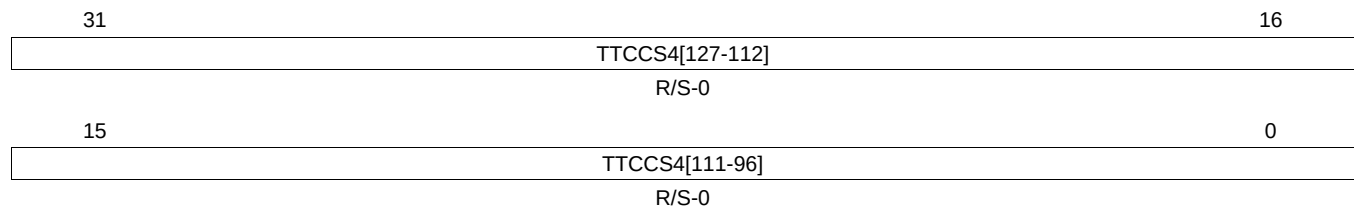
Figure 26-69. Trigger Transfer to Communication Controller Set 4 (TTCCS4) [offset_TU = B8h]
