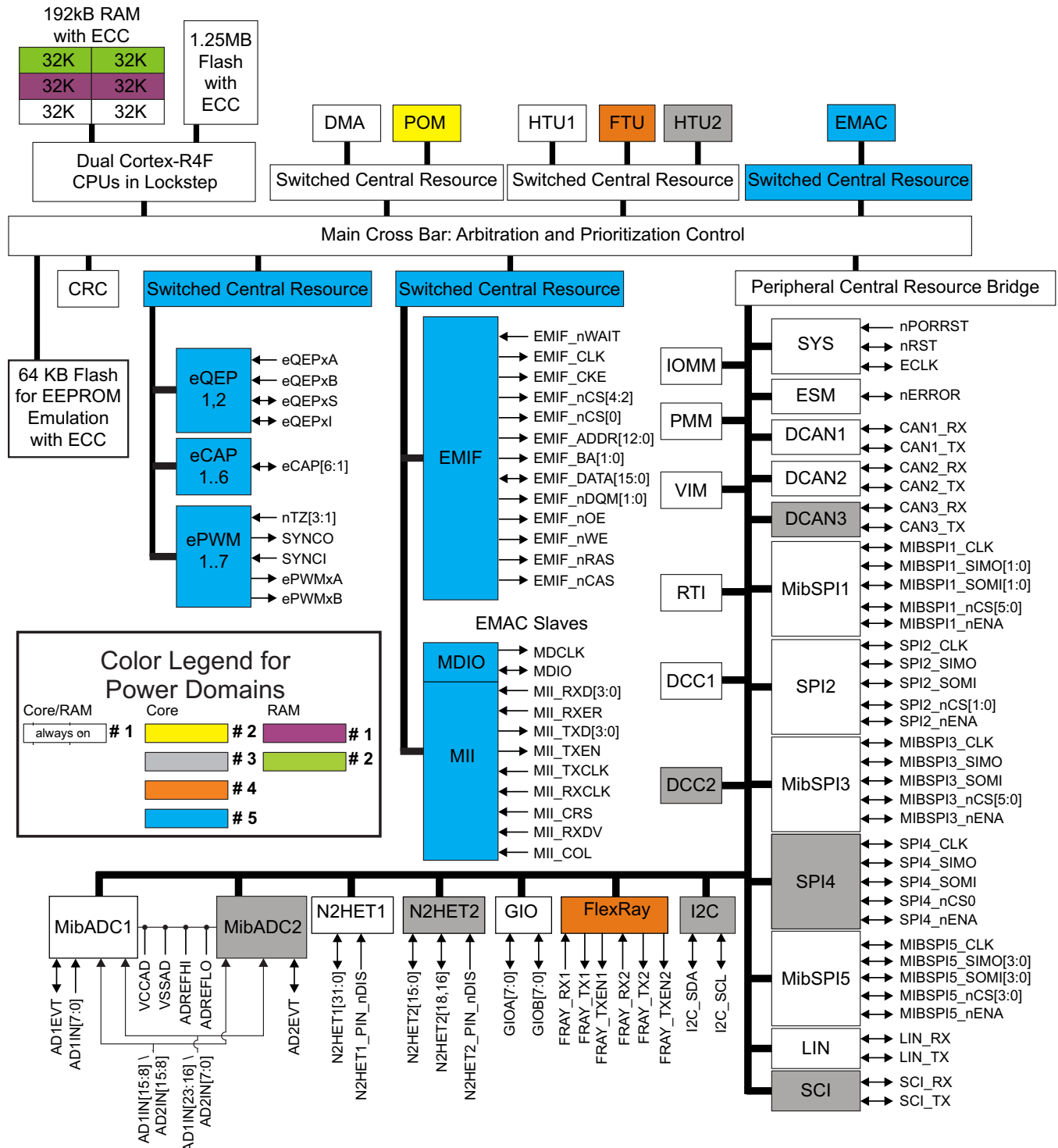
Figure 1-1. Block Diagram
