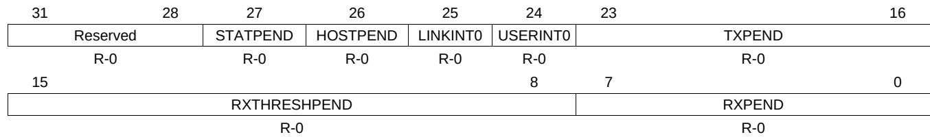
Figure 32-52. MAC Input Vector Register (MACINVECTOR)
