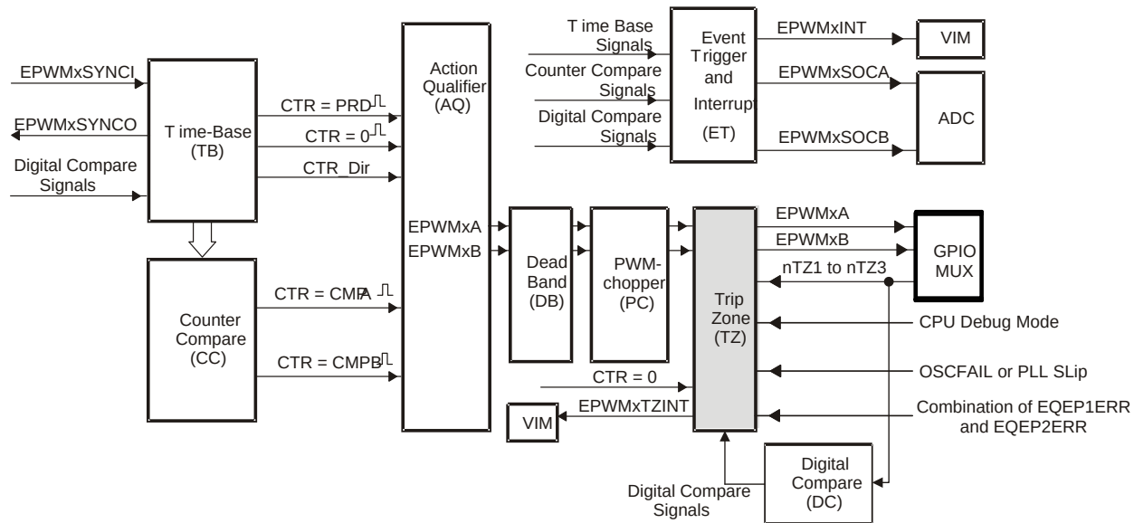
Figure 19-35. Trip-Zone Submodule
