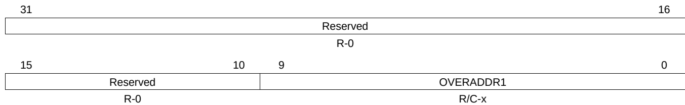
Figure 28-70. RXRAM Uncorrectable Parity Error Address Register (UERRADDR1) [offset = 128h]
