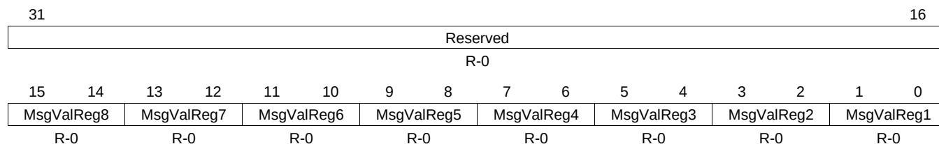
Figure 27-43. Message Valid X Register (DCAN MSGVAL X) [offset = C0h]
