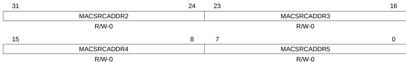
Figure 32-77. MAC Source Address High Bytes Register (MACSRCADDRHI)
