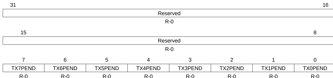
Figure 32-49. Transmit Interrupt Status (Masked) Register (TXINTSTATMASKED)
