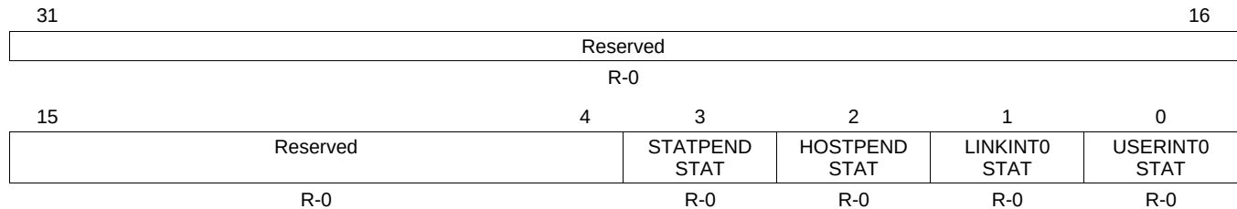
Figure 32-25. EMAC Control Module Miscellaneous Interrupt Status Register (C0MISCSTAT)
