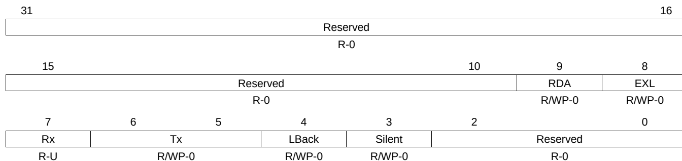
Figure 27-24. Test Register (DCAN TEST) [offset = 14h]
