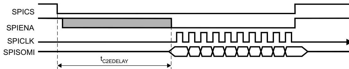
Figure 28-48. Chip-Select-Active-to-ENA-Signal-Active-Timeout
