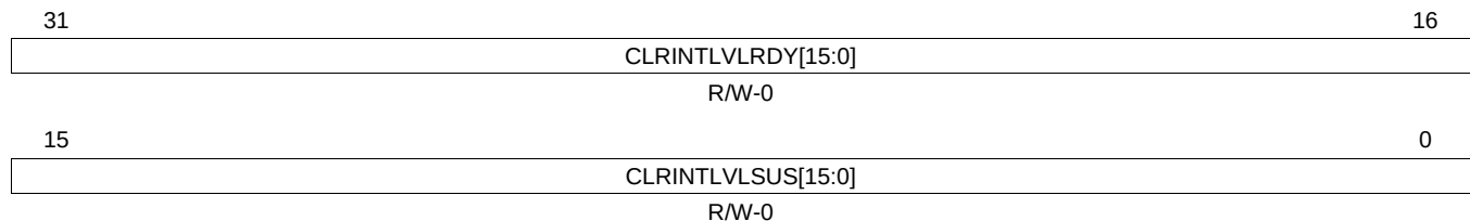
Figure 28-59. Transfer Group Interrupt Level Clear Register (TGITLVCR) [offset = 80h]
