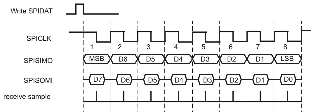
Figure 28-11. Clock Mode with Polarity = 1 and Phase = 1
