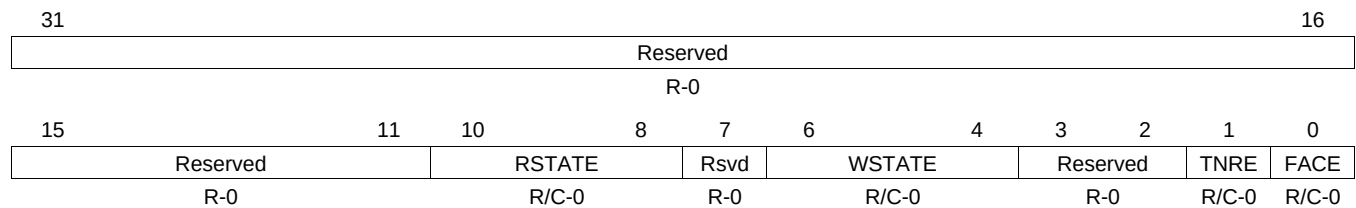
Figure 26-54. Transfer Error Interrupt Enable Reset (TEIRER) [offset_TU = 7Ch]
