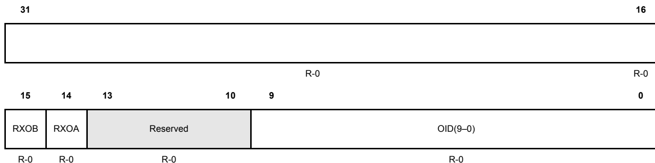
Figure 17-148. Odd Sync ID Register [1...15] (OSIDn) [offset CC = 0x170–0x1A8]
