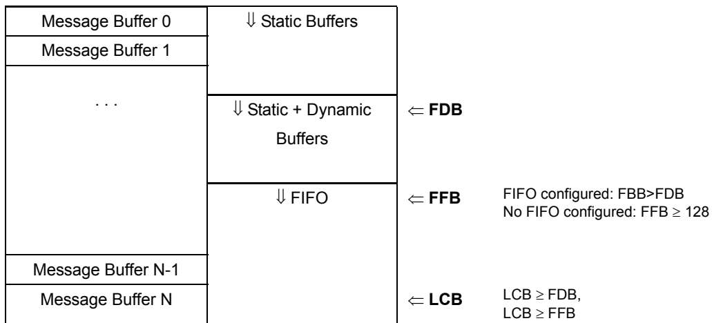
Figure 17-151. Buffer Configuration
