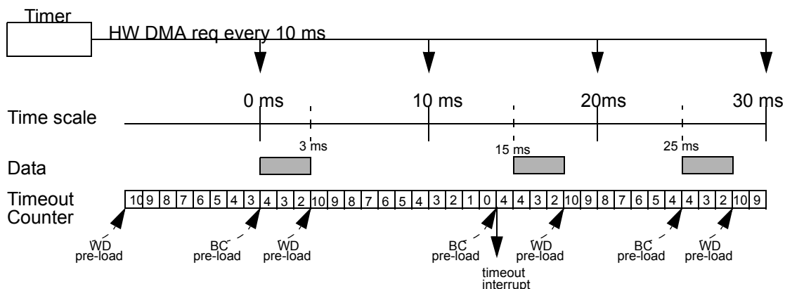
Figure 22-8. Timeout Example 3
