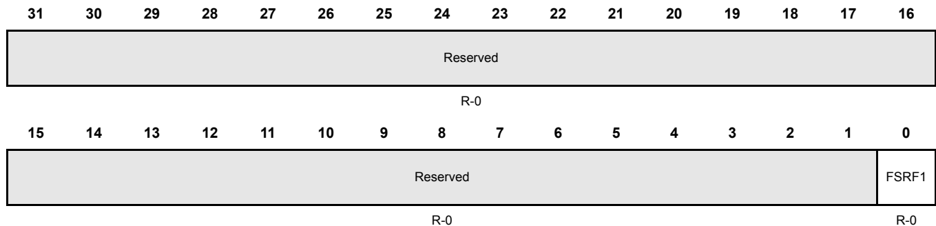
Figure 6-20. Fail Status Fail Register 1 (FSRF1) [offset = 0x0194]
