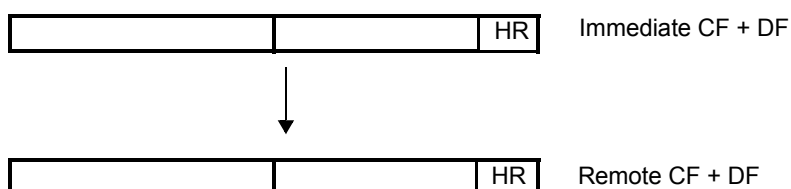
Figure 18-121. MOV64 Move Operation
