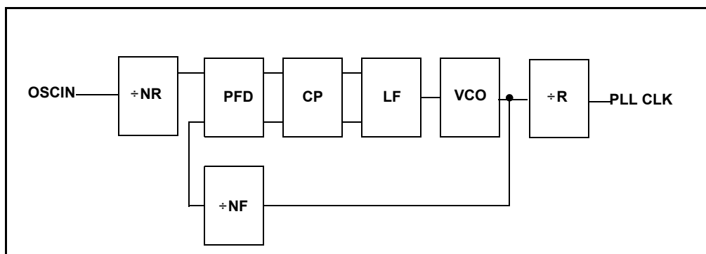
Figure 7-12. Basic PLL Circuit
