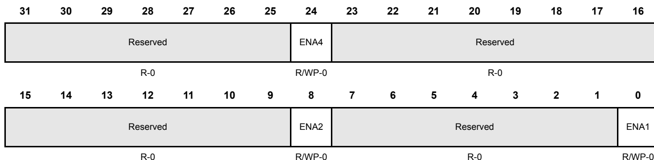
Figure 27-10. RTP Trace Enable Register (RTPTRENA) [offset = 04h]
