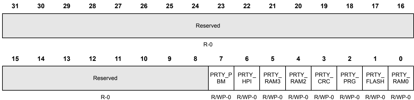
Figure 5-40. Bus Matrix Module Control Register2 (BMMCR2) [offset = 0xC8]
