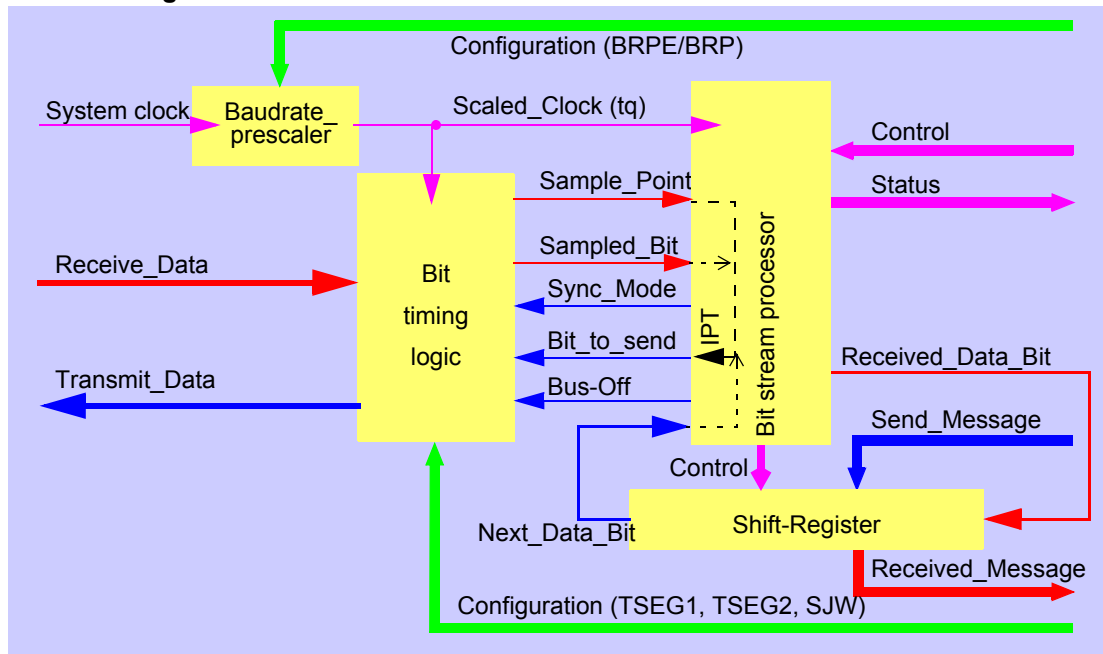
Figure 16-19. Structure of the CAN Core's CAN Protocol Controller
