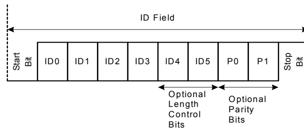
Figure 13-16. ID Field
