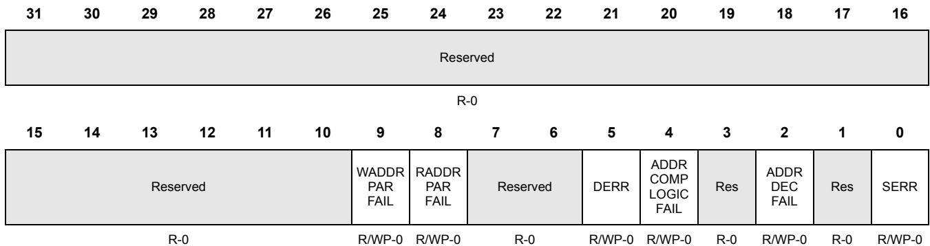
Figure 4-7. TCRAM Wrapper Error Status Register (RAMERRSTATUS) [offset = 0x10]
