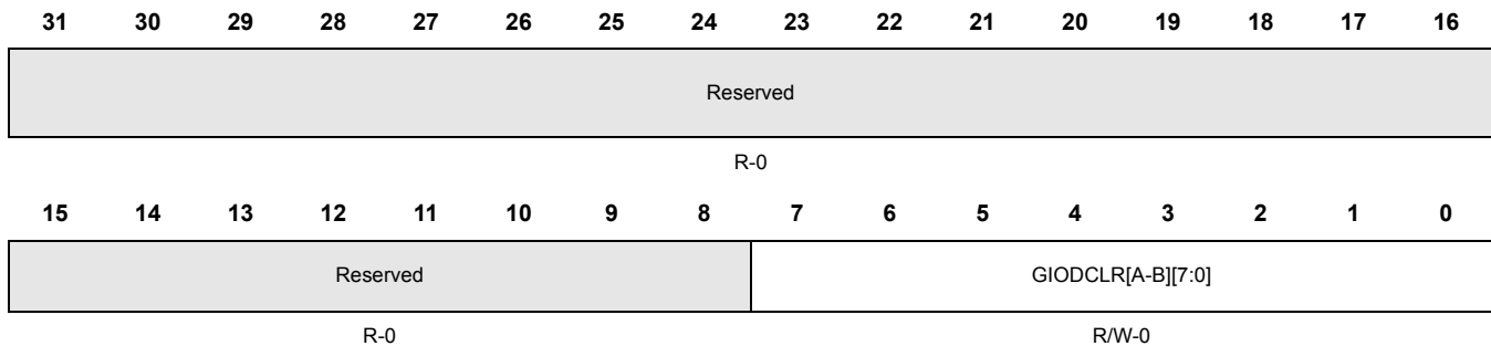
Figure 12-27. GIO Data Clear Registers [A-B][7:0] (GIODCLR[A-B][7:0])[0xFFFF7BC44, 0xFFFF7BC64]
