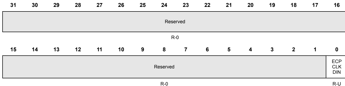
Figure 5-4. SYS Pin Control Register 3 (SYSPC3) [offset = 0x08]
