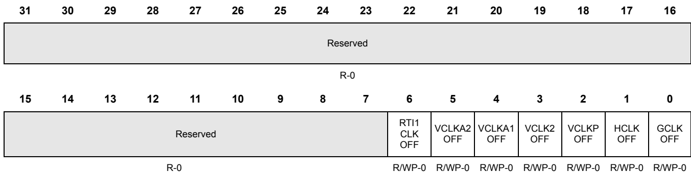
Figure 5-14. Clock Domain Disable Register (CDDIS) [offset = 0x3C]
