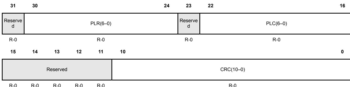
Figure 17-181. Read Header Section Register 2 (RDHS2) [offset_CC = 0x704]
