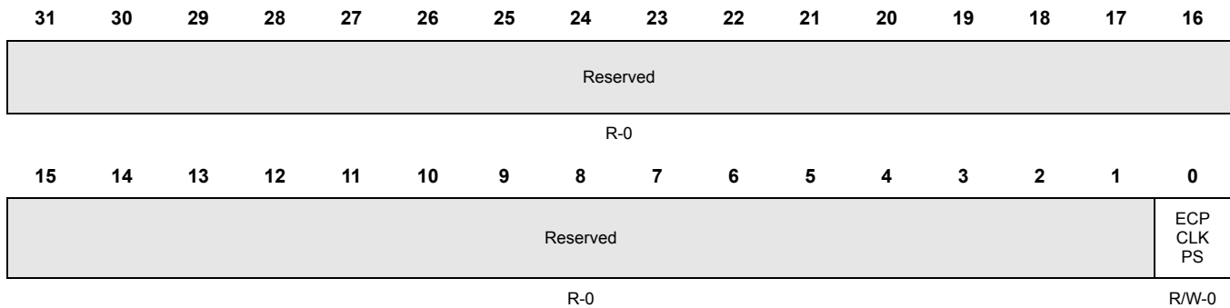
Figure 5-10. SYS Pin Control Register 9 (SYSPC9) [offset = 0x20]
