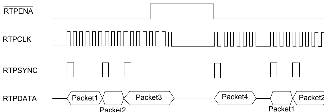
Figure 27-7. RTP Packet Transfer with Sync Signal
