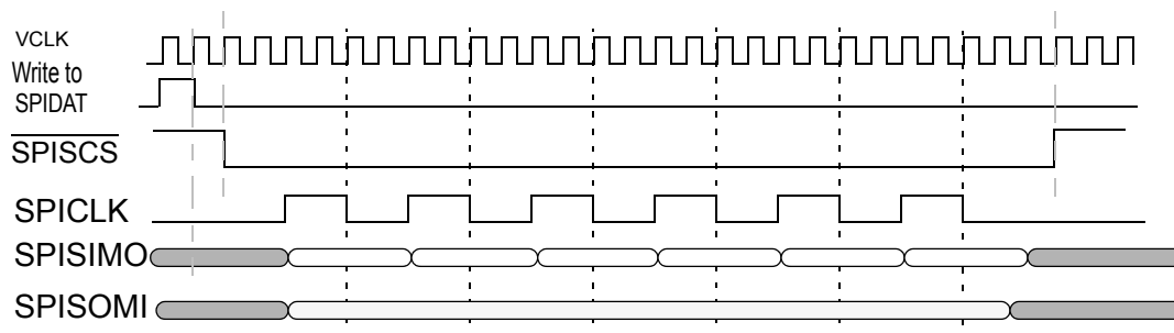
Figure 14-54. SPI/MibSPI pins during Master mode 4-pin with \overline{\text{SPISCS}} configuration.
