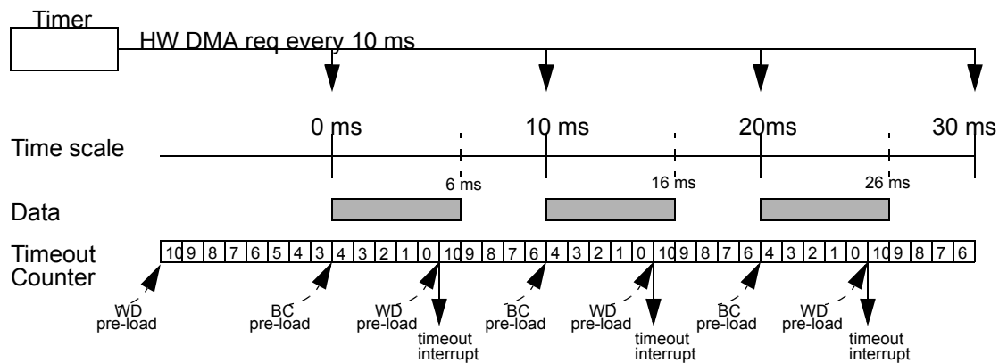
Figure 22-7. Timeout Example 2
