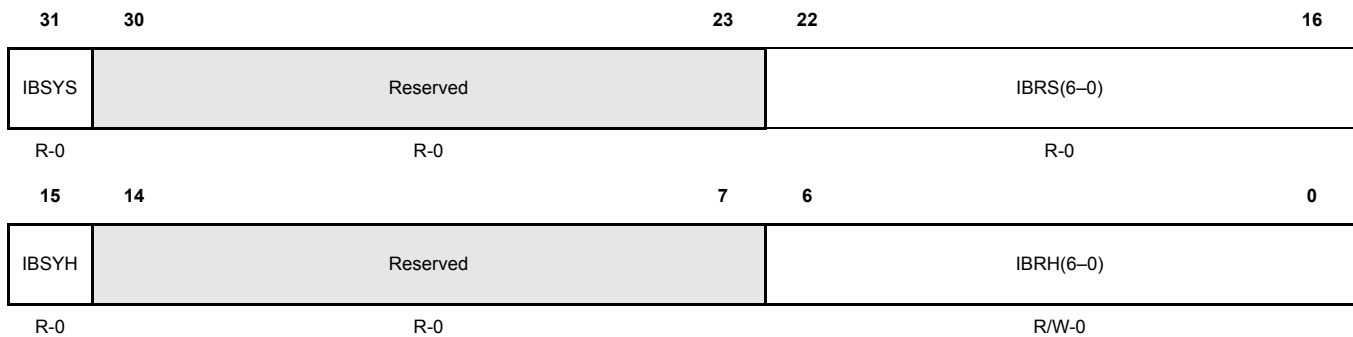
Figure 17-178. Input Buffer Command Request Register (IBCR) [offset_CC = 0x514]
