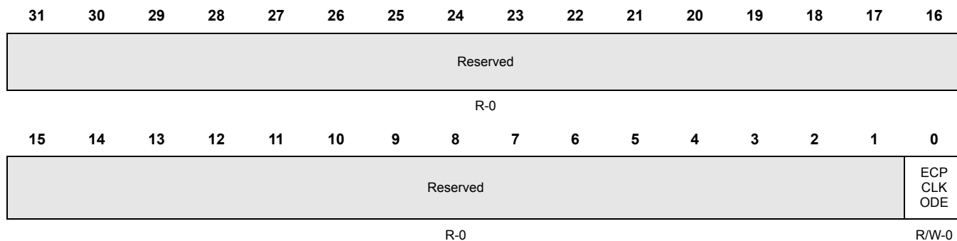
Figure 5-8. SYS Pin Control Register 7 (SYSPC7) [offset = 0x18]
