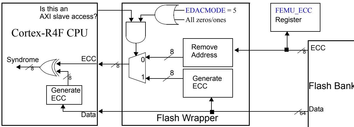
Figure 8-3. Cortex-R4F Flash ECC Read Path
