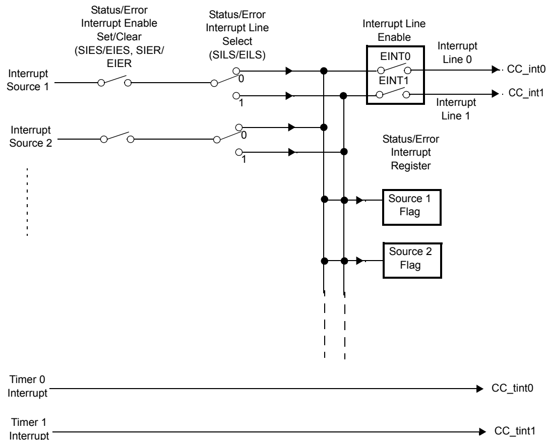
Figure 17-26. Interrupt Structure
