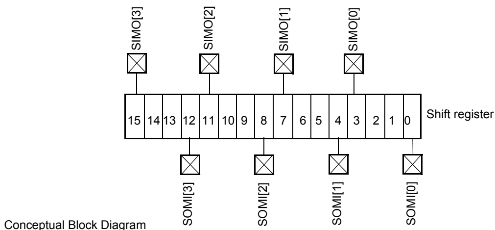
Figure 14-19. 4-Data Line Mode (Phase 0, Polarity 0)
