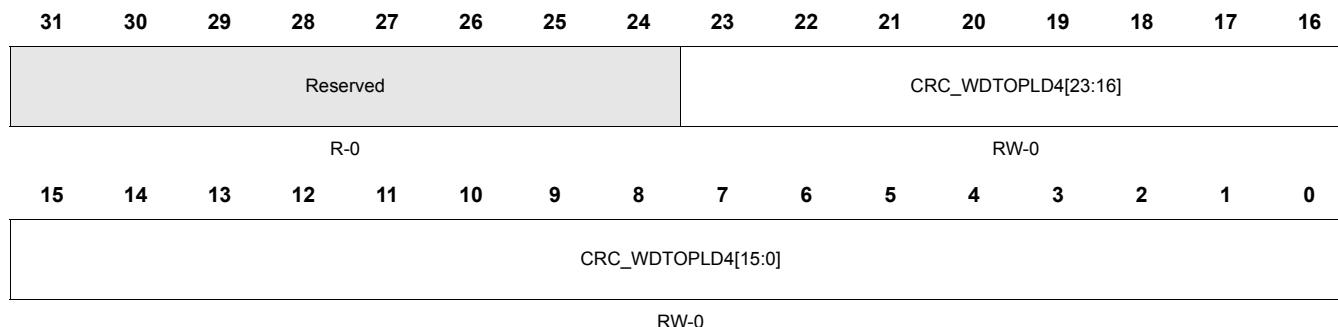
Figure 22-60. CRC Channel 4 Watchdog Timeout Preload Register A(CRC_WDTPLD4) [offset = 0x10C]
