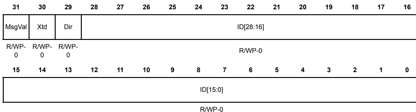
Figure 16-47. IF2 Arbitration Register (DCAN IF2ARB) [offset = 0x128]
