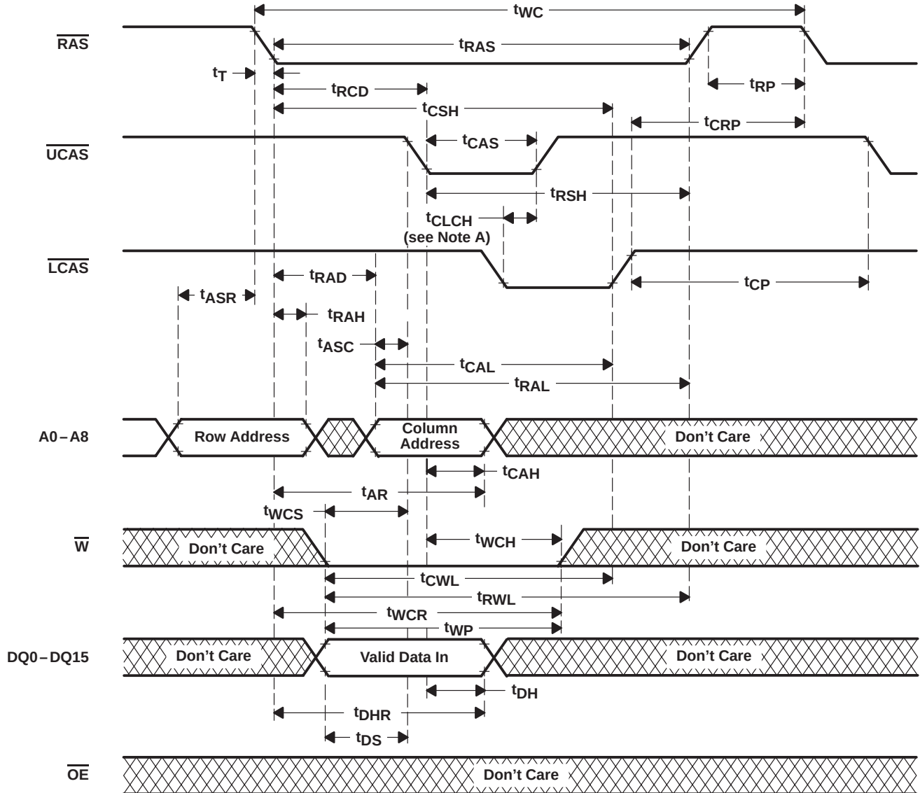
Figure 4. Early-Write-Cycle Timing
