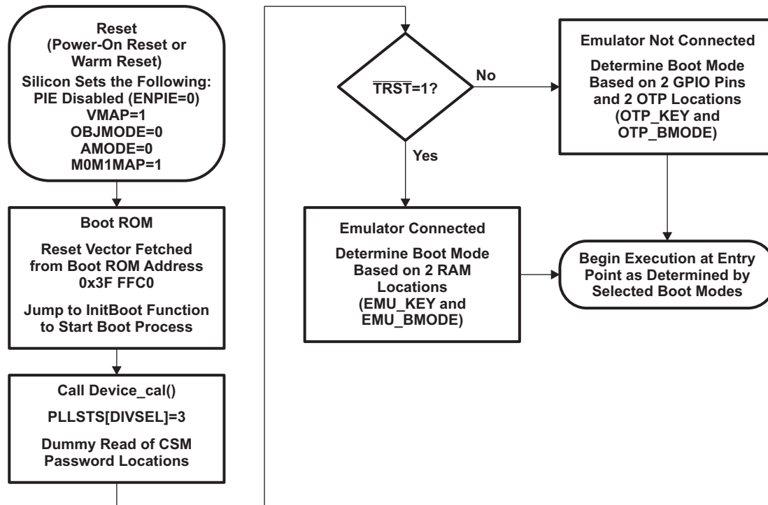
Figure 2-4. Bootloader Flow Diagram
