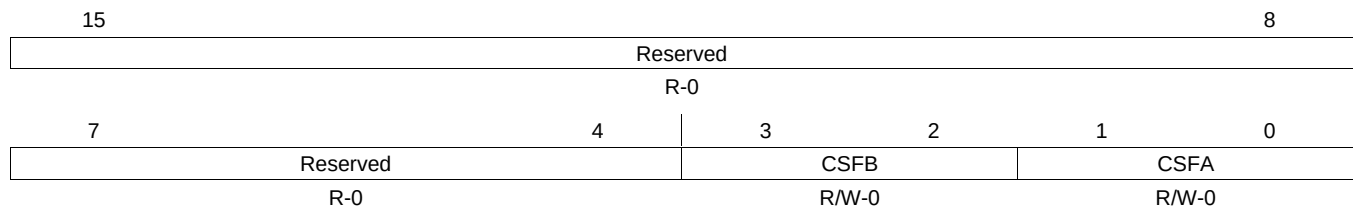
Figure 3-92. Action-Qualifier Continuous Software Force Register (AQCSFRC)
