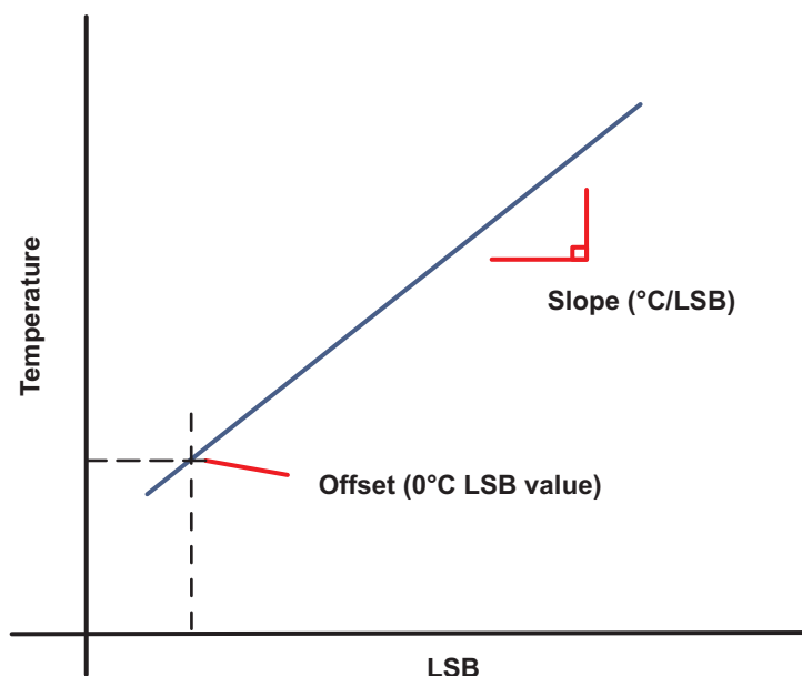
Figure 8-38. Temperature Sensor Transfer Function
