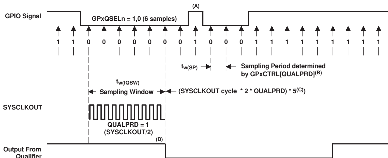
Figure 1-64. Input Qualifier Clock Cycles
