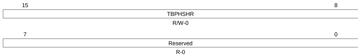
Figure 3-77. Time-Base Phase High Resolution Register (TBPHSHR)
