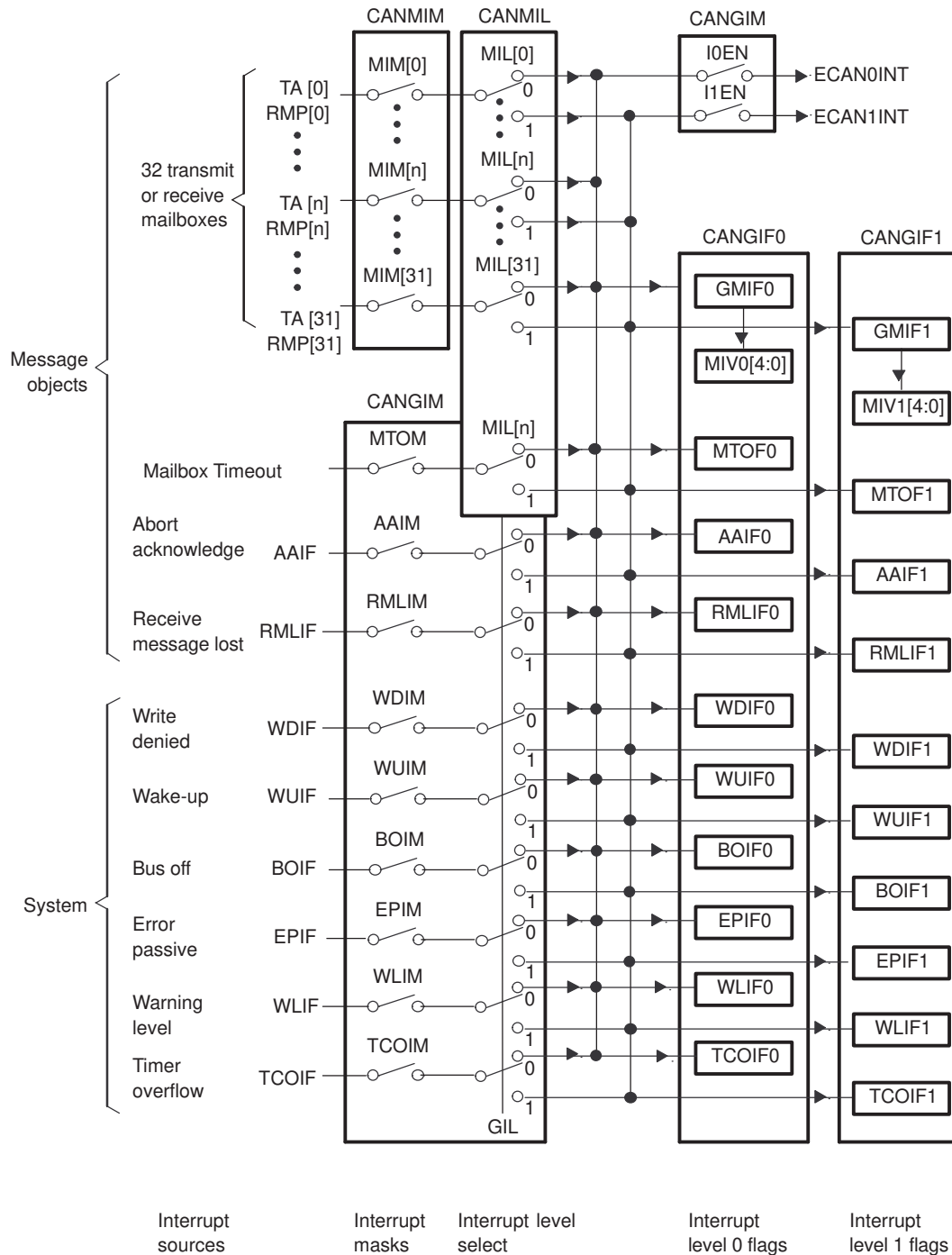
Figure 16-7. Interrupts Scheme
