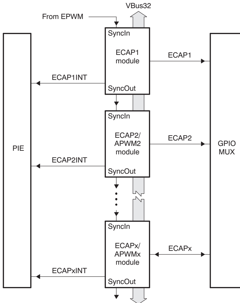
Figure 6-1. Multiple eCAP Modules In A C28x System
