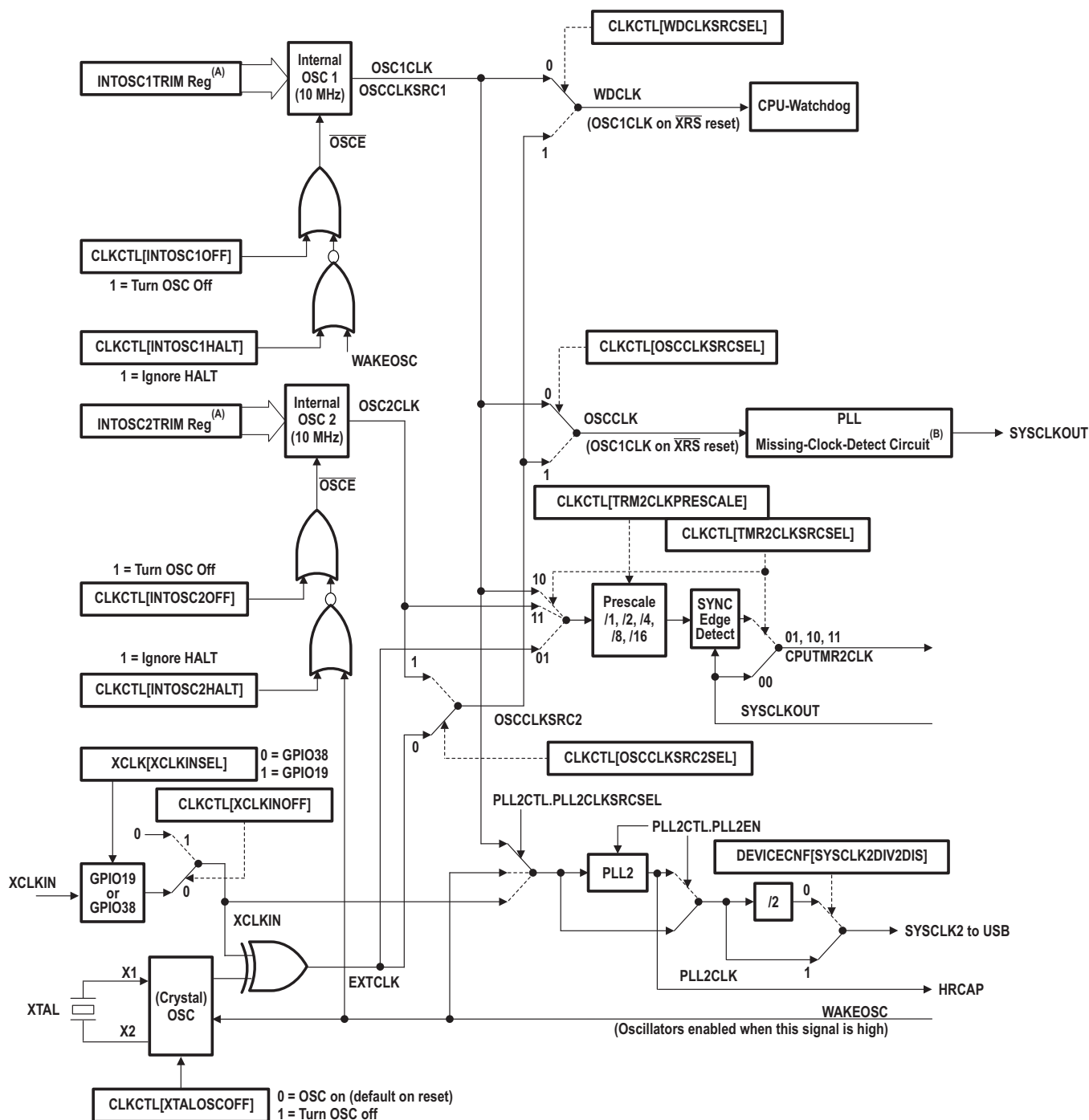
Figure 1-19. Clocking Options
