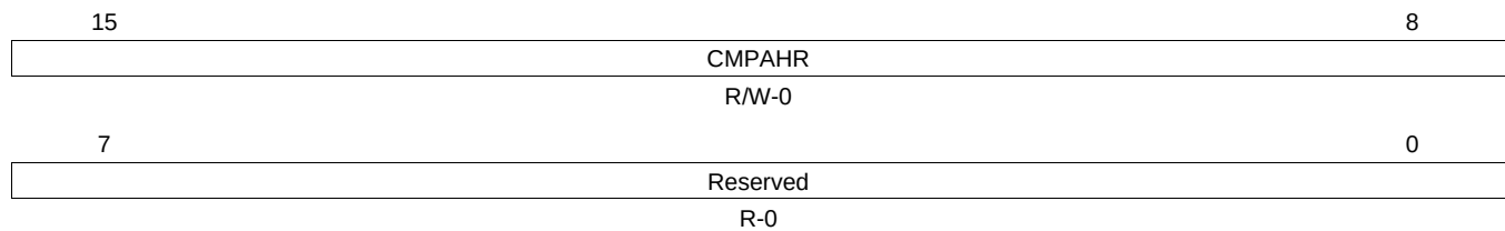
Figure 3-86. Compare A High Resolution Register (CMPAHR)
