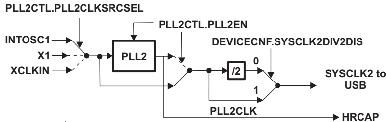
Figure 1-29. PLL2 Configuration (PLL2CTL) Register (EALLOW protected)
