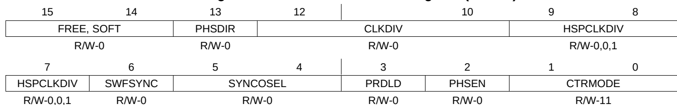
Figure 3-79. Time-Base Control Register (TBCTL)
