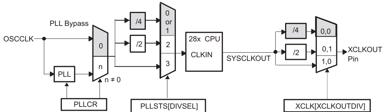
Figure 1-42. XCLKOUT Generation
