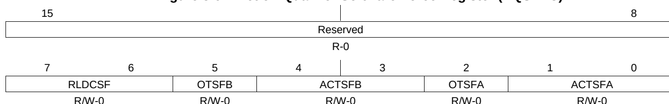
Figure 3-91. Action-Qualifier Software Force Register (AQSFRC)
