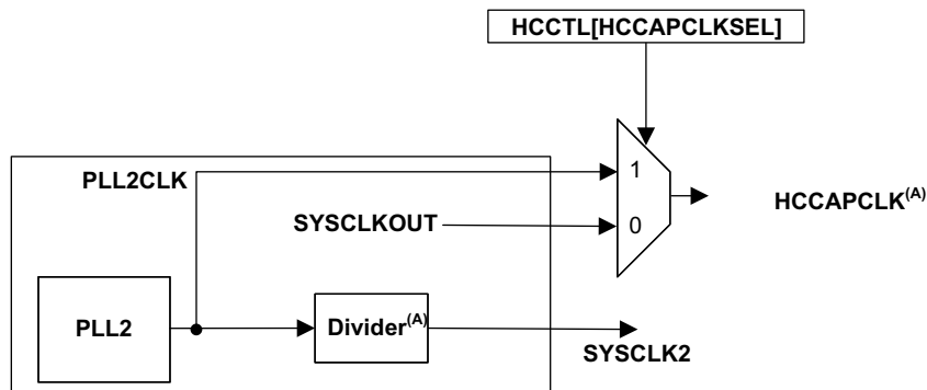
Figure 5-3. HCCAPCLK Generation
