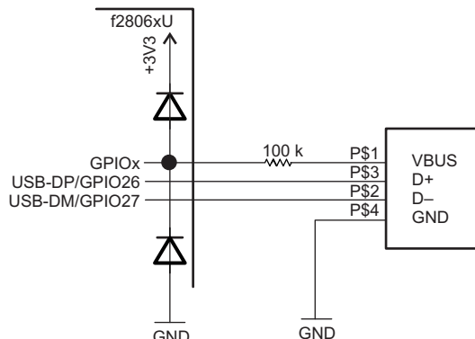
Figure 17-2. USB Scheme
