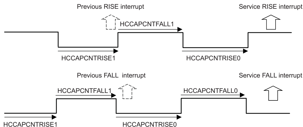
Figure 5-5. Rise vs. Fall Capture Events
