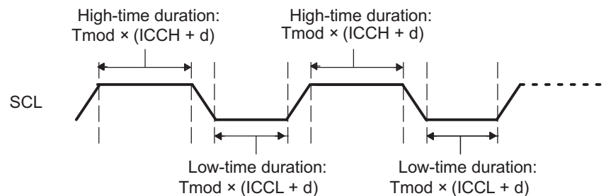
Figure 14-4. The Roles of the Clock Divide-Down Values (ICCL and ICCH)
