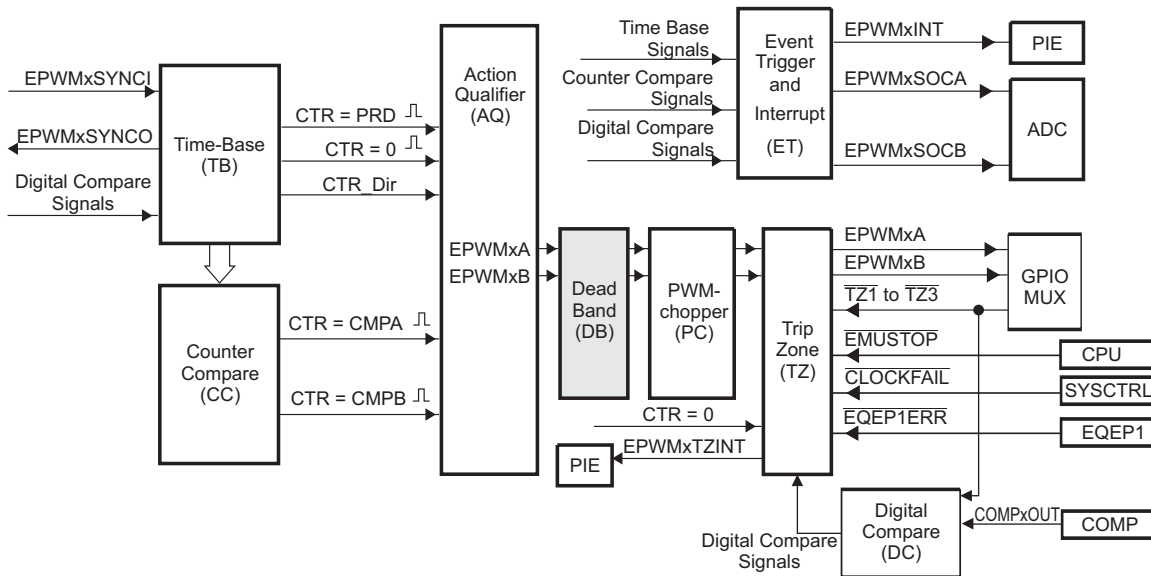
Figure 3-28. Dead-Band Submodule
