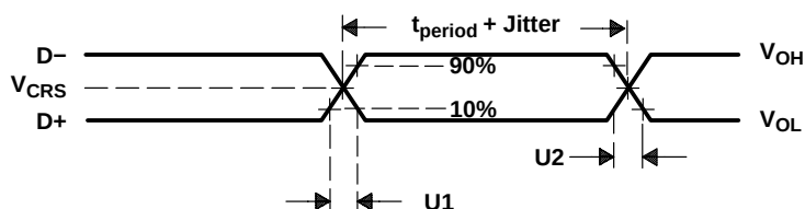
Figure 5–39. USB Timings
