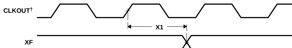
Figure 5–19. XF Timings
