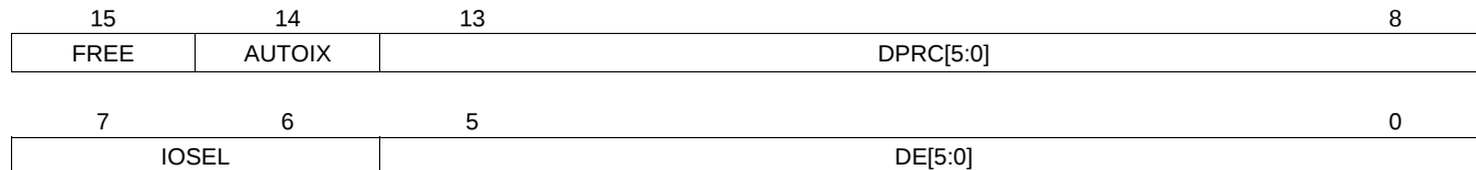
Figure 3-19. DMPREC Register
