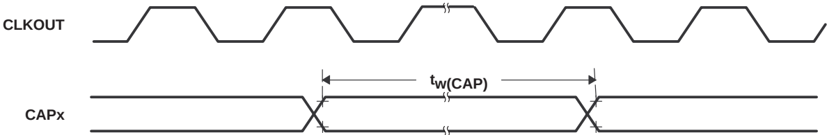
Figure 37. Capture Input and QEP Timing
