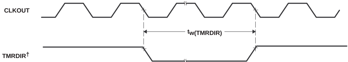
Figure 36. TMRDIR Timing
