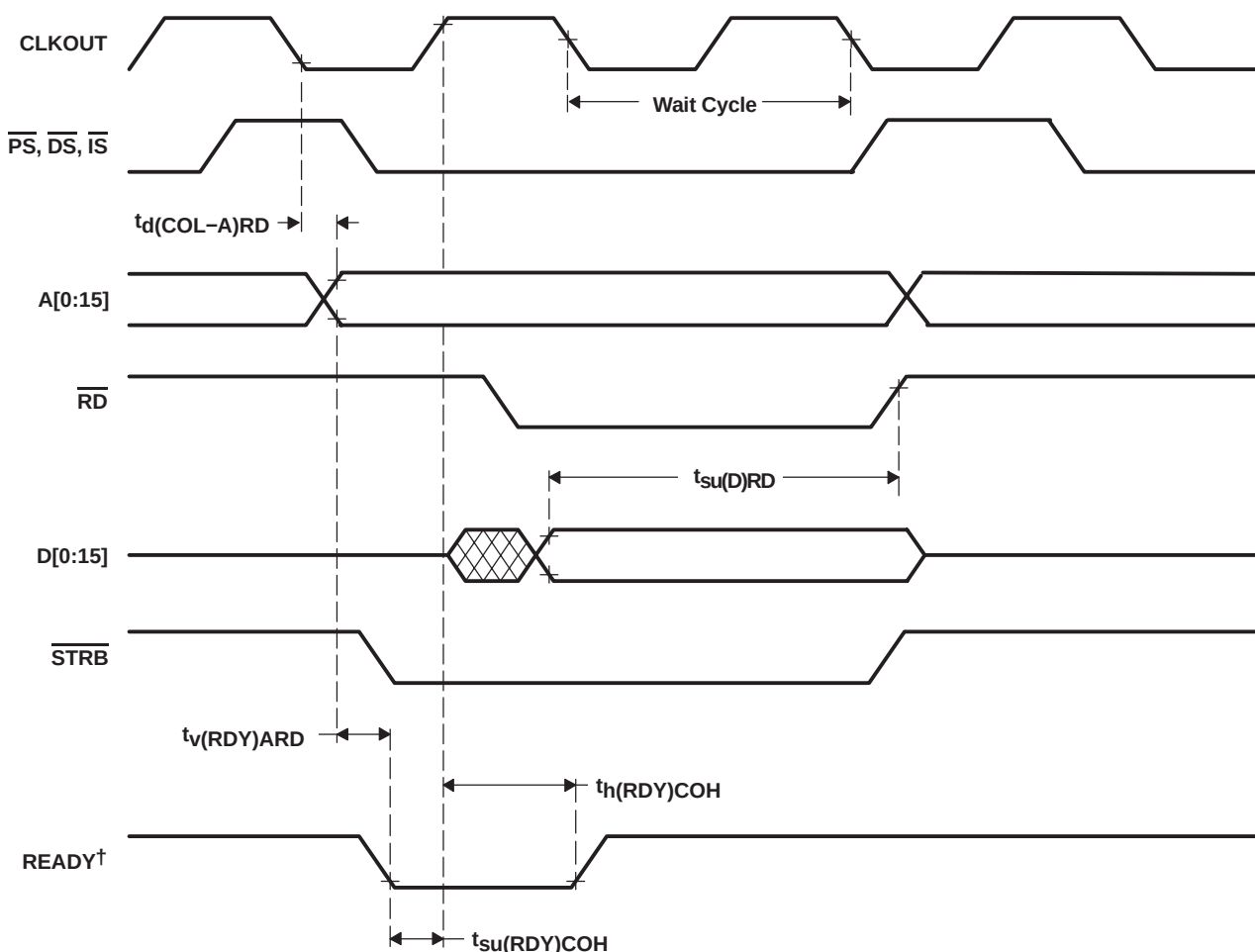
Figure 47. Ready-on-Read Timings
