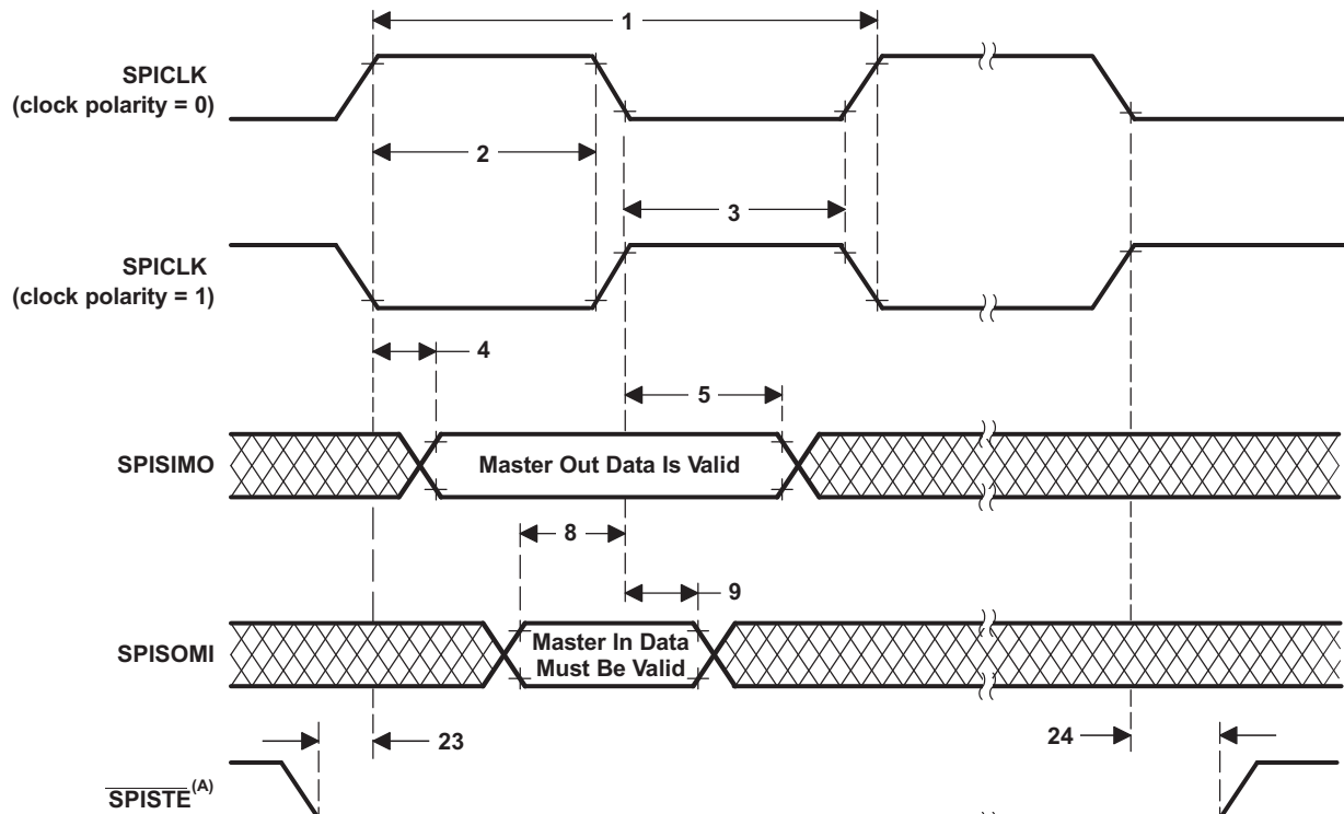
Figure 5-72. SPI Master Mode External Timing (Clock Phase = 0)
