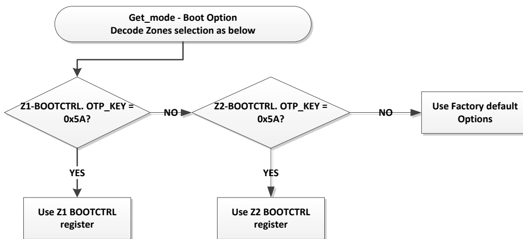
Figure 4-1. Z1 and Z2 BOOTCTRL Selection
