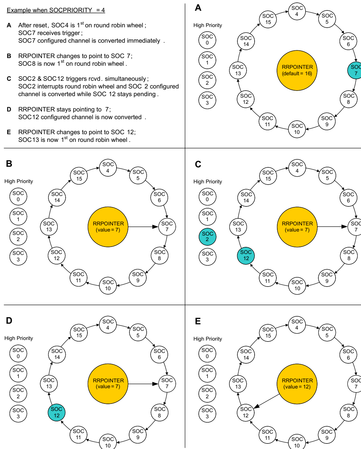
Figure 11-6. High Priority Example
