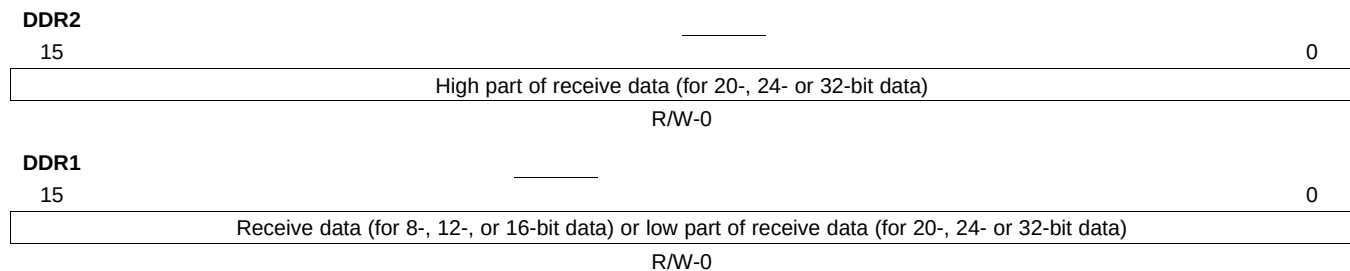
Figure 21-67. Data Receive Registers (DDR2 and DDR1)
