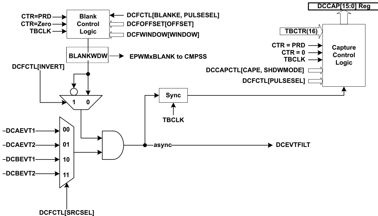
Figure 15-54. Event Filtering
