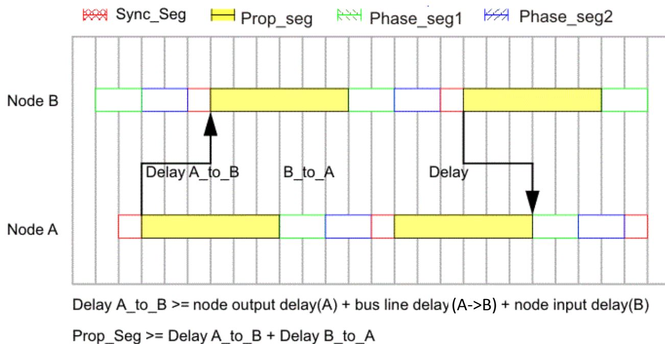
Figure 22-14. The Propagation Time Segment
