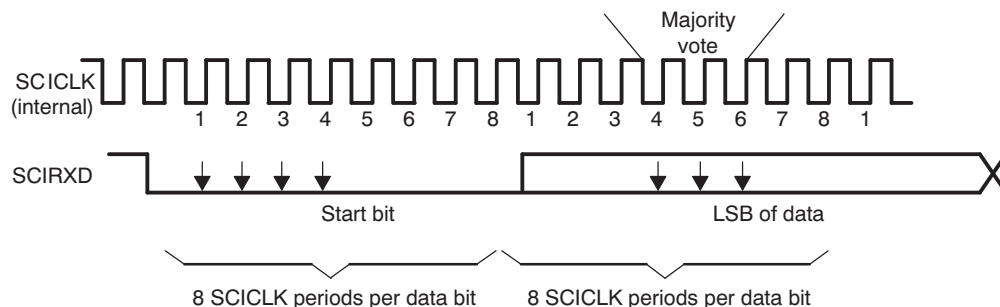
Figure 19-7. SCI Asynchronous Communications Format
