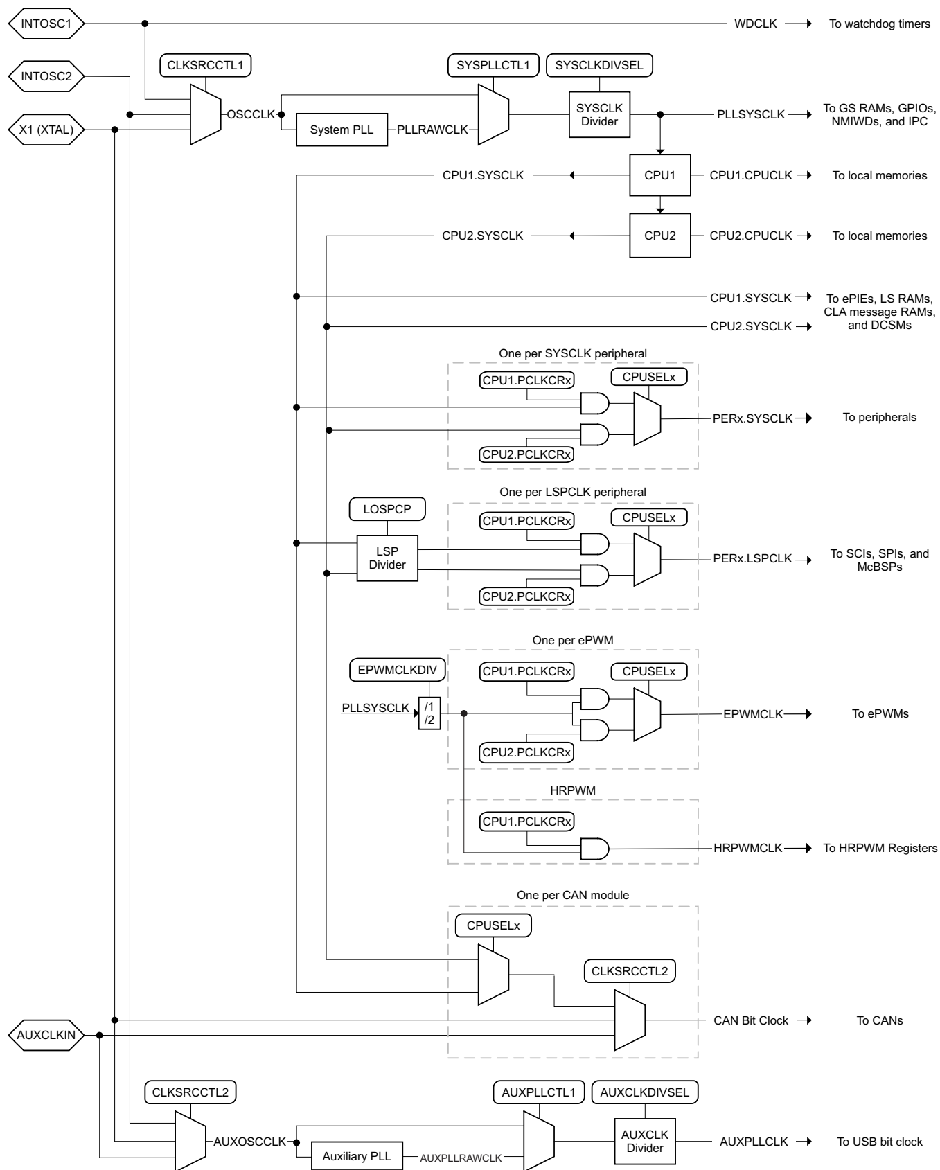
Figure 3-5. Clocking System
