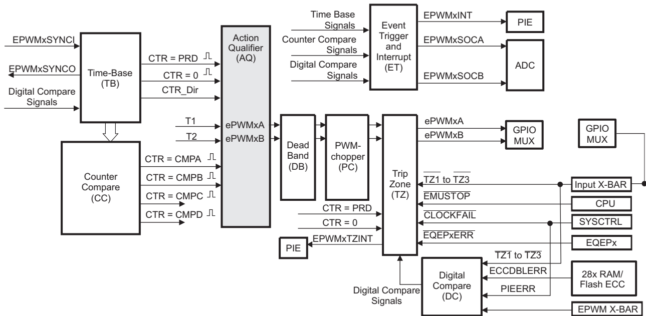
Figure 15-19. Action-Qualifier Submodule
