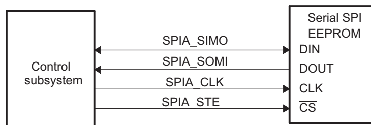
Figure 4-10. SPI Loader
