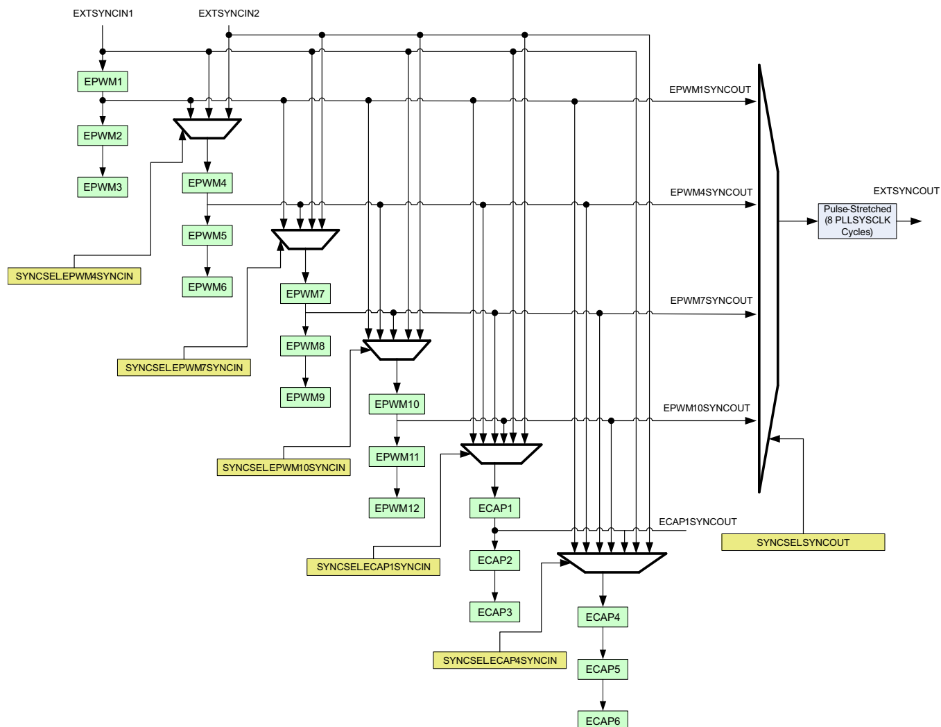
Figure 16-8. Time-Base Counter Synchronization Scheme
