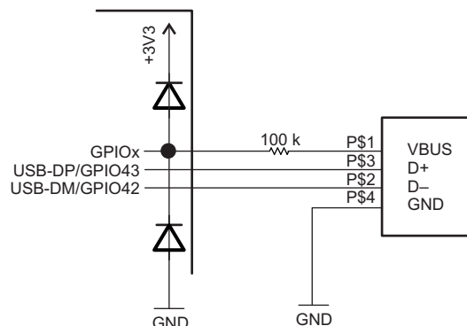
Figure 23-2. USB Scheme
