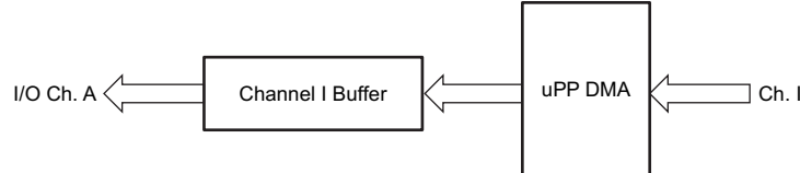
Figure 24-5. TX in SDR (non-interleave) or DDR (non-demux) Mode
