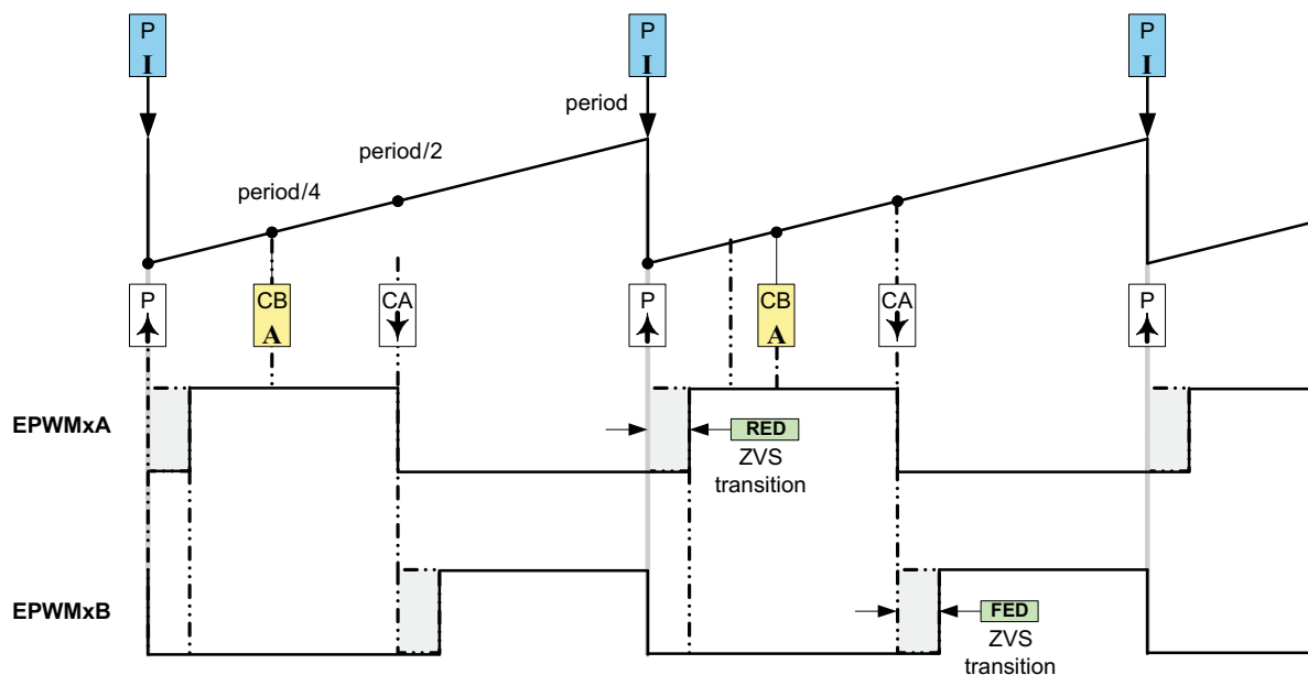
Figure 15-77. H-Bridge LLC Resonant Converter PWM Waveforms
