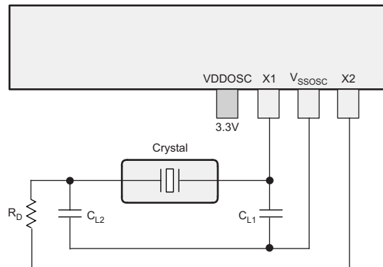
Figure 3-7. External Crystal
