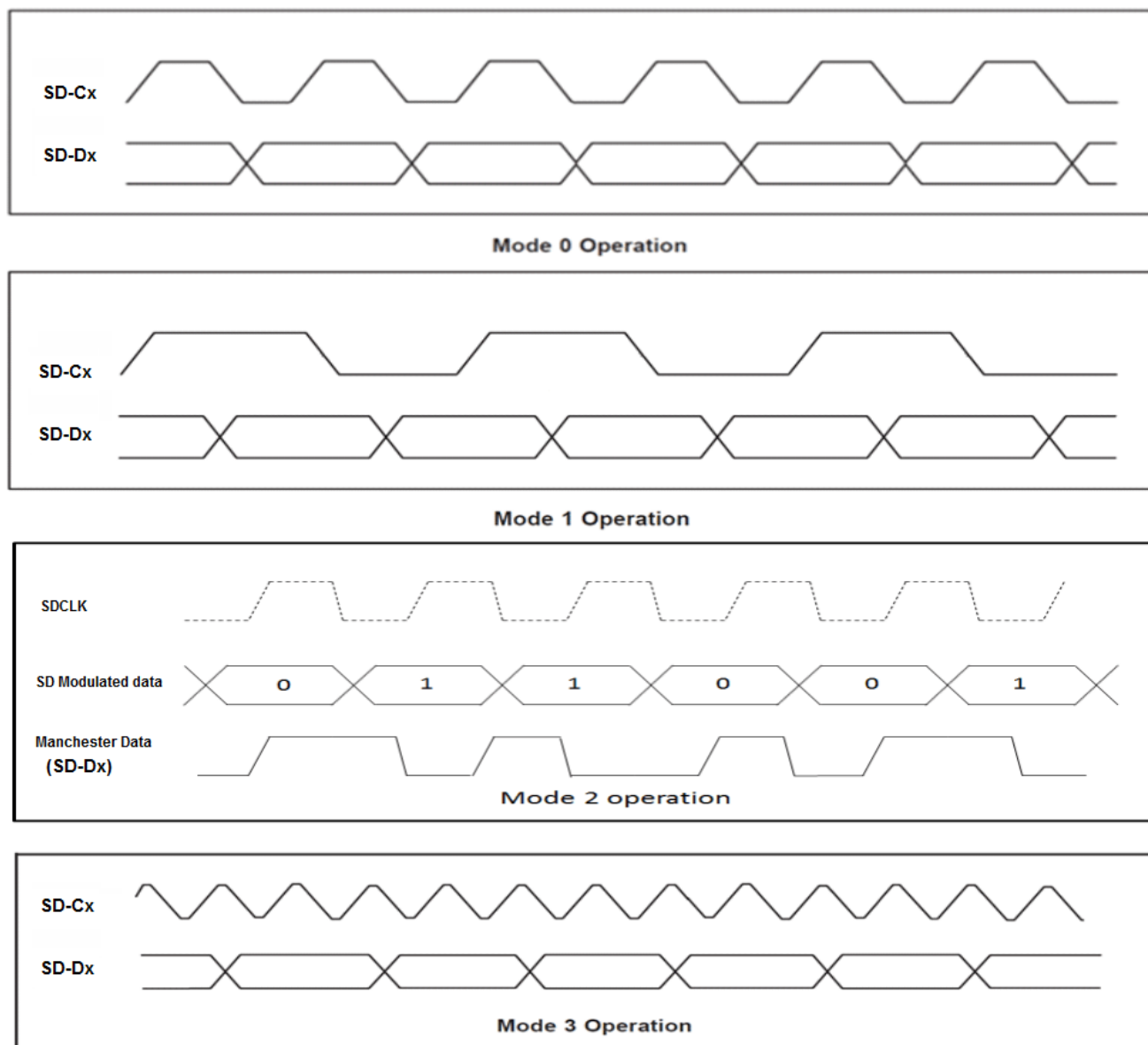
Figure 14-4. Different Modulator Modes Supported
