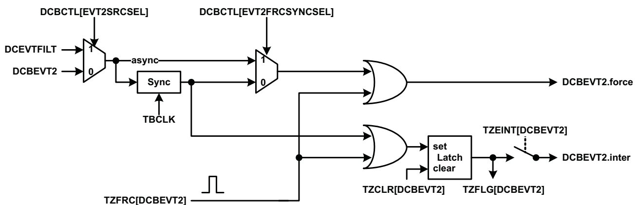
Figure 15-53. DCBEVT2 Event Triggering
