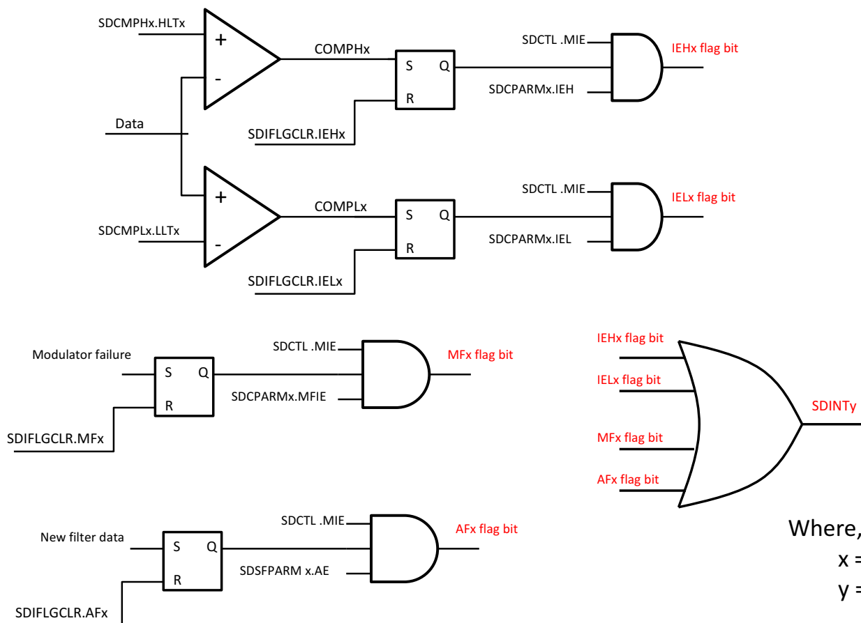
Figure 14-10. SDFM Interrupt Unit
