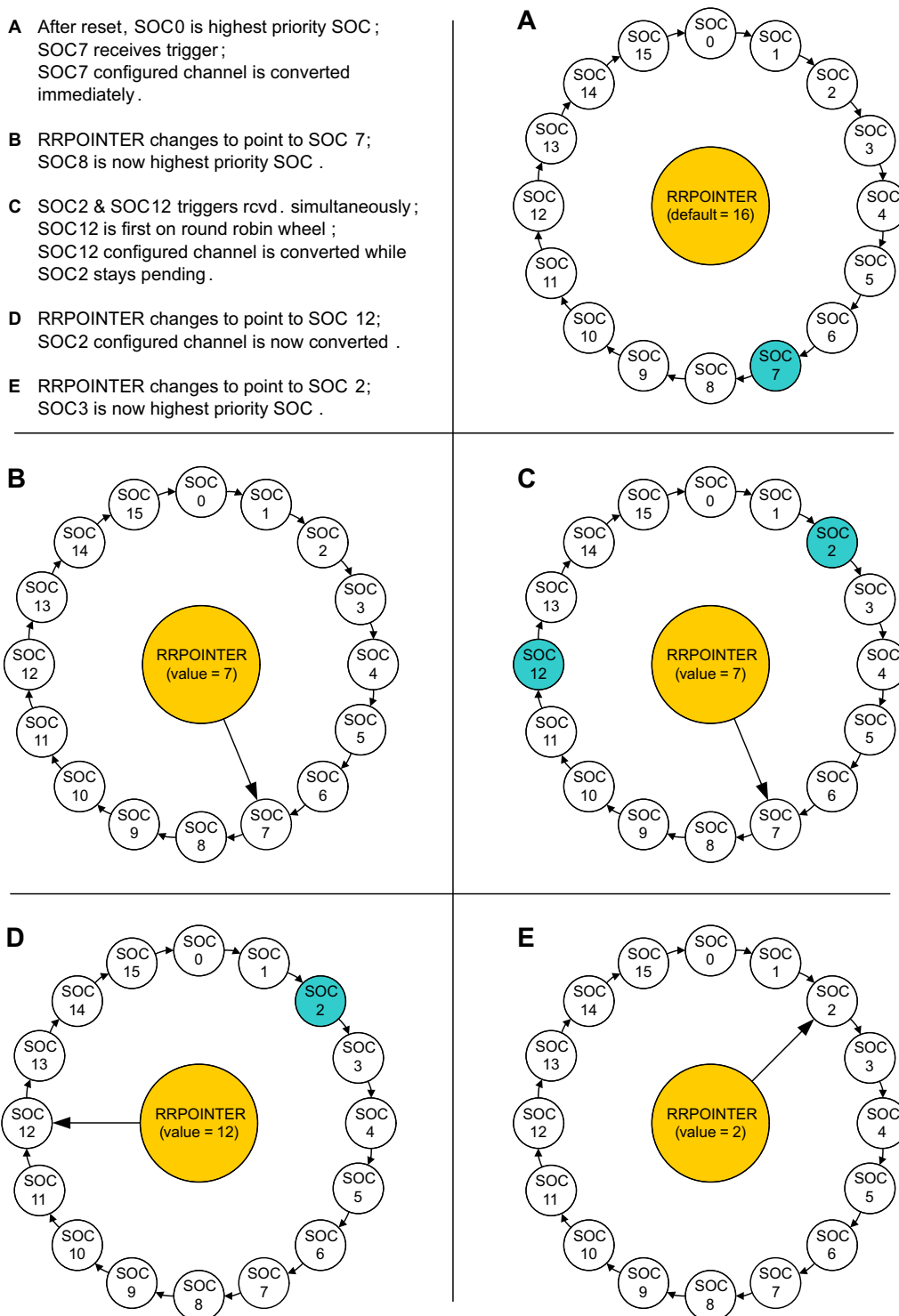
Figure 11-5. Round Robin Priority Example
