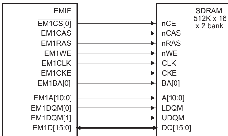
Figure 25-5. EMIF to 512K × 16 × 2 bank SDRAM Interface
