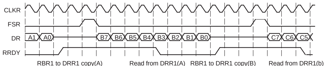
Figure 21-14. McBSP Reception Signal Activity
