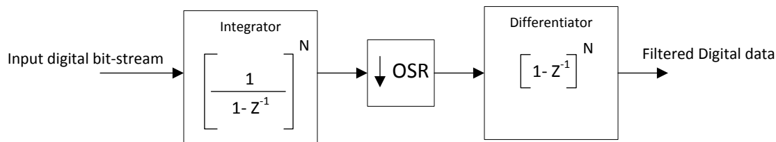
Figure 14-6. Simplified Sinc Filter Architecture
