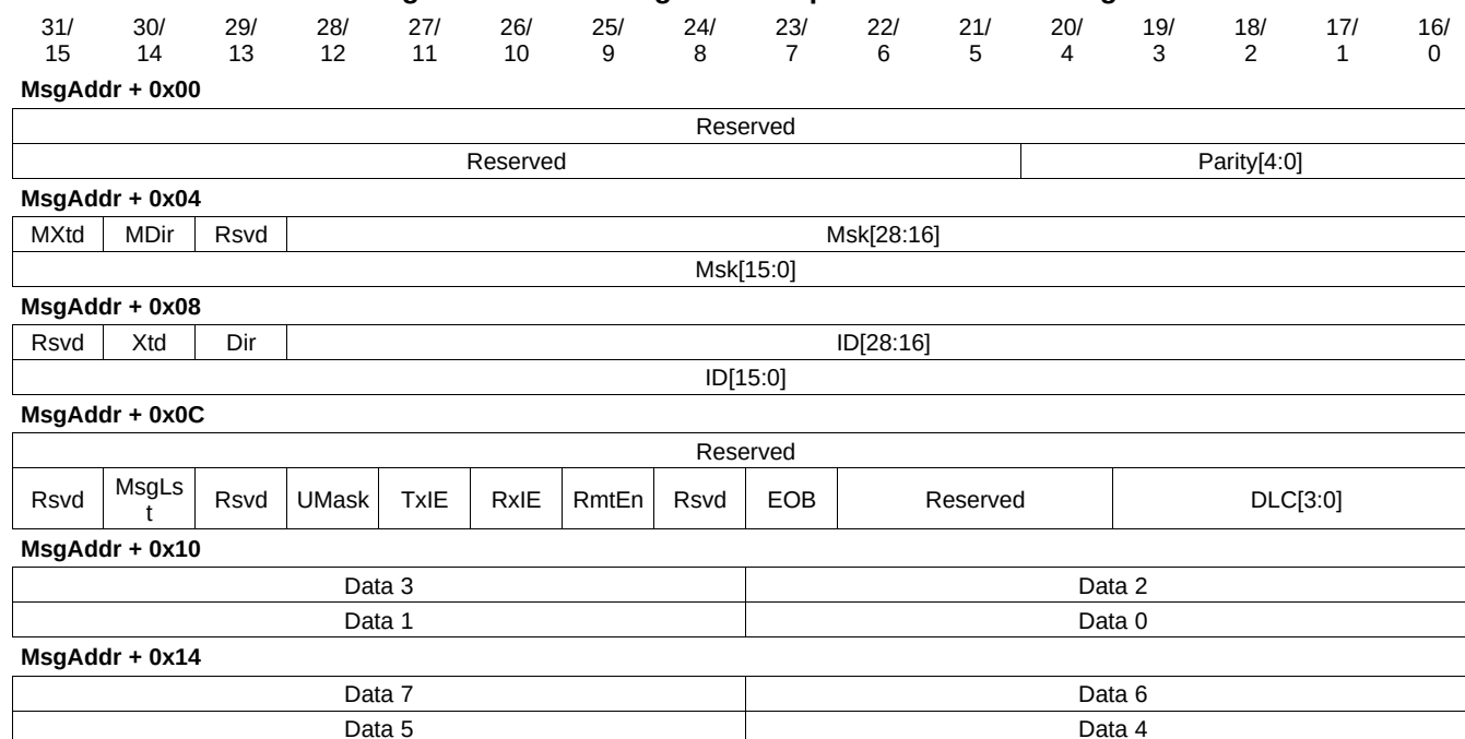
Figure 22-20. Message RAM Representation in Debug Mode
