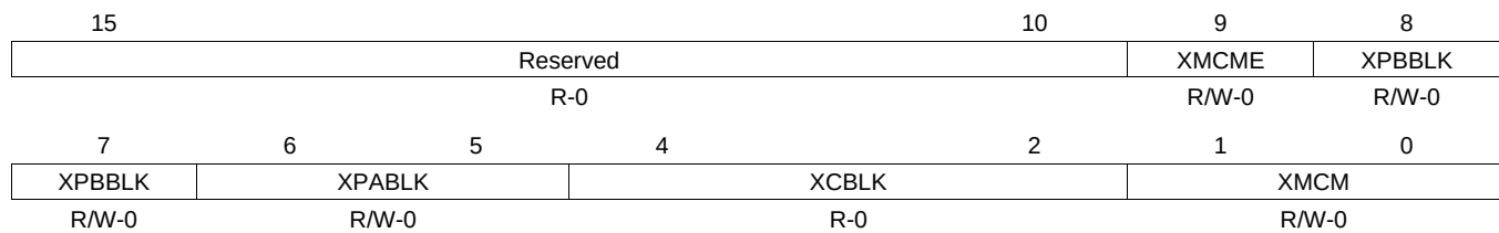
Figure 21-78. Multichannel Control 2 Register (MCR2)
