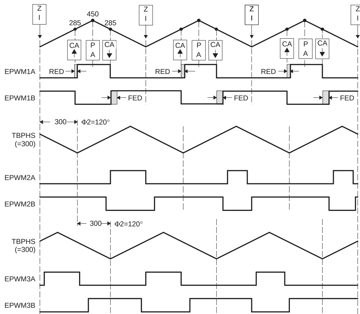
Figure 15-71. 3-Phase Interleaved DC/DC Converter Waveforms for Figure 15-70
