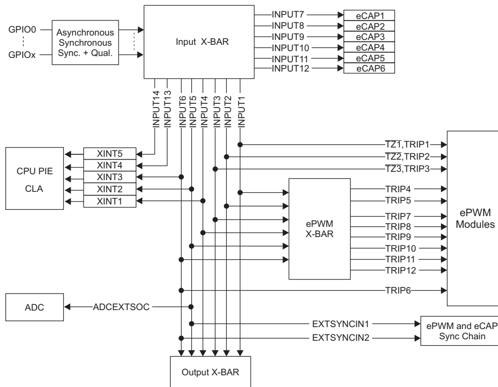
Figure 9-1. Input X-BAR
