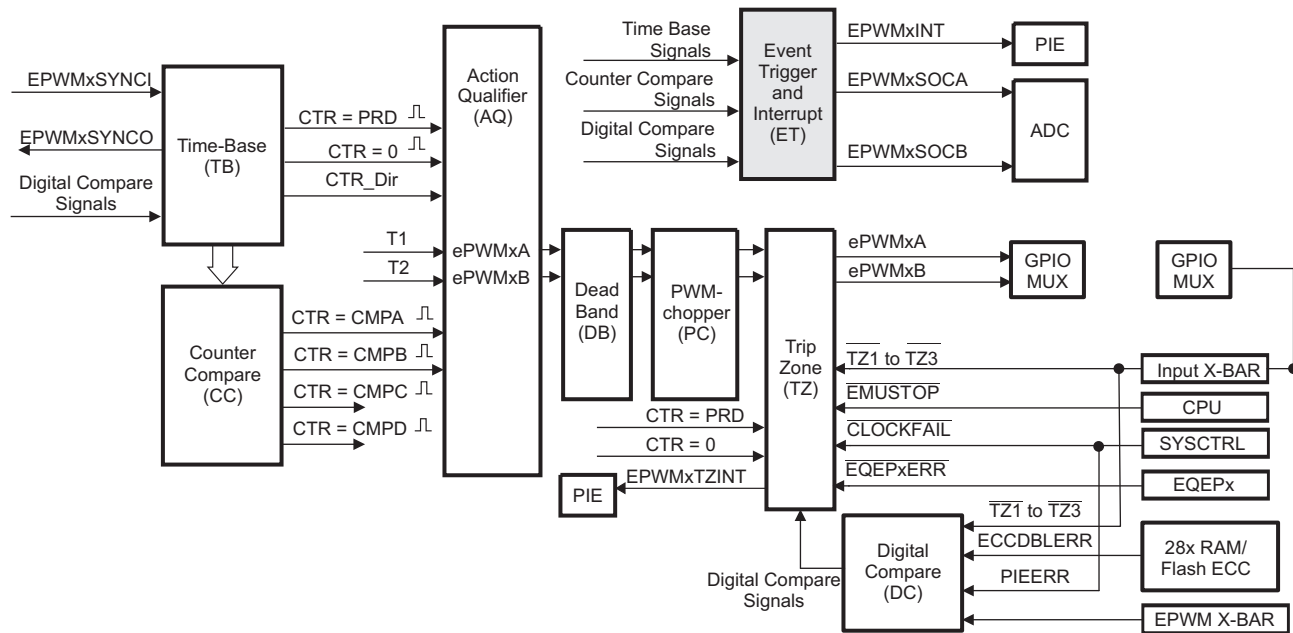
Figure 15-43. Event-Trigger Submodule
