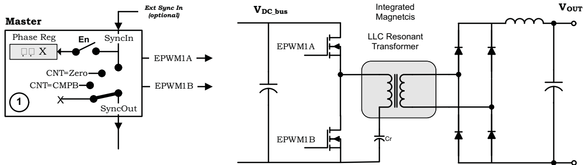
Figure 15-76. Control of Two Resonant Converter Stages
