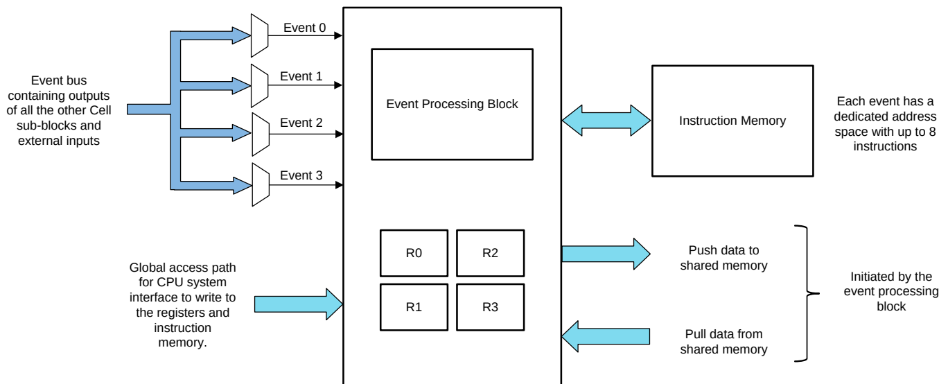
Figure 26-13. High Level Controller Block
