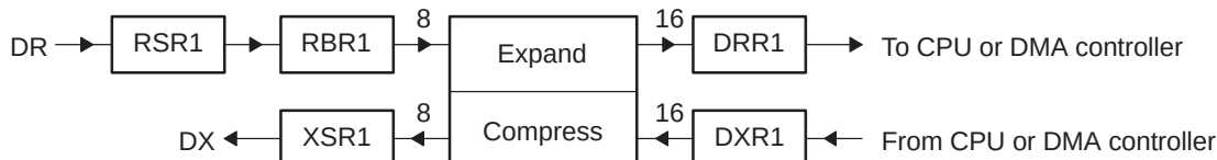
Figure 21-53. Companding Processes for Reception and for Transmission
