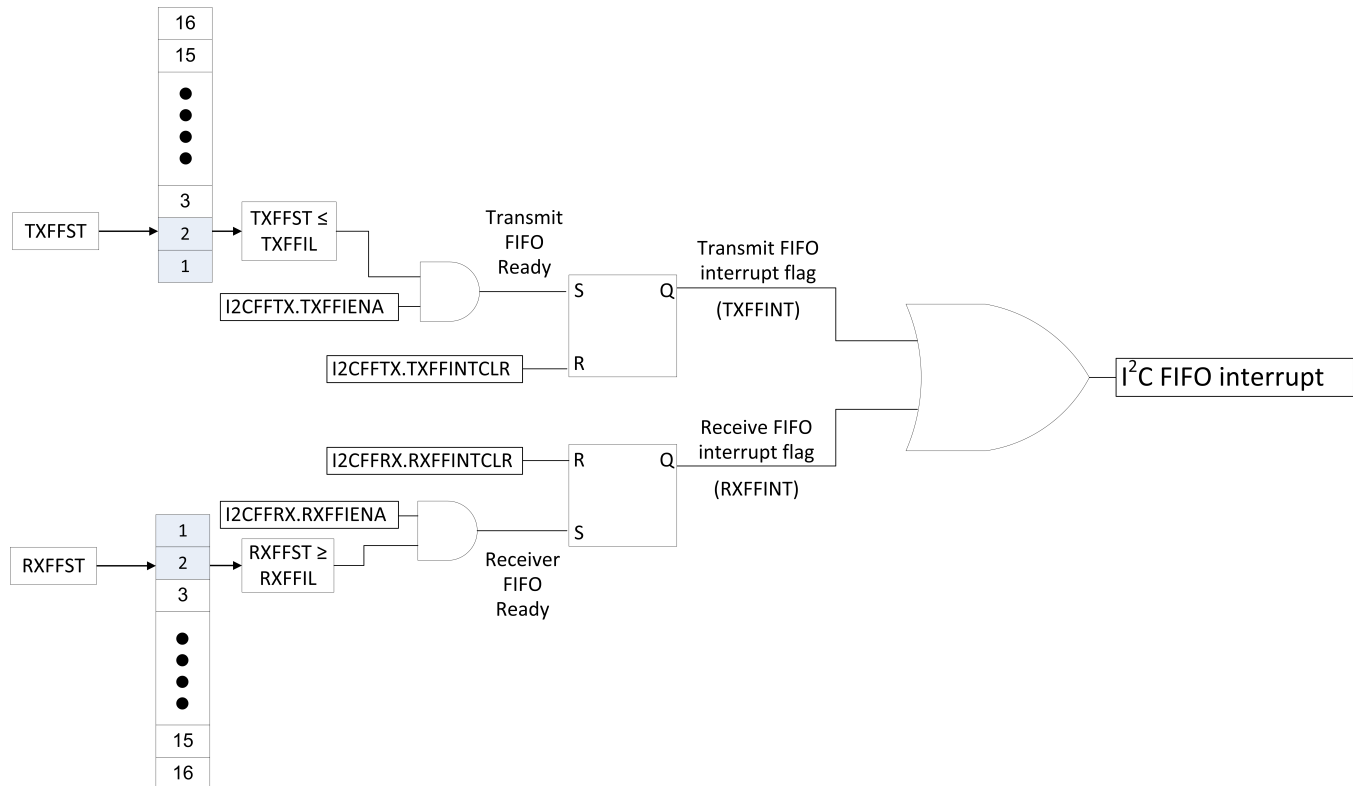
Figure 20-17. I2C_FIFO_interrupt
