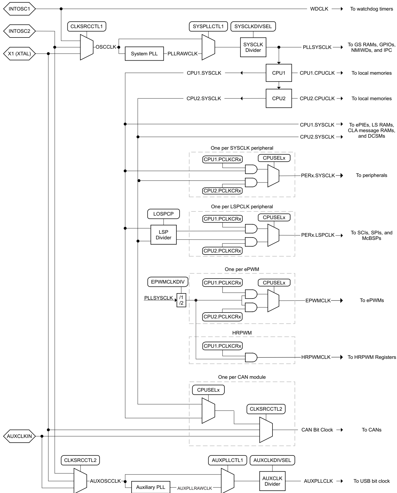
Figure 5-7. Clocking System
