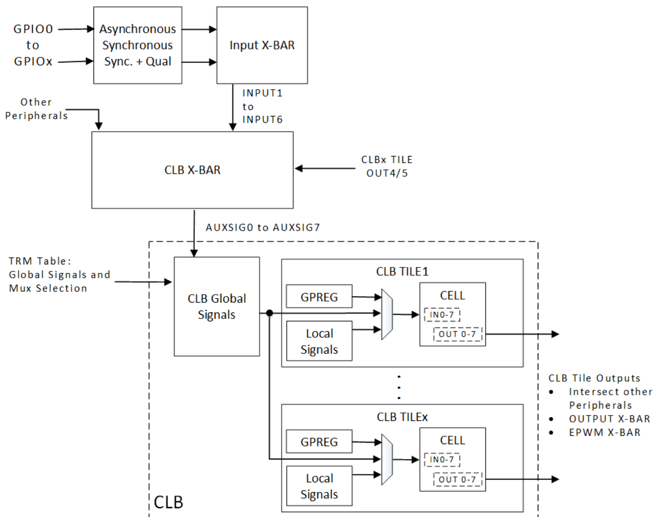
Figure 6-6. CLB Overview
